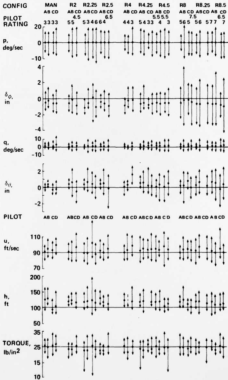
Figure 19.- Maximum, minimum, and average value summary.
