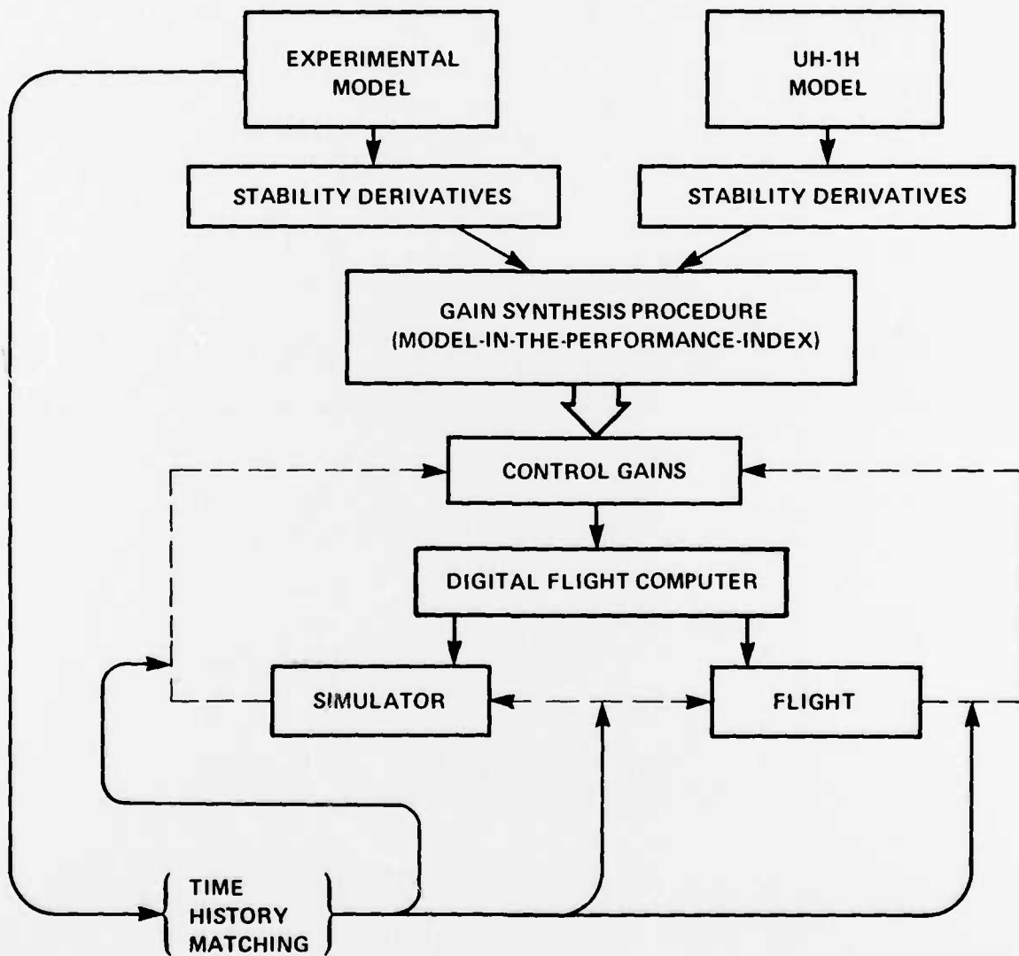
Figure 21.- Configuration verification cycle.
