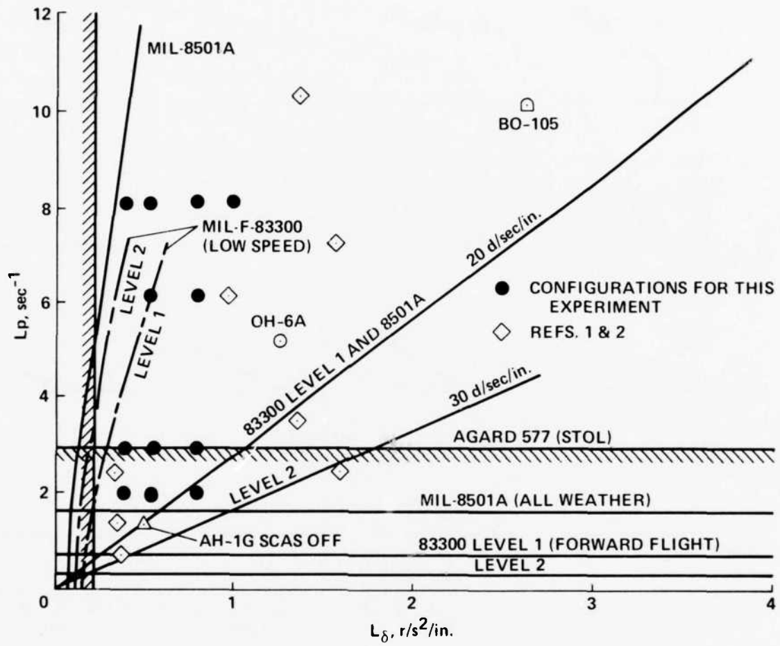
Figure 1.- Current flying qualities boundaries for roll control.
