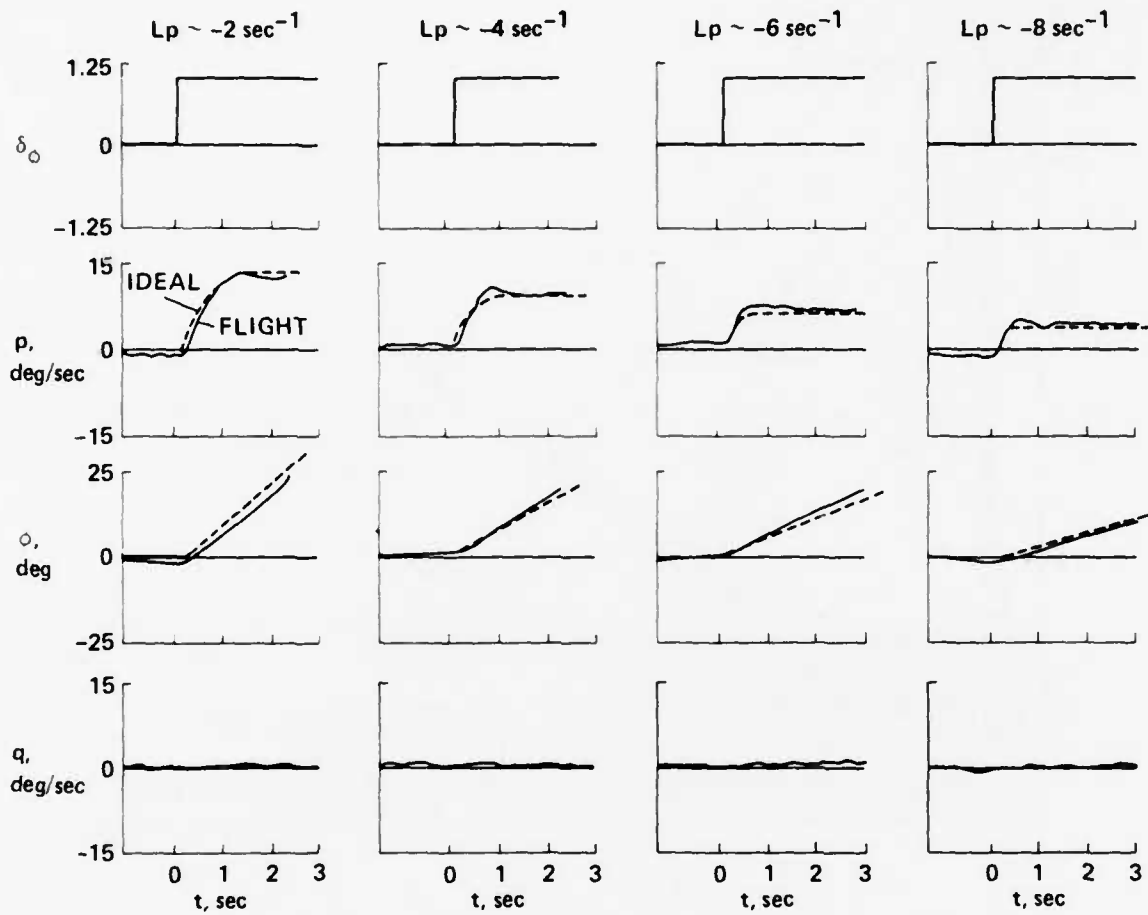
Figure 2.- Configuration verification responses-roll axis (60 knot flight data).
