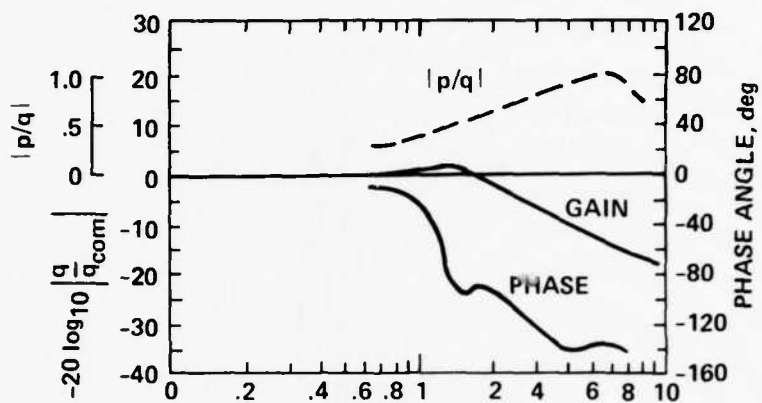
Figure 12.- UH-1H pitch frequency response, 60 knots.
