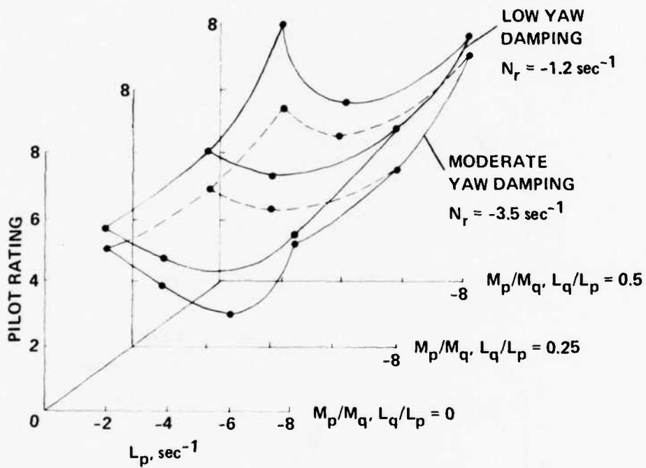
Figure 11.- Composite of roll damping and cross-coupling data.
