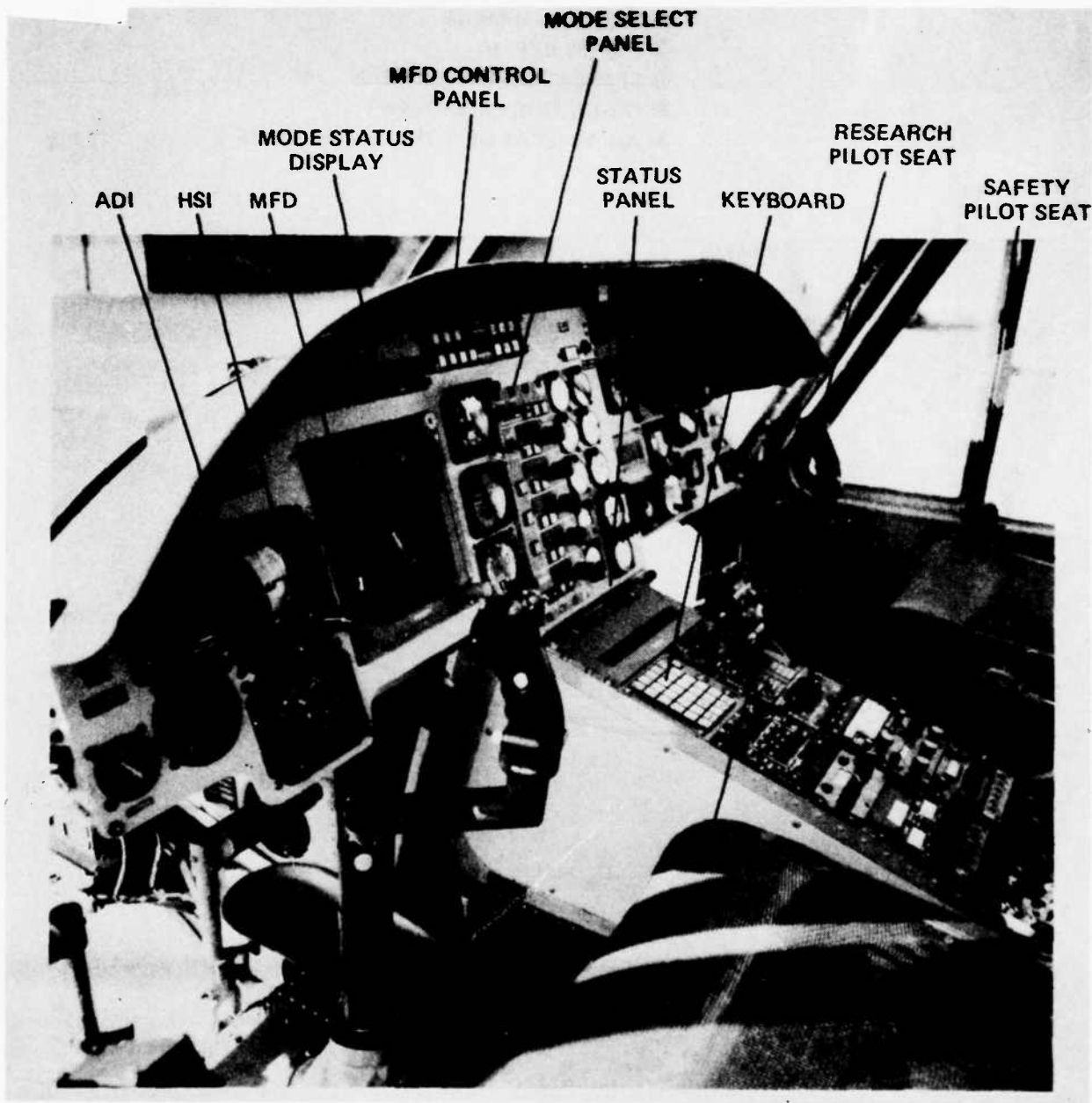
Figure 7.- Cockpit layout from research pilot's side.
