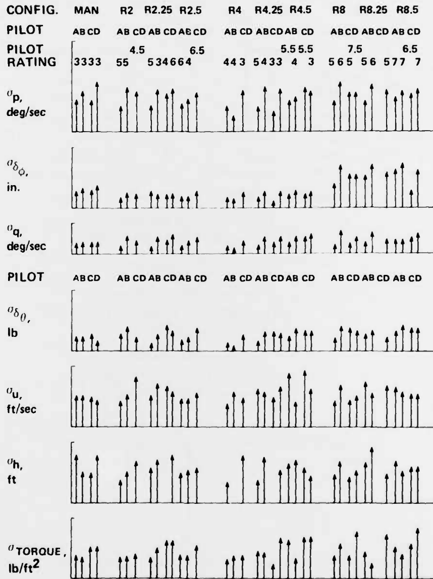
Figure 20.- Standard deviation summary.
