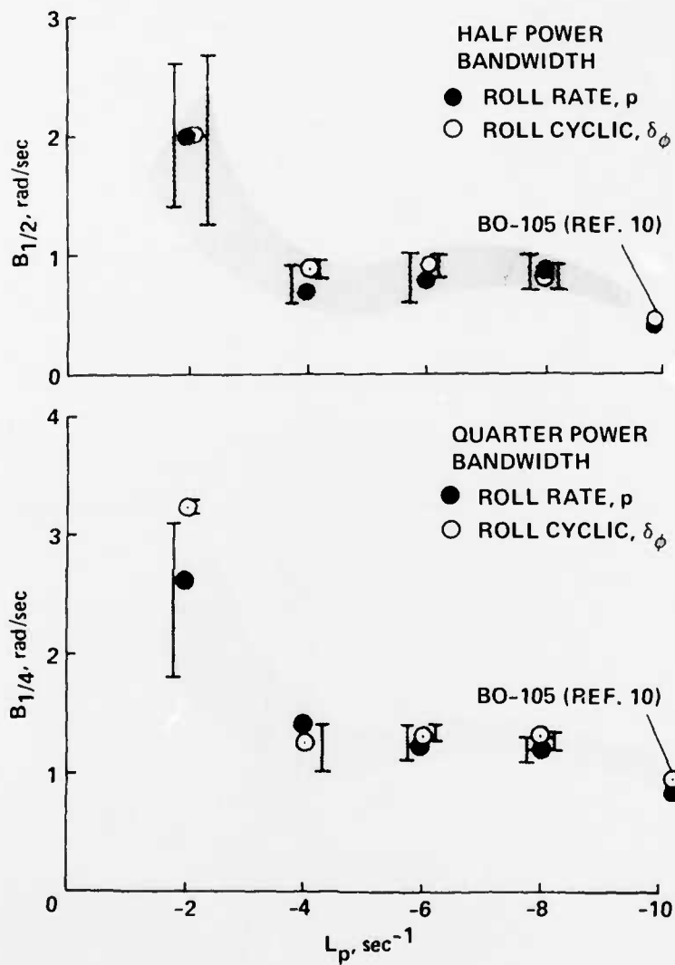
Figure 17.- Roll spectral density, bandwidths.
