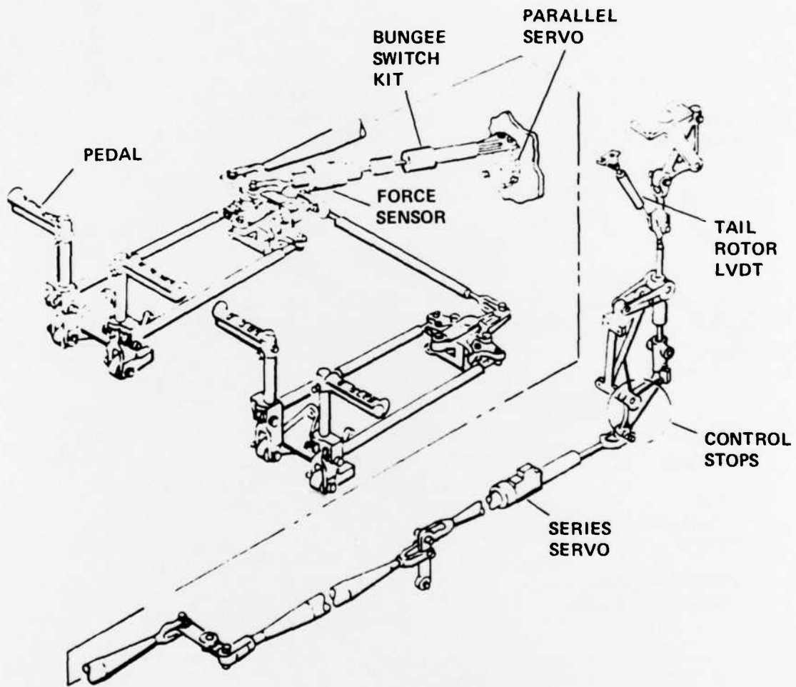
Figure 23.- UH-1H VSTOLAND directional controls.
