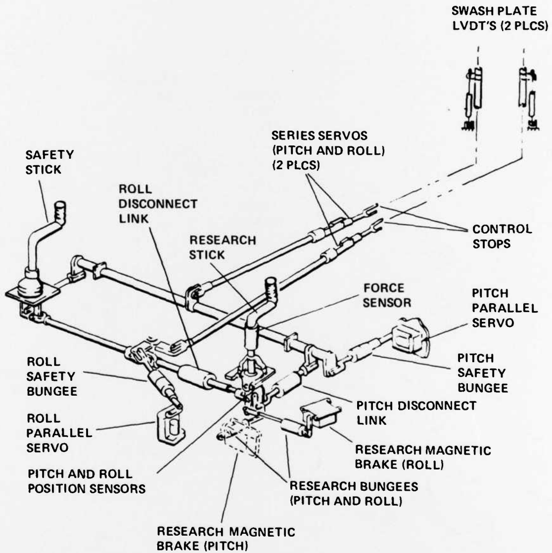
Figure 22.- UH-1H VSTOLAND cyclic controls.
