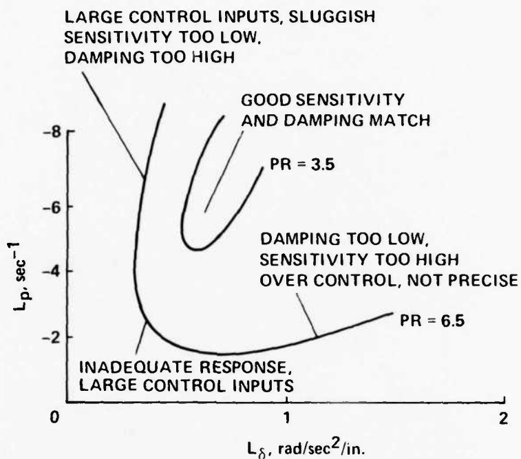
Figure 9.- Summary of pilot comments.
