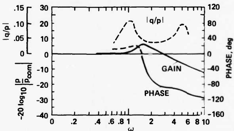
Figure 13.- UH-1H roll frequency response, 60 knots.
