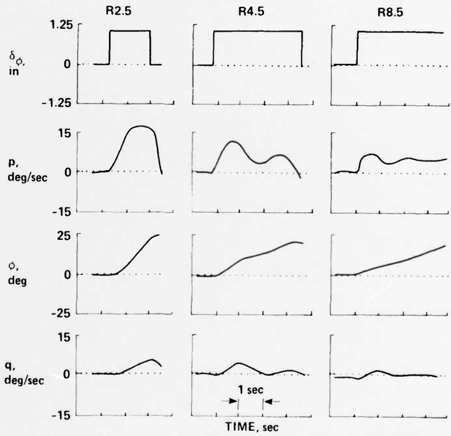
Figure 3.- Coupled responses-roll axis (60 knot flight data).
