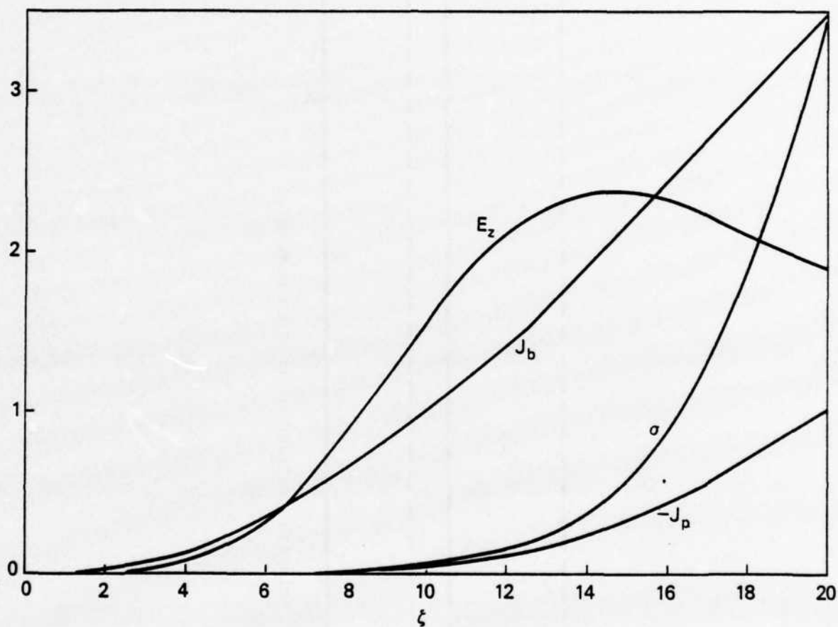
Fig. 2 Typical z -dependences of beam current density J_b on the beam axis, plasma current density J_p , axial electric field E_z and conductivity \sigma on the channel axis near the beam head.
