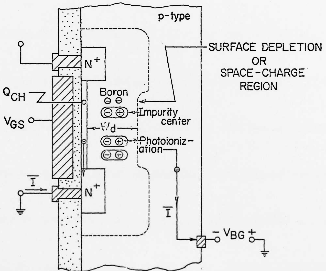
Fig. 1. The Infrared Sensing MOSFET Showing Source and Substrate Current, \bar{I} , due to Emission of Holes from Impurity Centers.
