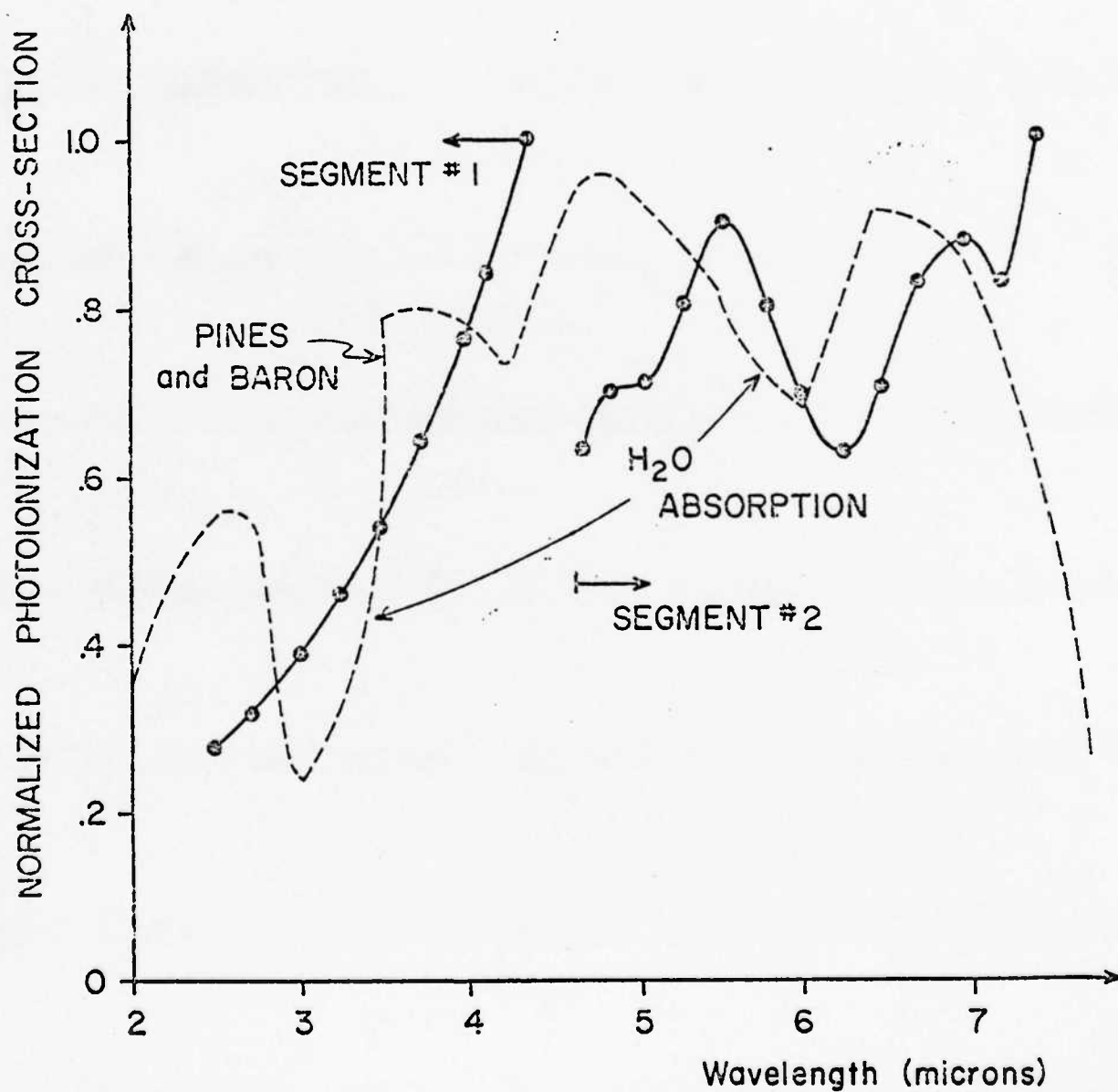
Fig. 8. The experimentally determined photoionization cross section of indium in silicon (solid line) superimposed upon the result of Pines and Baron [16].
