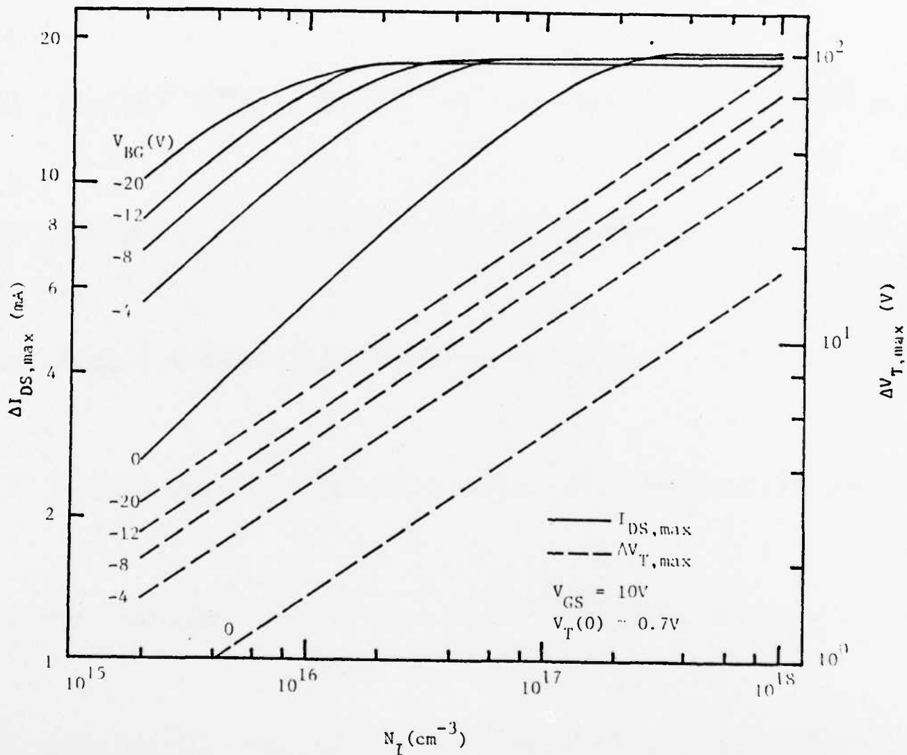
Fig.1. \Delta I_{DS, \max} versus N_I for various backgate bias. V_{GS} = 10V , W/L = 20 , X_0 = 1\text{\AA} , \mu = 600 \text{ cm}^2/V\cdot\text{sec} , A = 0.6V , V_T(0) \approx 0.7V .
