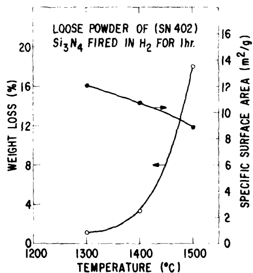
Figure 3. Weight Loss and Specific Surface Area of Loose Powder of SN-402 \text{Si}_3\text{N}_4 Fired in Dry Hydrogen for 1 Hr
