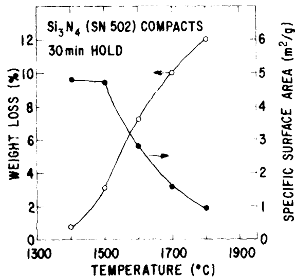
Figure 6. Weight Loss and Specific Surface Area As a Function of Temperature for (SN-502) Si 3 N 4 Compacts Fired for 30 Min in N 2
