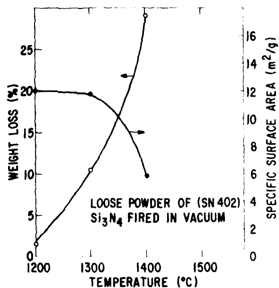
Figure 2. Weight Loss and Specific Surface Areas as a Function of Temperature for Loose Powder of SN-402 \text{Si}_3\text{N}_4 Fired in Vacuum for 1 Hr
