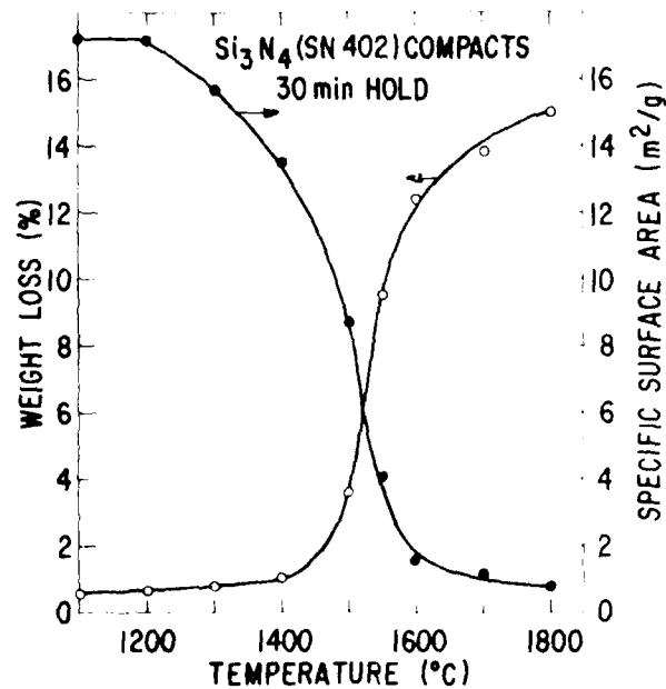
Figure 5. Weight Loss and Specific Surface Area As a Function of Temperature for (SN-402) Si 3 N 4 Compacts Fired for 30 Min in N 2
