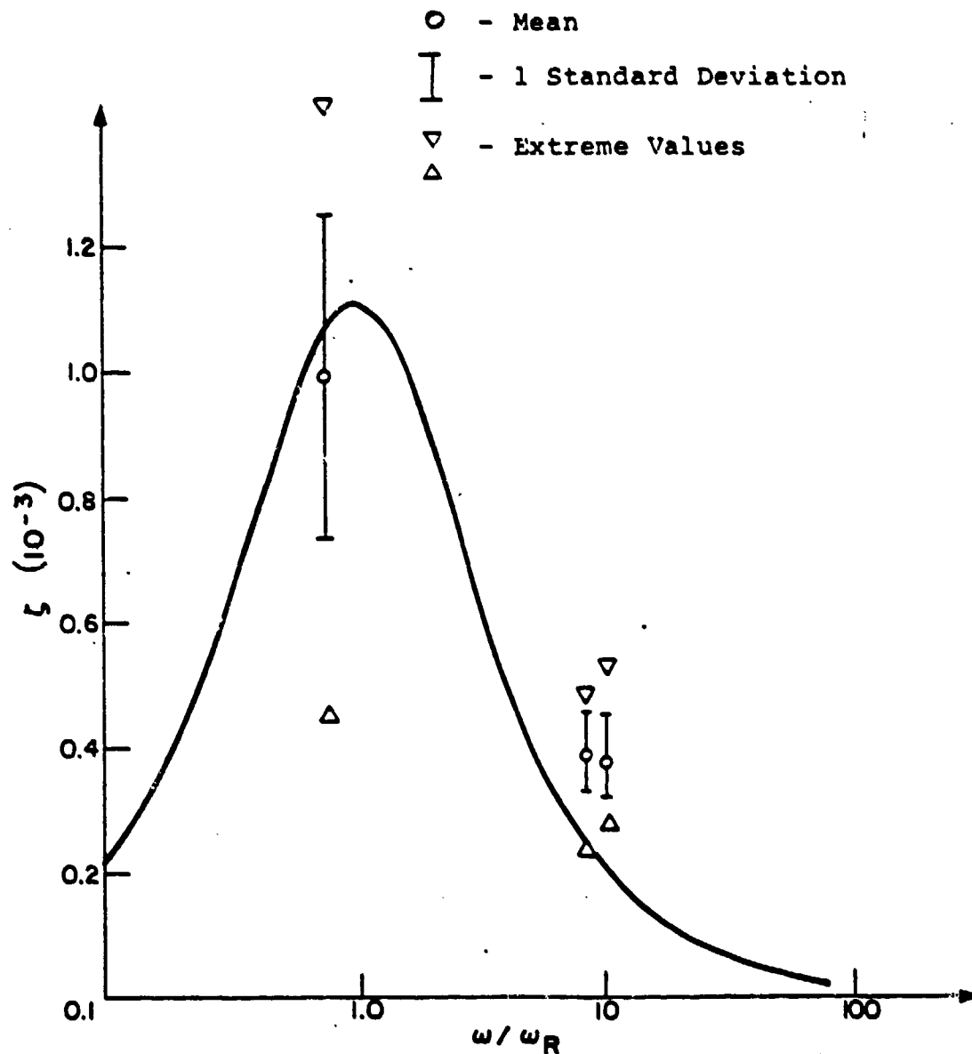
Figure 4.9 Damping of Metal Matrix Specimens vs. Frequency
