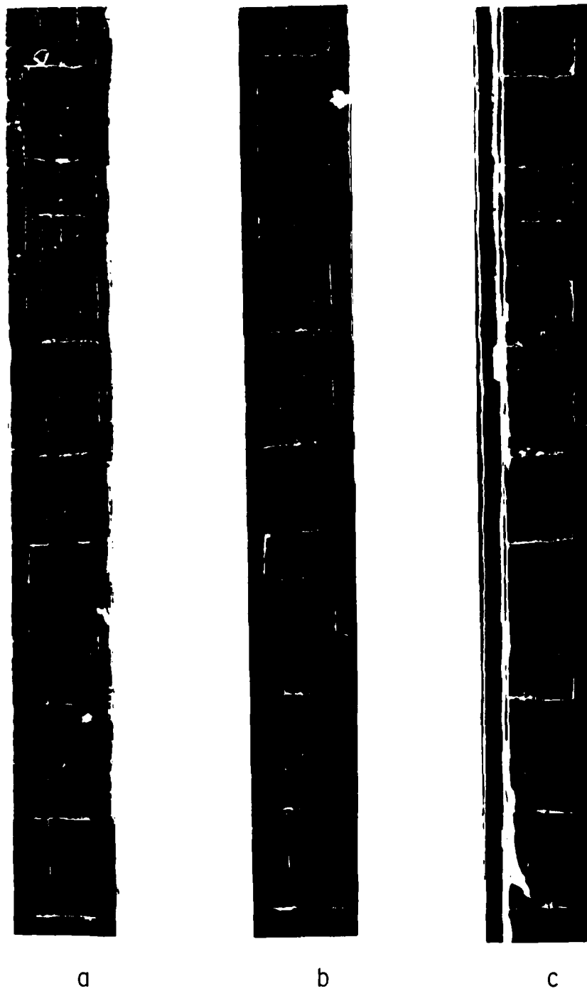
Fig. 1. Edge Replicas of a Progressively Fatigue-Damaged [0,90_2]_s Laminate, \sigma_{\max}/\sigma_{\text{ult}} = 0.70 : a) 1 cycle, Stage I; b) 1400 cycles, 1 percent stiffness change, Stage I; c) 22,000 cycles, 3 percent stiffness change, Stage II.
