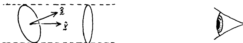
Figure 4. A surface patch viewed from a direction that is not perpendicular to the surface appears foreshortened. The apparent area is its true area times the cosine of the angle between the surface normal and the direction towards the viewer. A surface patch will intercept an amount of light proportional to its apparent area as seen from the light source. In the case of an ideal Lambertian reflector, all of this light is re-emitted. So the brightness is proportional to the cosine of the angle between the surface normal and the direction towards the light source.
