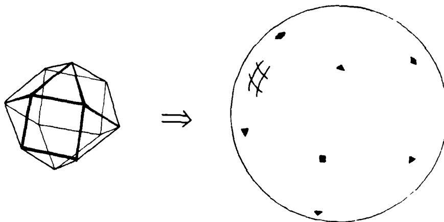
Figure 12. The extended Gaussian image of a polyhedral object is a distribution of point masses on the sphere. The position of the points is determined by the orientation of the faces of the polyhedron, while the masses are equal to the corresponding areas. For clarity only points lying on the visible hemisphere of the Gaussian sphere are shown.
