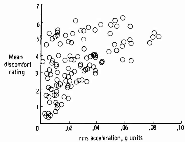
(b) Weighted acceleration; r = 0.535 .
