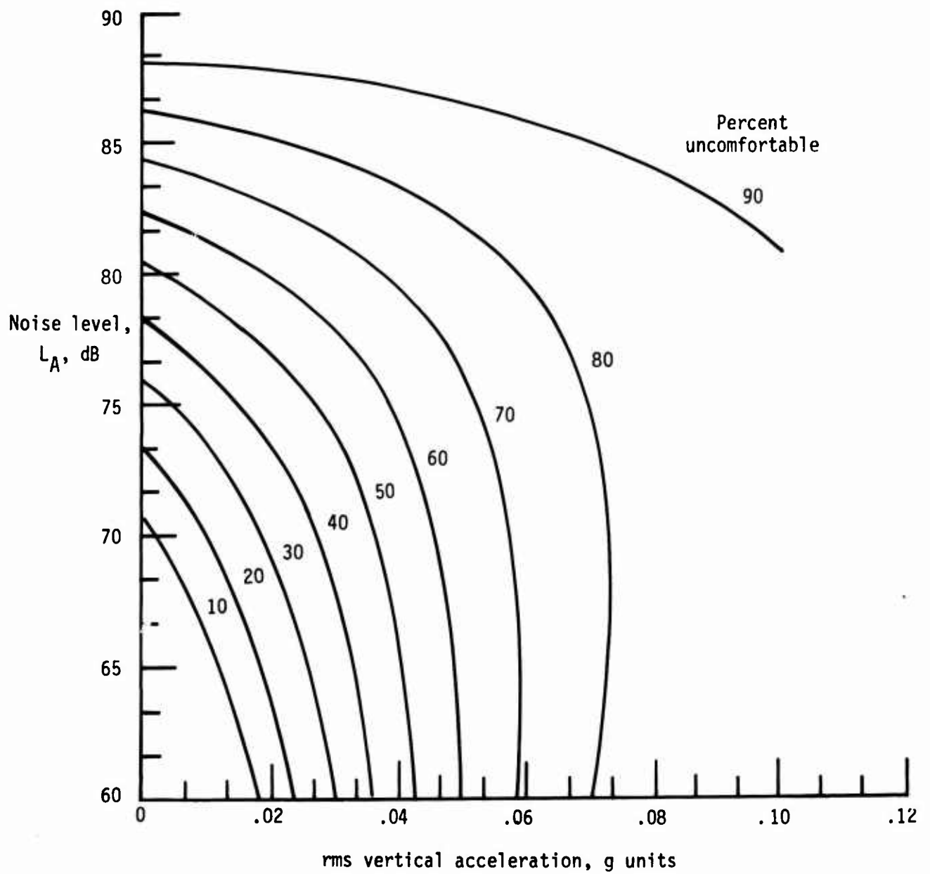
Figure 12.- Values of A-weighted noise level and rms vertical acceleration that produce constant values of discomfort.
