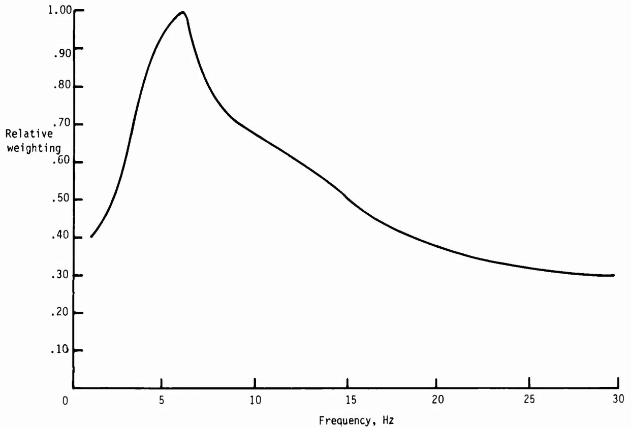
Figure C1.- Relative frequency weighting for vertical-axis vibration.
