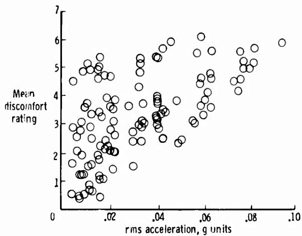
(a) Unweighted acceleration; r = 0.551 .
