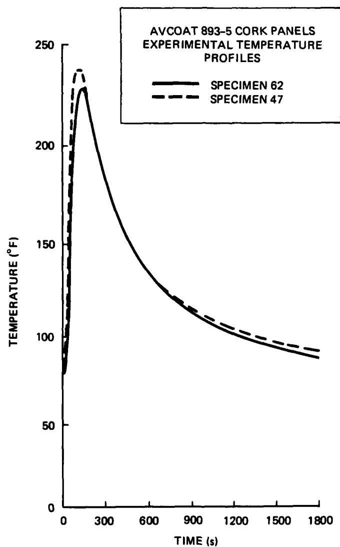
Figure C-12. Avcoat 893-5 cork sheet.
