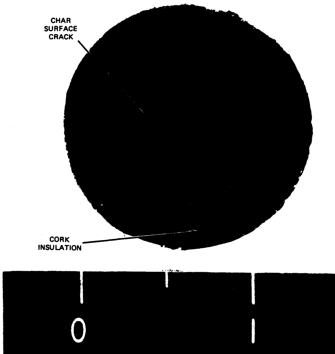
Figure G-3. Flexfram 605 ( 9.91 \text{ Btu/ft}^2\text{-s} heat flux).
