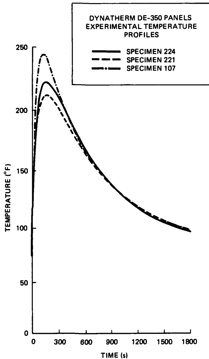
Figure C-7. Dynatherm DE-350.
