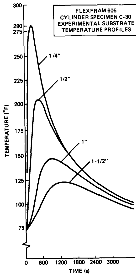
Figure D-5. Flexfram 605, specimen C-30.
