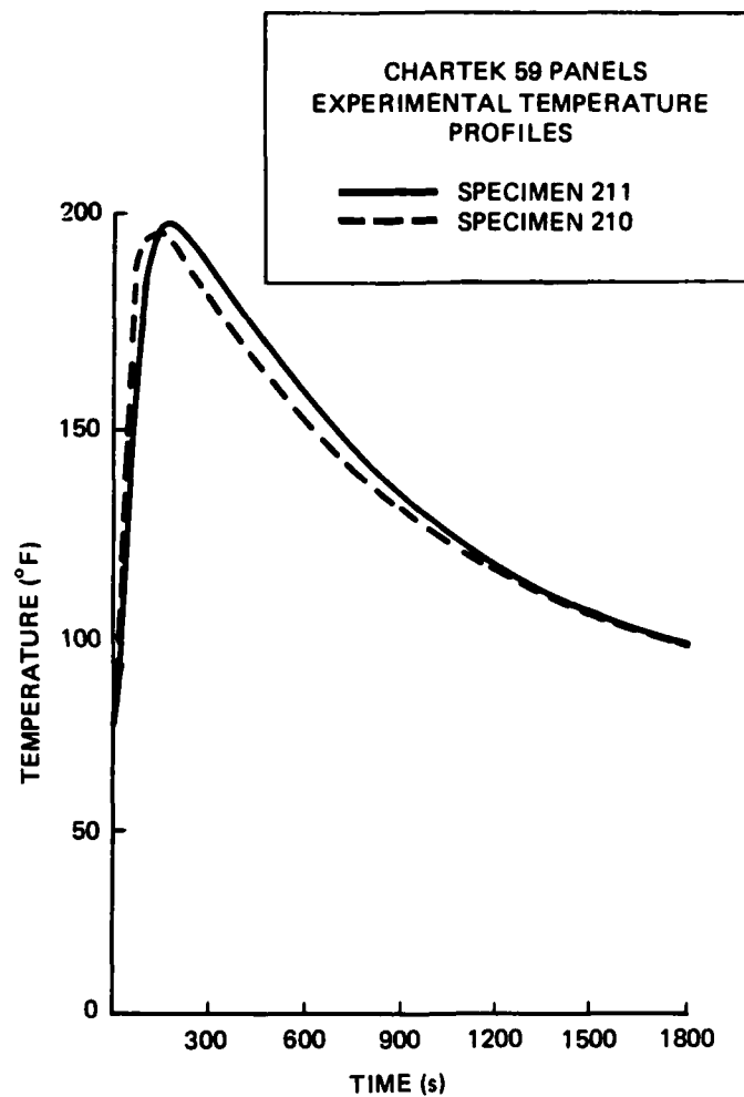
Figure C-4. Chartek 59.
