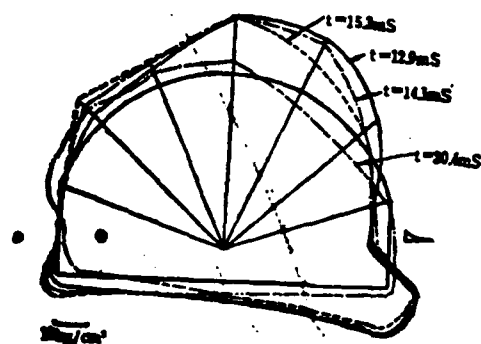
Fig. 10. Variations of radial stress with time.
