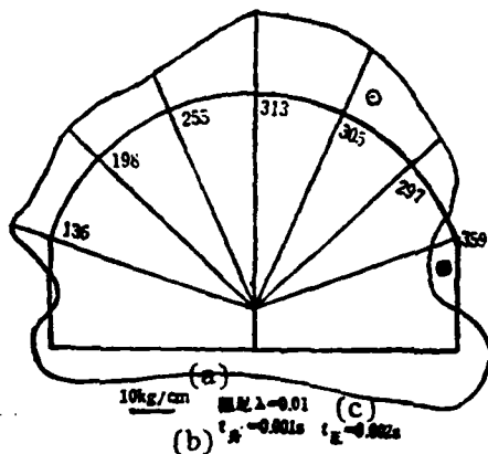
Fig. 4. Radial stress surrounding the cave. Key: (a) Damping; (b) Ascending; (c) Positive.
