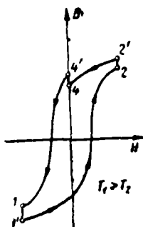
Fig. 3-4. Anomalous manifestations of magnetic viscosity with T_1 > T_2 and H=0 .
