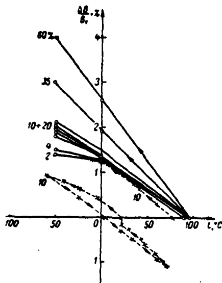
Fig. 6-1. Dependence of magnetic induction on the temperature in magnetic system with the inner frame magnet from the alloy ДИДК25БА with different degree of demagnetization.
