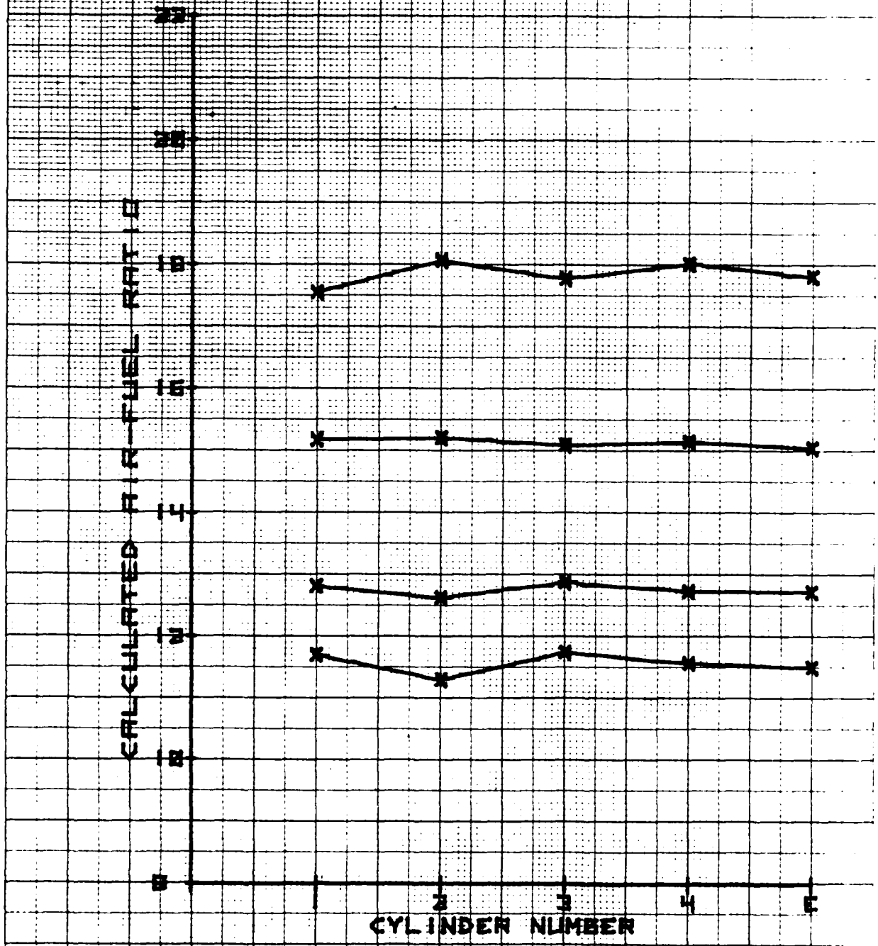
Figure A-16. Air-Fuel Variation, Turbulent Flow Manifold, Leanout, Approach
