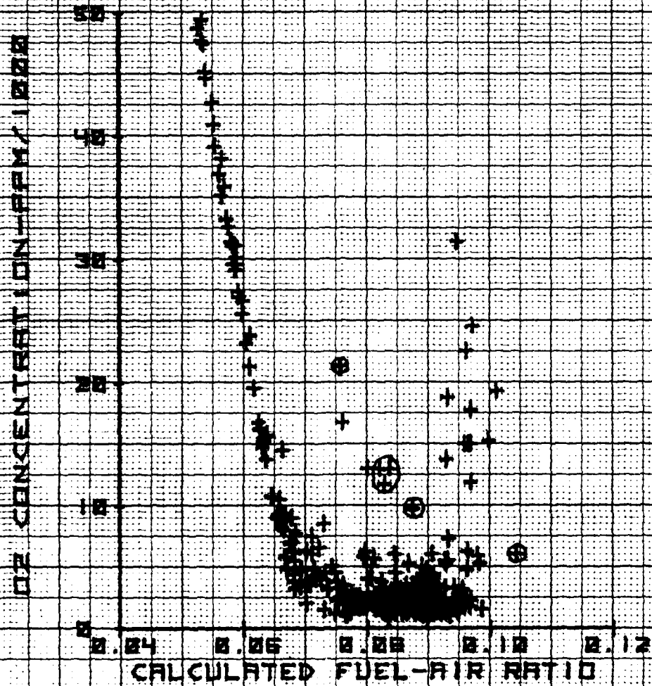
Figure A-30. Exhaust Oxygen Versus Calculated Fuel-Air Ratio
