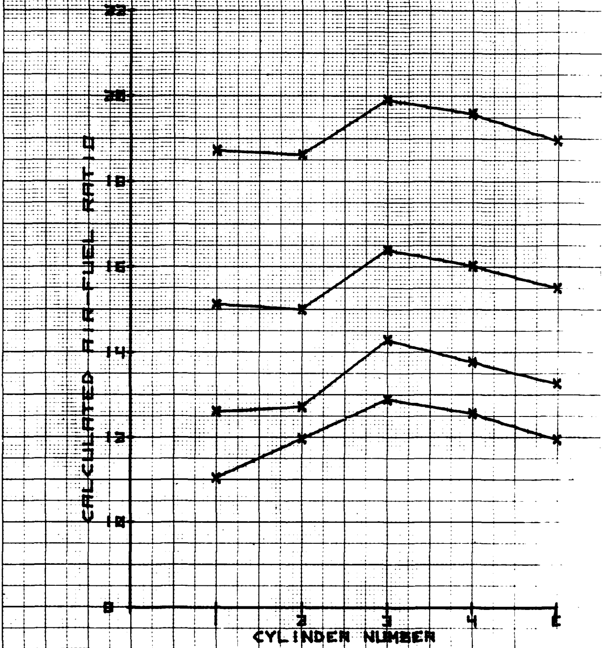
Figure A-15. Air-Fuel Variation, Turbulent Flow Manifold, Leanout, Climb
