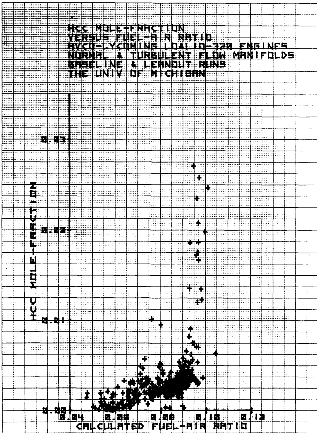
Figure A-28. Exhaust Hydrocarbons Versus Calculated Fuel-Air Ratio
