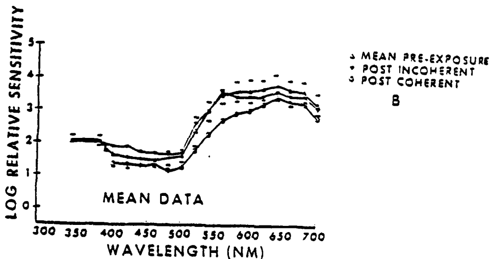
Figure 7. ERG recorded from Pseudemys . In the upper graph (A) mean preexposure spectral sensitivity is compared to the animal's spectral sensitivity during exposure to either 620 nm coherent or incoherent light. In the lower graph (B) the animal's postexposure spectral sensitivity is compared to its preexposure level for the two different exposure conditions.
