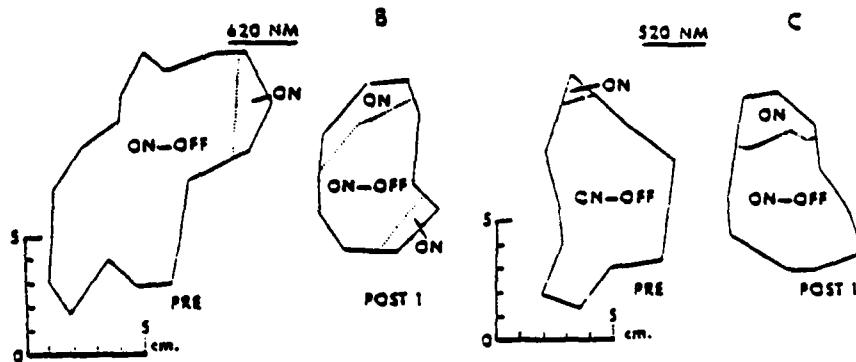
Figure 2. This cell was exposed for one hour over its entire receptive field at 10^{11} quanta/sec/cm 2 . Post-exposure spectral sensitivities for both the on (upper portion) and off (lower portion) components decreased significantly within the first two hours postexposure and were no longer measurable after two hours. Receptive fields constricted and by the end of two hours were no longer measurable.
