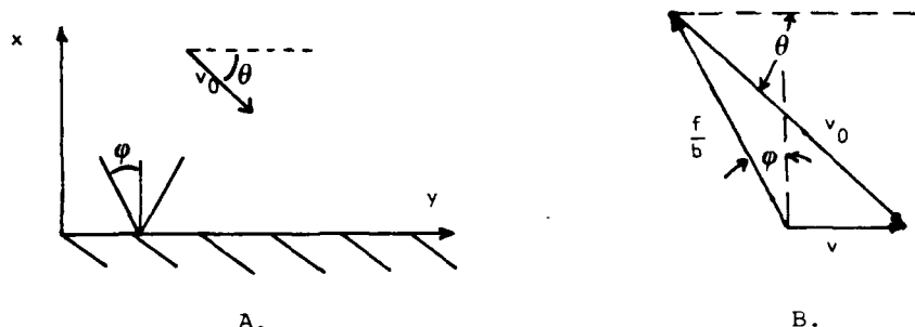
Figure 19. Geometry for generalized damper analysis
