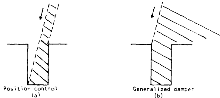
Figure 9. Friction cone
