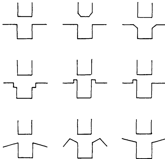
Figure 2. Variations of peg-in-hole require different strategies
