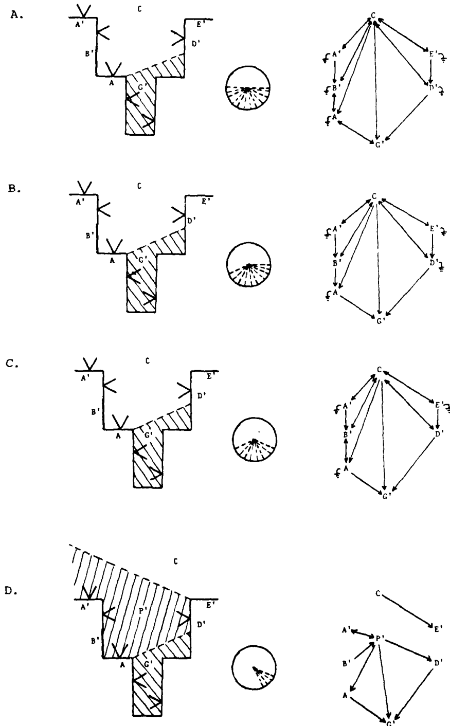
Figure 11. Multi-move peg-in-hole strategy synthesis
