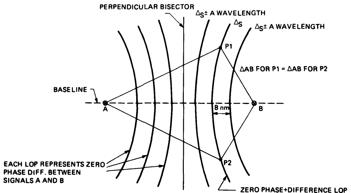
Figure 10. Hyperbolic Configuration
