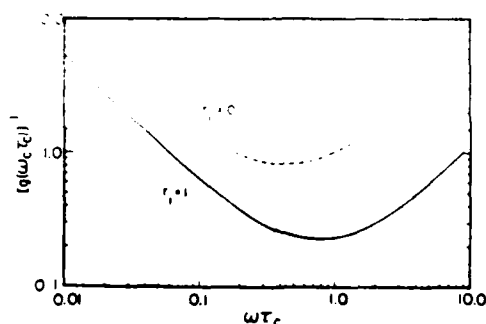
FIG. 2. Dimensionless function [g(\omega\tau_c)]^{-1} vs \omega\tau_c for r_c = 0 and 1 with r_0 = 1 .
