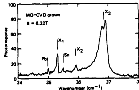
Fig. 6 Photothermal ionization spectrum for Dapkus' et al MO-CVD sample.
