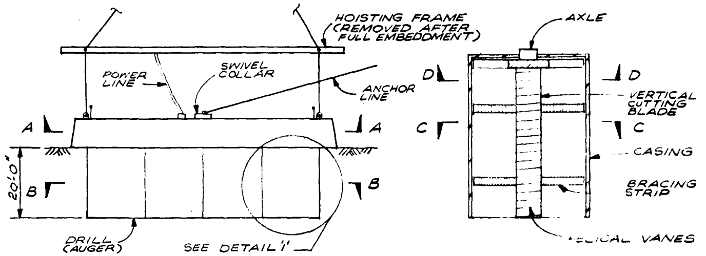
DRILLED-IN-ANCHOR ELEVATION 1" = 20'
