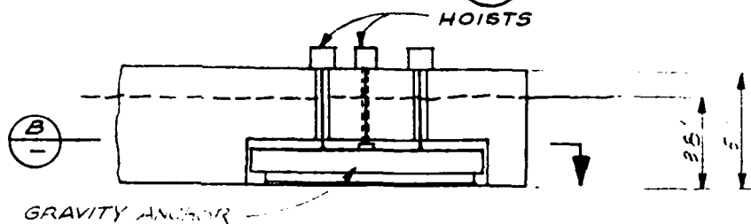
DETAIL ② 1" = 60'
