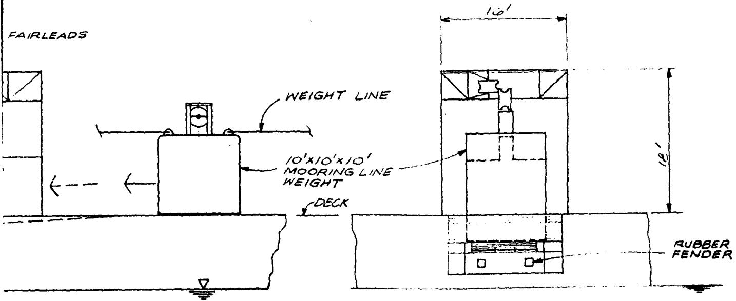
BOW ELEVATION 1" = 10'
