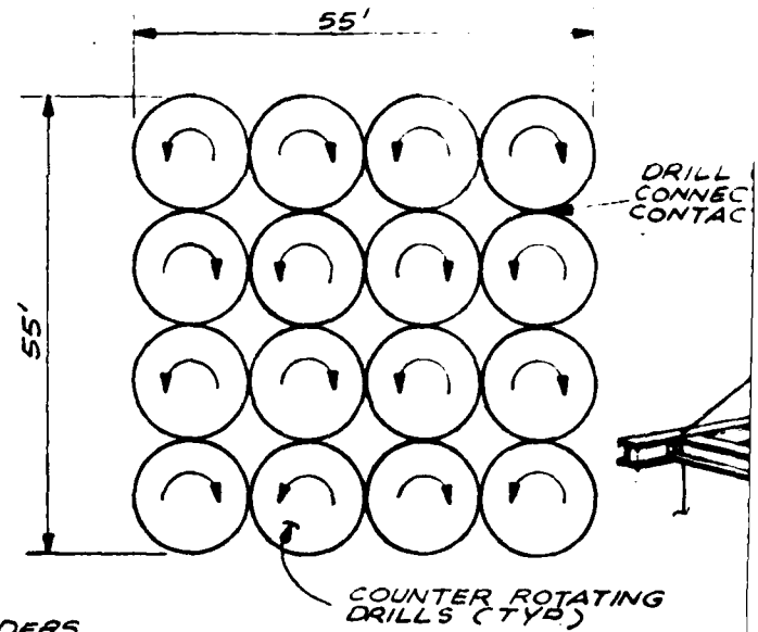
DETAIL 'I' 1" = 10'
