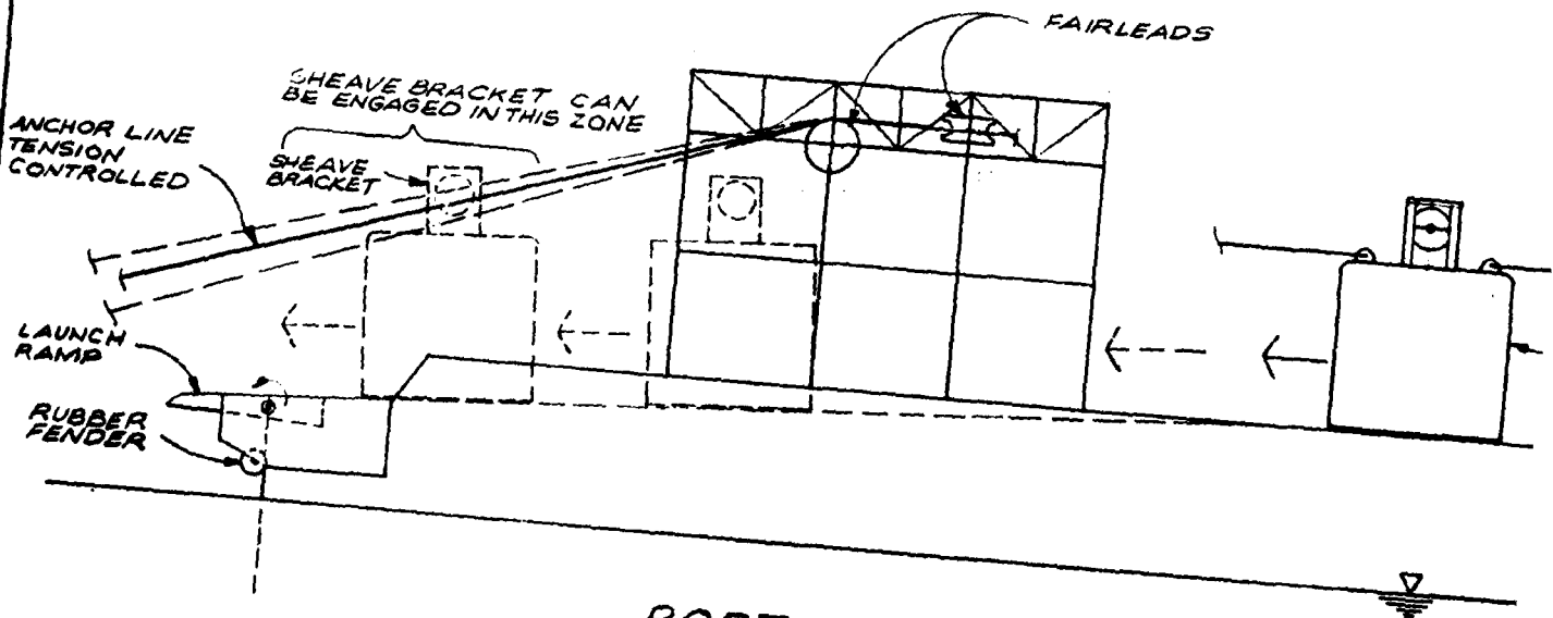
PORT ELEVATION 1" = 10'
