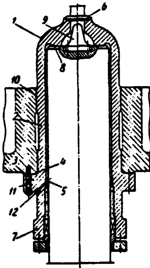
Fig. 126. Schematic of hydraulic cylinder.
