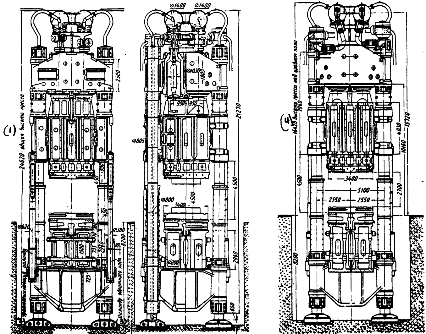
Fig. 43. Eight-cylinder hydraulic press by effort/force 30000 t. Sections/cuts along the transverse axes (see Fig. 42).
