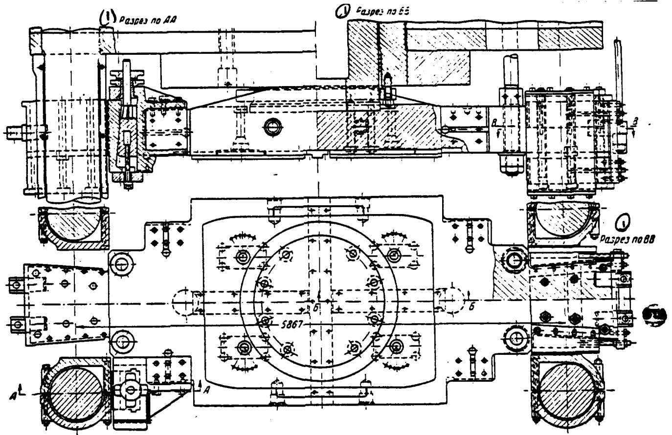
Fig. 19. The crosshead of forging press by effort/force 7000 t.
