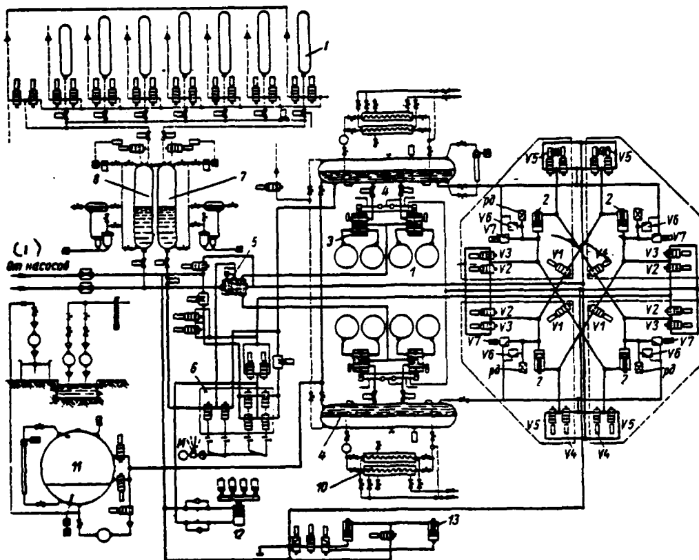
Fig. 354. The hydraulic schematic of stamping machine by effort/force 31500 t: 1 - master cylinders; 2 - recurrent and compensating cylinders; 3 - filler valves; 4 - filler tank; 5 - main bleeder; 6 - control valves; 7 - water bottles of pull-backs; 8 - water bottles of master cylinders; 9 - compressed air tanks; 10 - water cooler; 11 - receiver tank; 12 - servocontrol by filler valves; 13 - knockouts; V1 - valves for double-t joint of pull-backs; V2 - pressure valves of pull-backs; V3 - support valves; V4 - drain valves (from the upper
