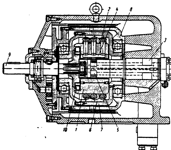
Fig. 266. The construction/design of a rotational-plunger pump with the freely moving plungers: 1 - rotor; 2 - plunger; 3 - distributive axis/axle; 4 - valve ports; 5 - plenum channels; 6 - conical carrier rings; 7 - rotating drum; 8 - unit of pump; 9 - drive shaft; 10 -
