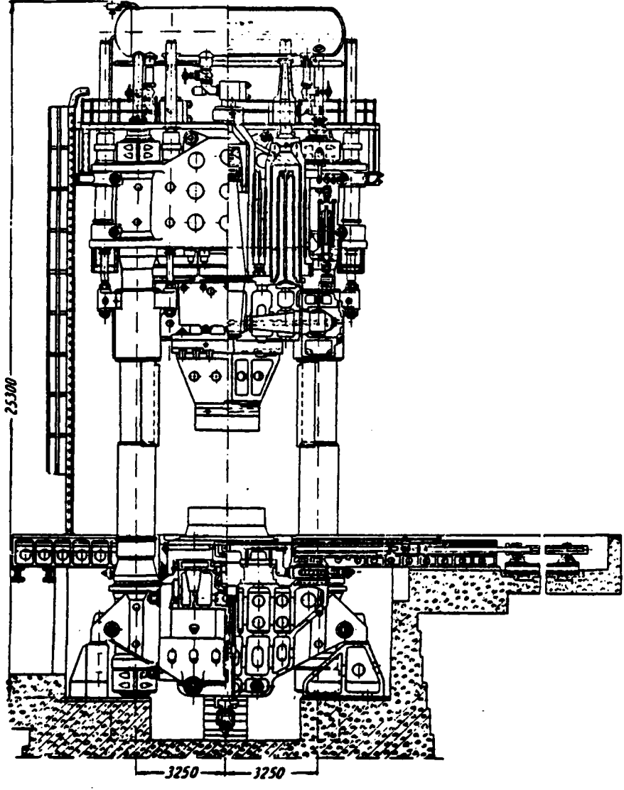
Fig. 17. Hydraulic forging press by effort/force 15000 t.
