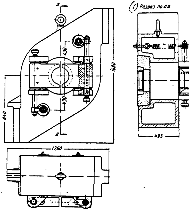
Fig. 100. Stripper, used in the broaching presses.
