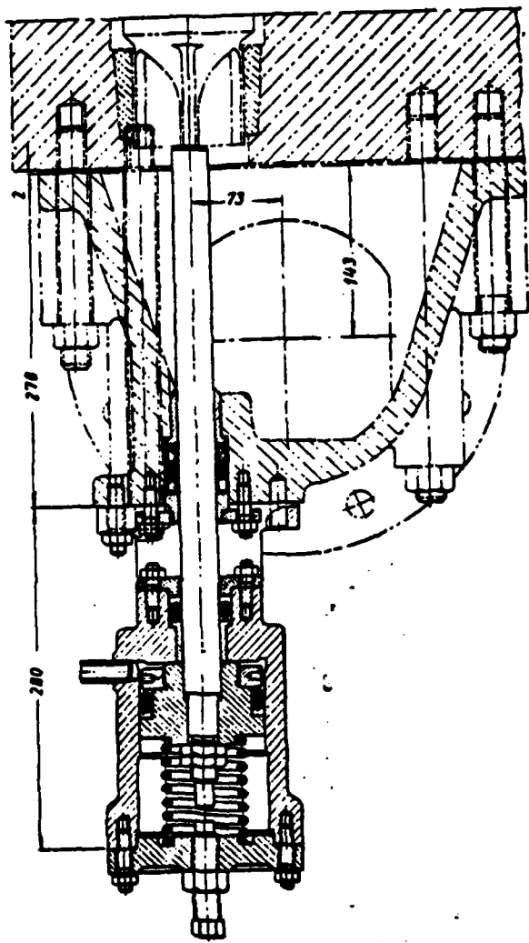
Fig. 296. Pneumatic cylinder for lifting the intake valves of pump.
