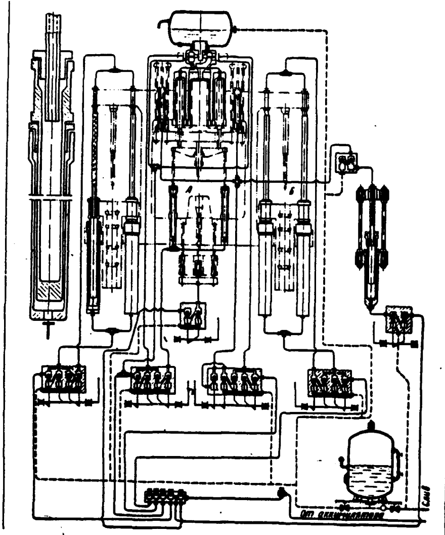
Fig. 102. Diagram paired piercing A (effort/force 400 t) and broaching B (with effort/force 150 t) press.
