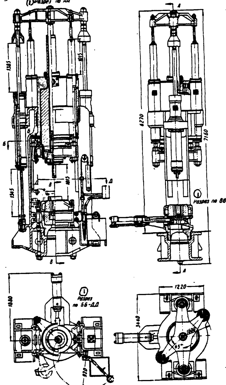
Fig. 88. Vertical bar-tube press with effort/force 600 t.
