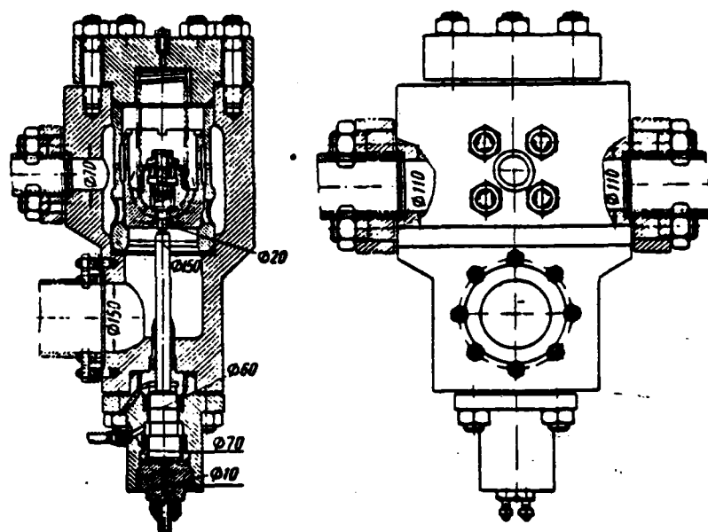
Fig. 332. Extended construction/design of filler valve.
