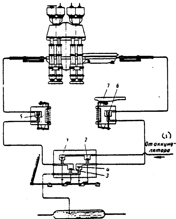
Fig. 356. The hydraulic schematic of the extensible table of stamping machine by effort/force 30000 t: 1 and 2 - pressure valves; 3 and 4 - drain valves; 5 and 6 - throttle (brake) valves; 7 - cams, fastened on roller table.
