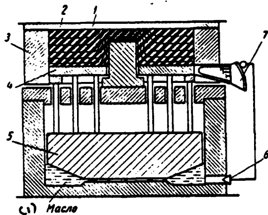
Fig. 73. The diagram of rubber-pad forming with deep drawing: 1 - slider; 2 - rubber pad; 3 - container; 4 - clamp; 5 - drive of clamp; 6 - pressure regulator; 7 - the cam gear of control of pressure regulator.
