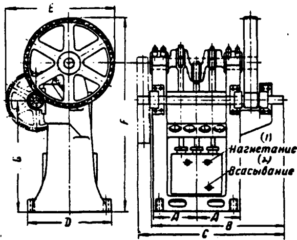
Fig. 253. Vertical three-plunger pump.
