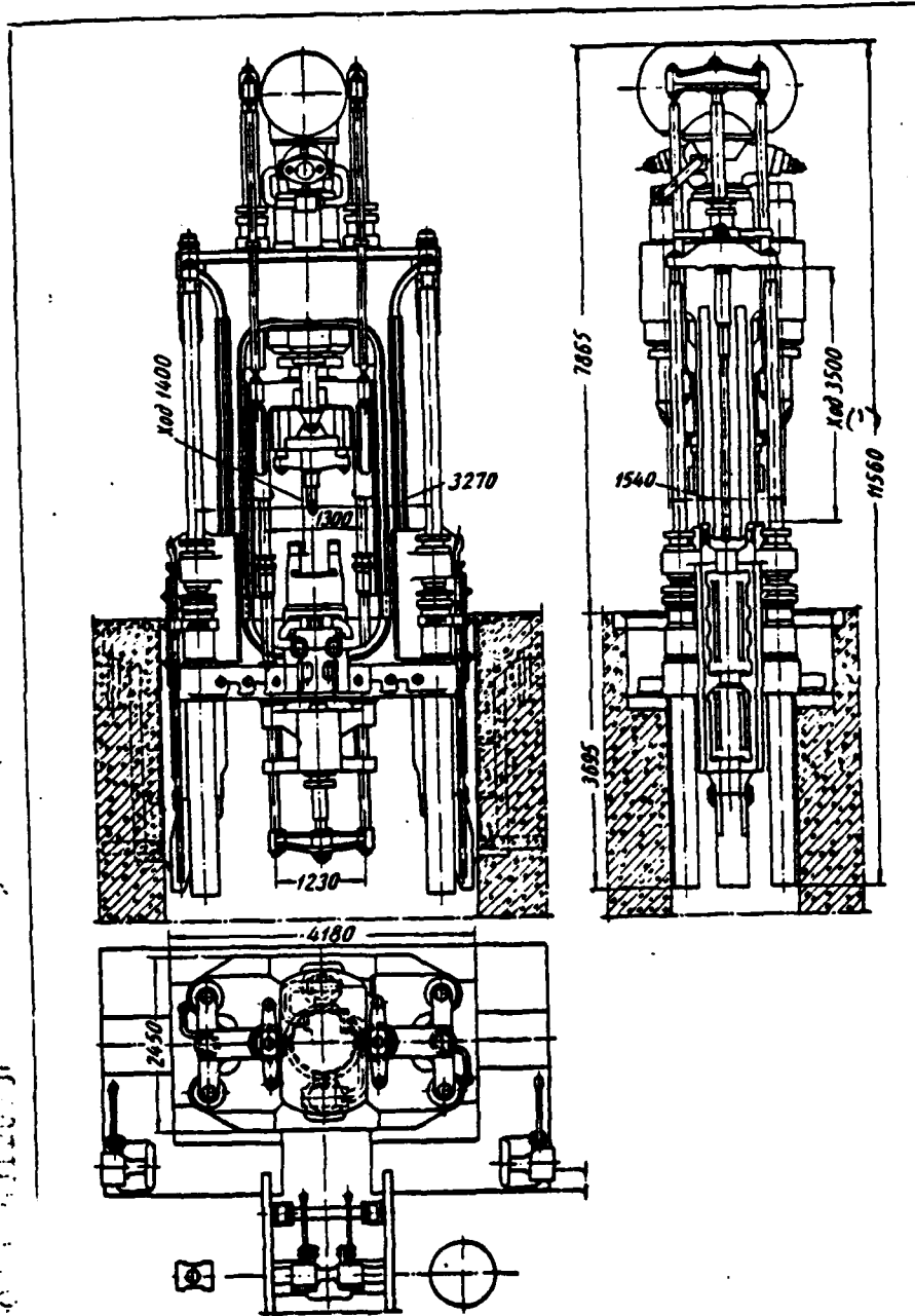
Fig. 101. Paired press: piercing by effort/force 400 t and drawn-out by effort/force 150 t.
