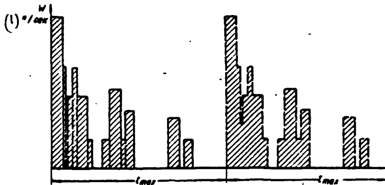
Fig. 288. Combined graph of fluid flow rate by presses.
