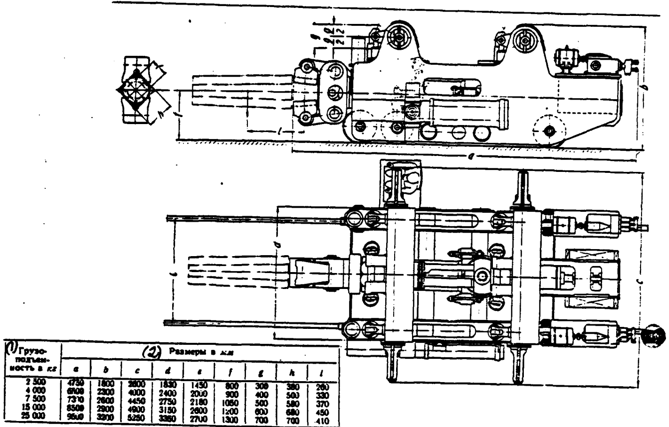
Fig. 30. Construction/design and the basic dimensions of manipulators with hydraulic drives of the mechanisms of trunk.
