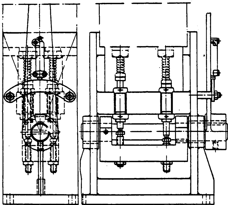
Fig. 393. Construction/design of hoisting device of valves.
