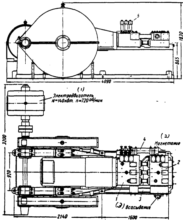
Fig. 256. The general view of three-plunger pump with two steps/stages of supply and pressure - 1200/360 \frac{1}{\text{min}} ; 50/175 \text{kg/cm}^2 : 1 - cylinder block of low-pressure; 2 - cylinder block of high-pressure; 3 - suction header; 4 - discharge header; 5 - safety valves.
