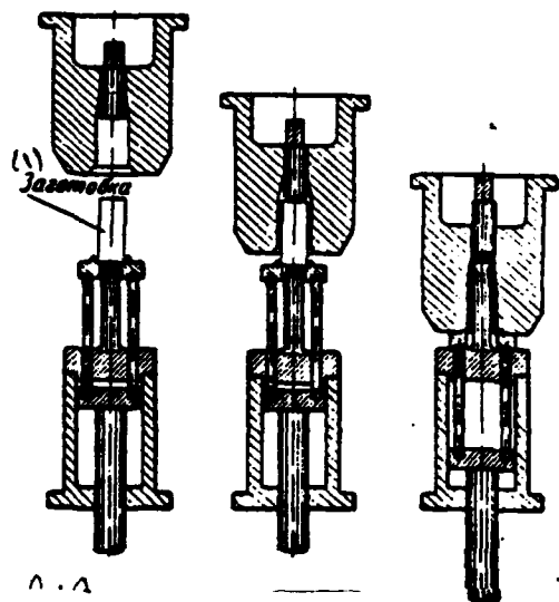
Fig. 98. Piercing in the container, fastened/strengthened to the slider of press.
