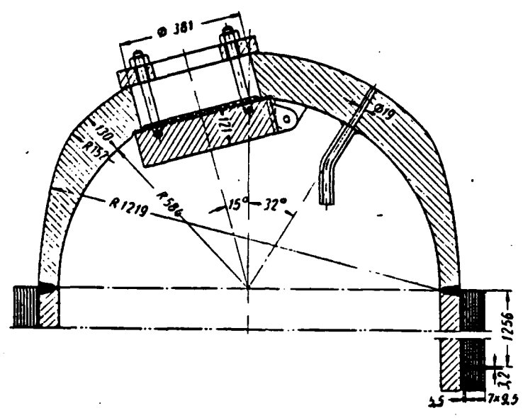
Fig. 322. Nose section of the multilayer welded bottle with the thick-walled internal shell.
