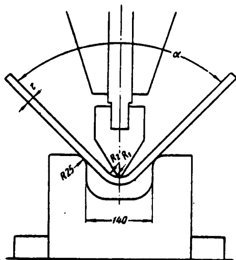
Fig. 81. Diagram of bending.
