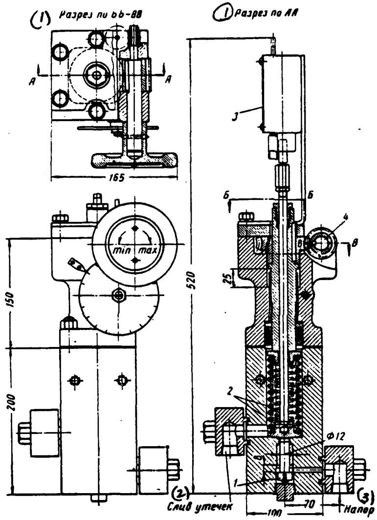
Fig. 378. Pressure relays with the plunger on the pressure 220 kg/cm 2 for the work on oil: 1 - plunger; 2 - load springs; 3 - terminal switch; 4 - mechanism for the tightening of springs.
