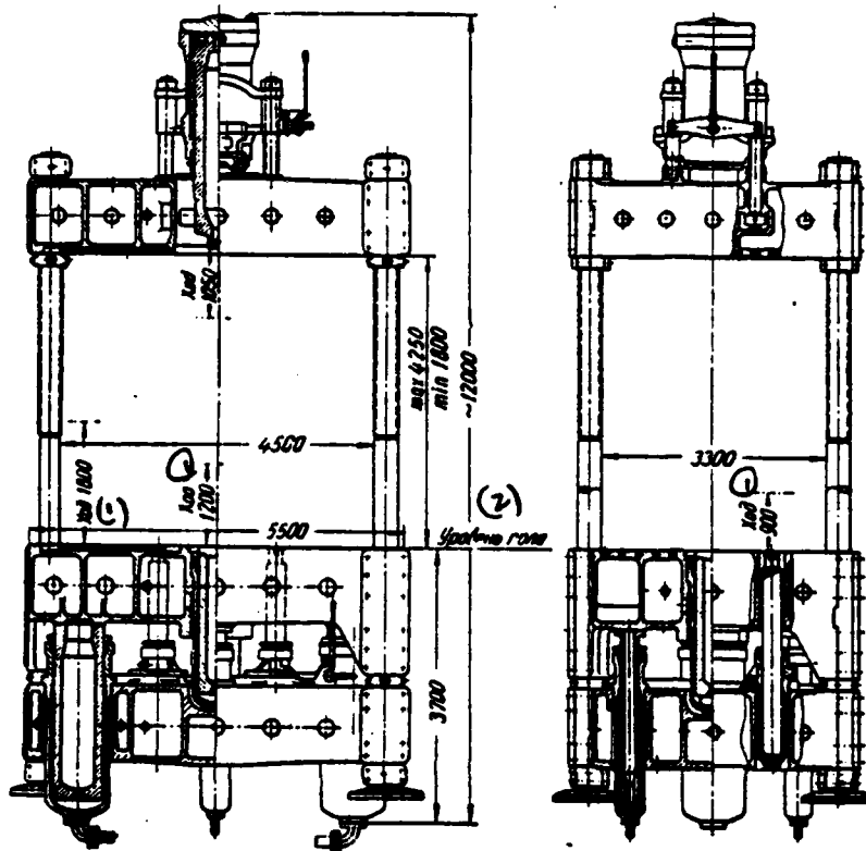
Fig. 58. Corner post-type press by effort/force 1500 t for the hot die forging of thick sheets with the lower arrangement of working cylinders.
