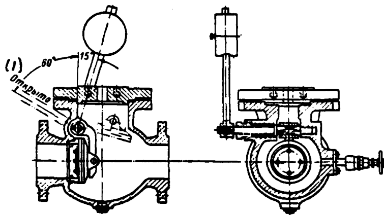
Fig. 327. Check valve with the load.
