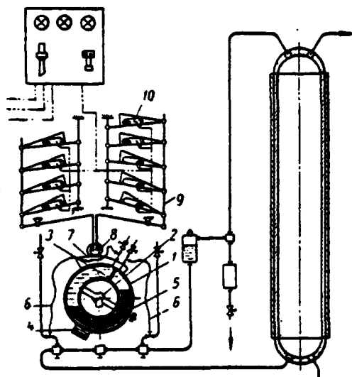
Fig. 306. Schematic of mercury apparatus with the rotary ring for the checking of the levels of liquid in the storage battery/accumulator.
