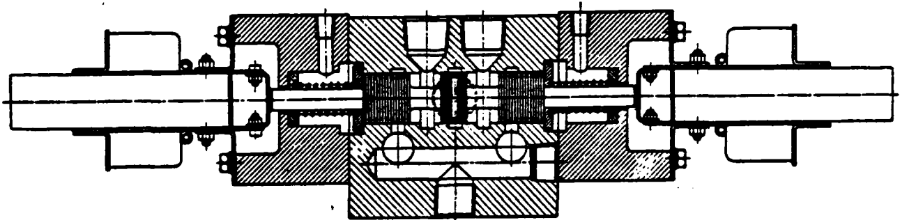
Fig. 362. Valve, moved by electromagnets.
