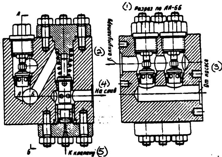
Fig. 294. Construction/design of the bypass valve of pump.
