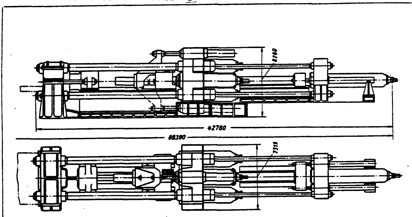
Fig. 95. The general view of bar-tube press with effort/force 18000 t.
