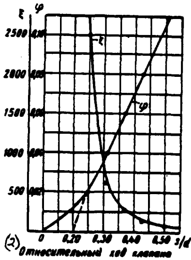
Fig. 225. Dependence \xi=f(s/d) and \phi=f(s/d) for the throttle valve with the "cup".
