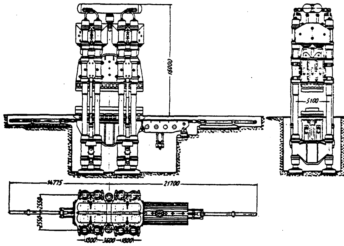
Fig. 42. Eight-cylinder hydraulic stamping machine 30000 t. General view.
