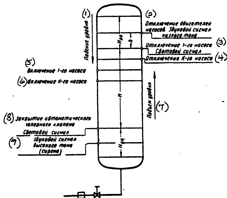
Fig. 293. Controlled/inspected levels of liquid in the storage battery/accumulator: H , H_{ав} and H_{ст} — respectively the height/altitude of working, emergency and standby liquid columns.
