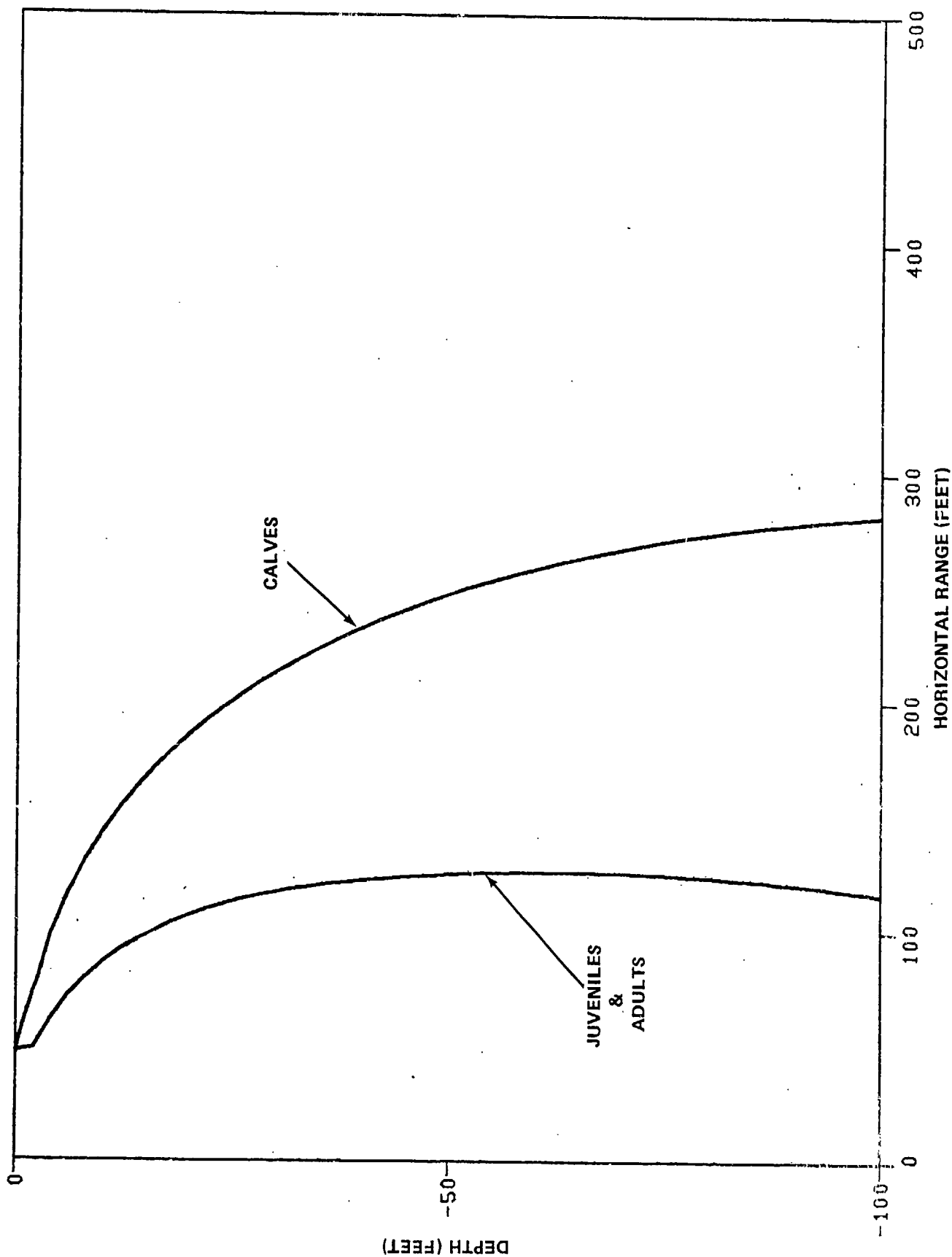
FIGURE 3.4.1. CONTOURS FOR SLIGHT INJURY TO MANATEES: 12-LB CHARGE AT 5-FT DEPTH
