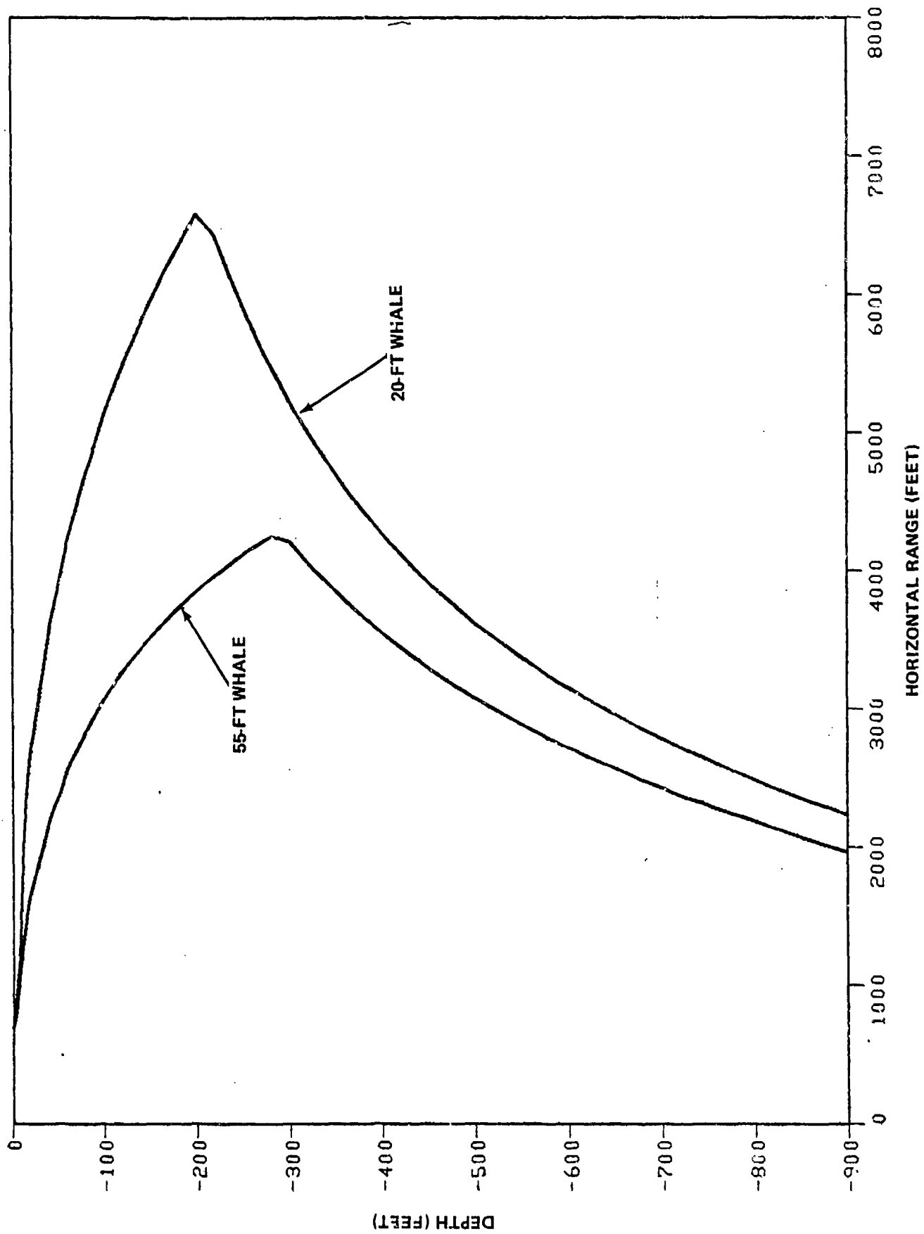
FIGURE 3.1.3. CONTOURS FOR SLIGHT INJURY TO WHALES: 40,000-LB CHARGE AT 200-FT DEPTH
