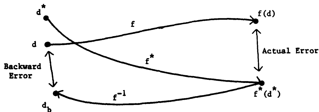
FIGURE 2.4 Illustration of backward error.
