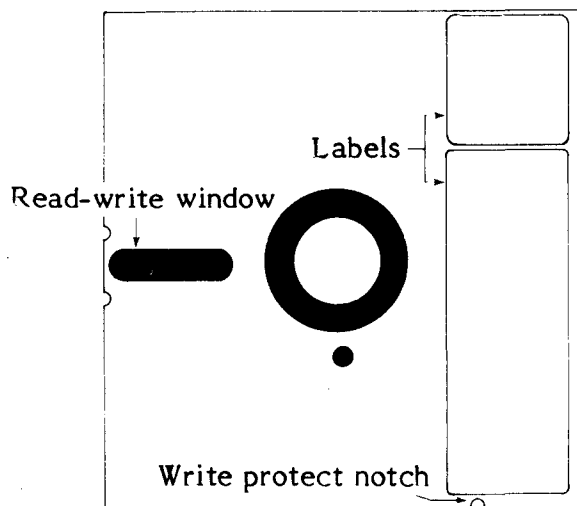
Figure 9. Floppy diskette.
