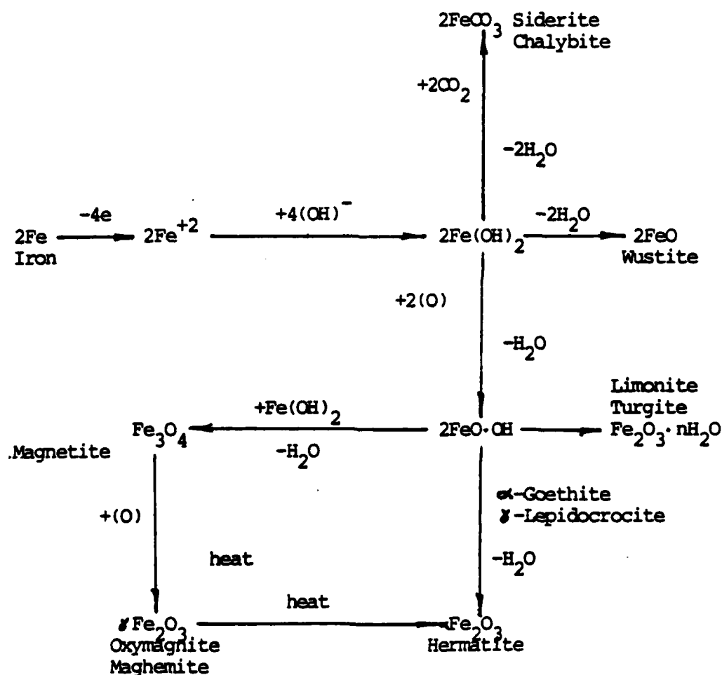
Figure 3.6 Notational reactions in the formation of rust. 7
