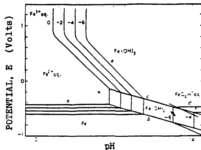
Figure 3.3 Simplified potential/pH diagrams for the \text{Fe}/\text{H}_2\text{O} 6 system showing the zones of thermodynamic stability of cations, anions, and hydroxides of iron (Deltombe and Pourbaix).
