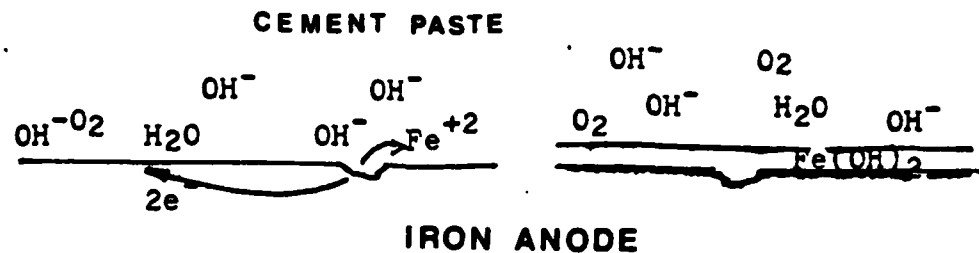
Figure 3.5 Corrosion process at the metal surface.
