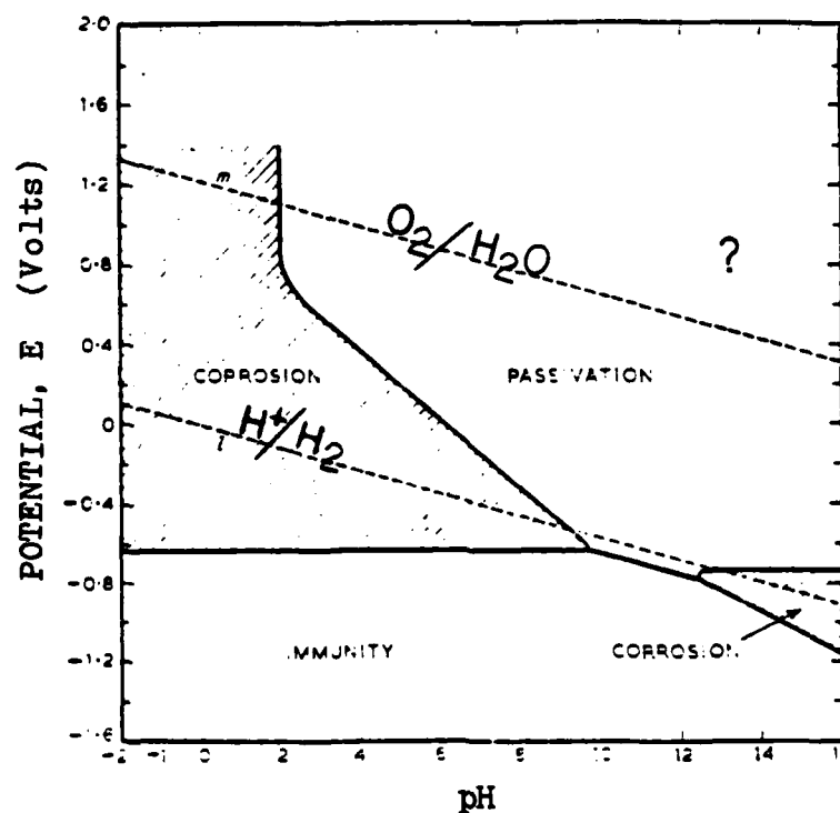
Figure 3.4 Simplified potential/pH diagram showing the 6 zones of corrosion, immunity, and passivation.
