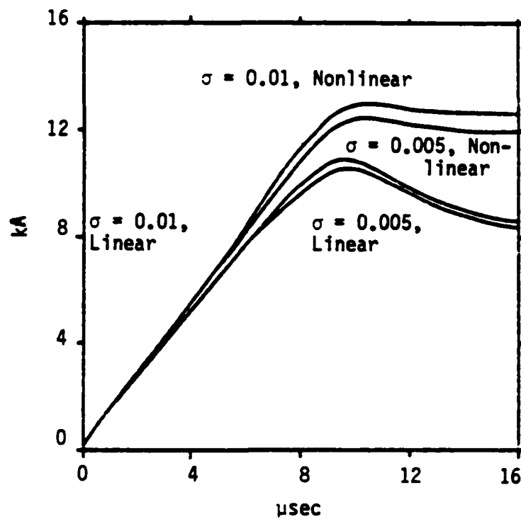
Figure 3.17 Tactical Short Circuit Current for 600 m RG 58.
