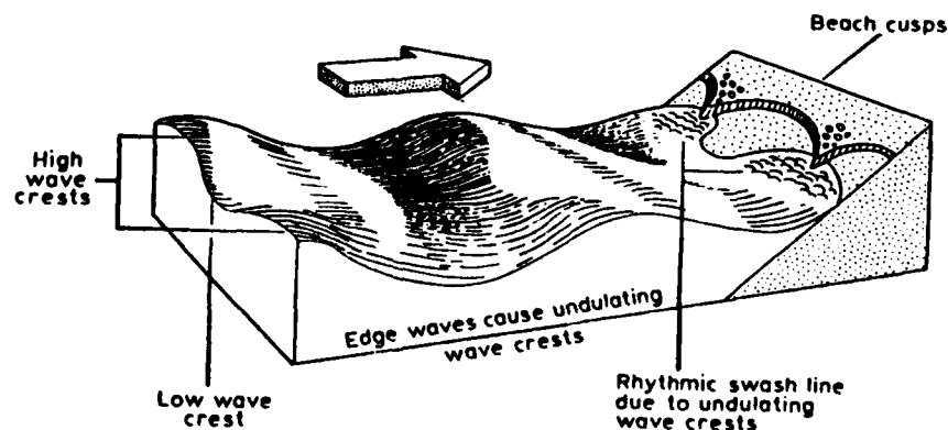
Figure 2. The relationship between edge-waves and beach cusps.
