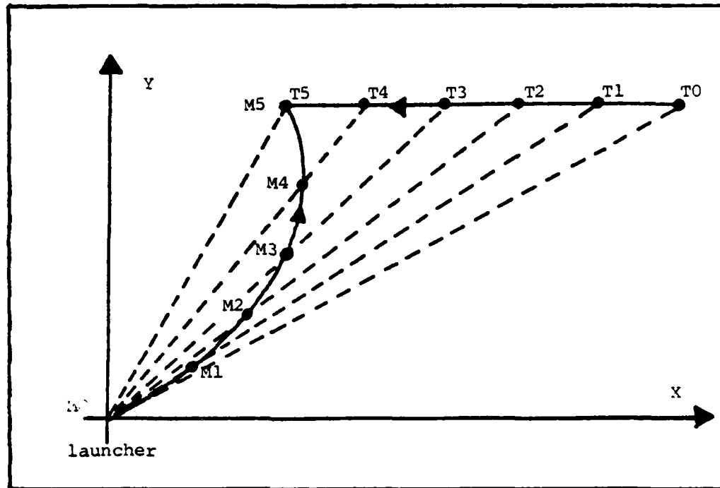
Figure 2.1 Missile Target Encounter with LOS Guidance
