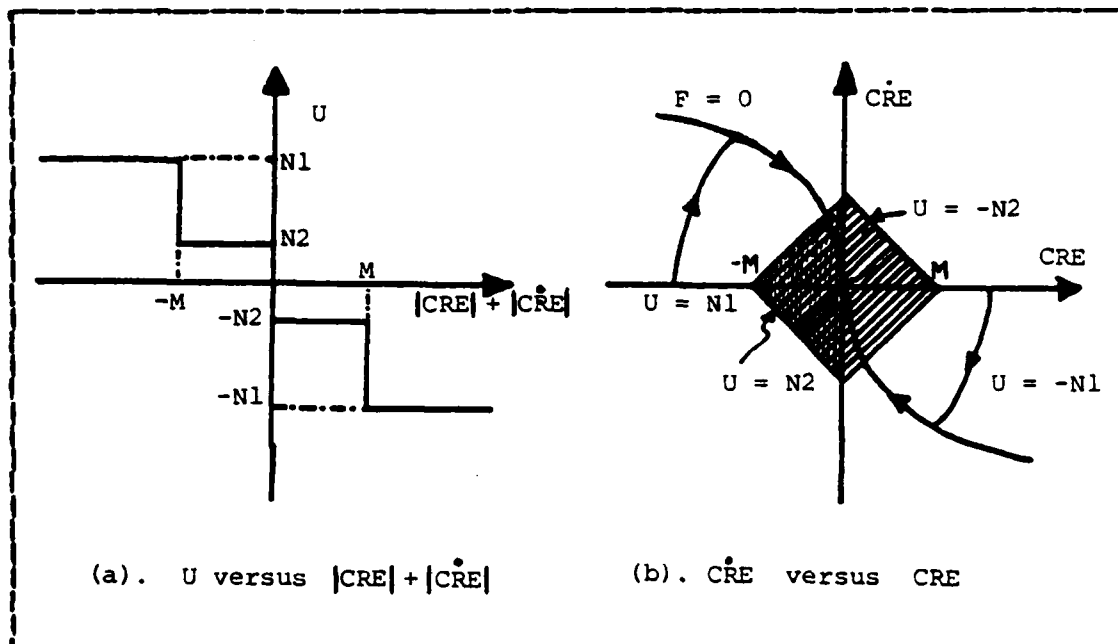
Figure 7.1 Two-Level Relay
