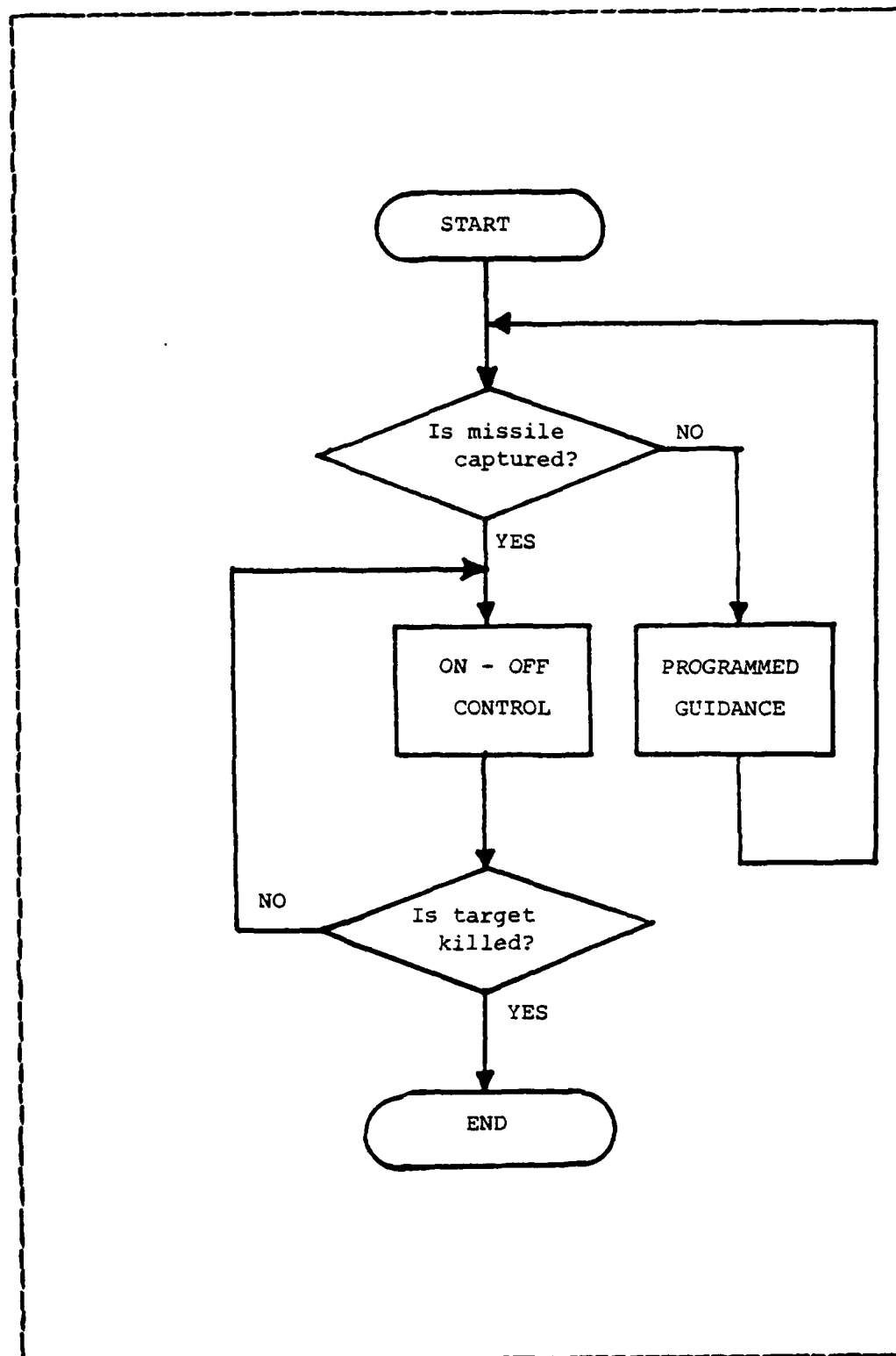
Figure 5.1 Simplified Flow Chart of Basic LOS Control
