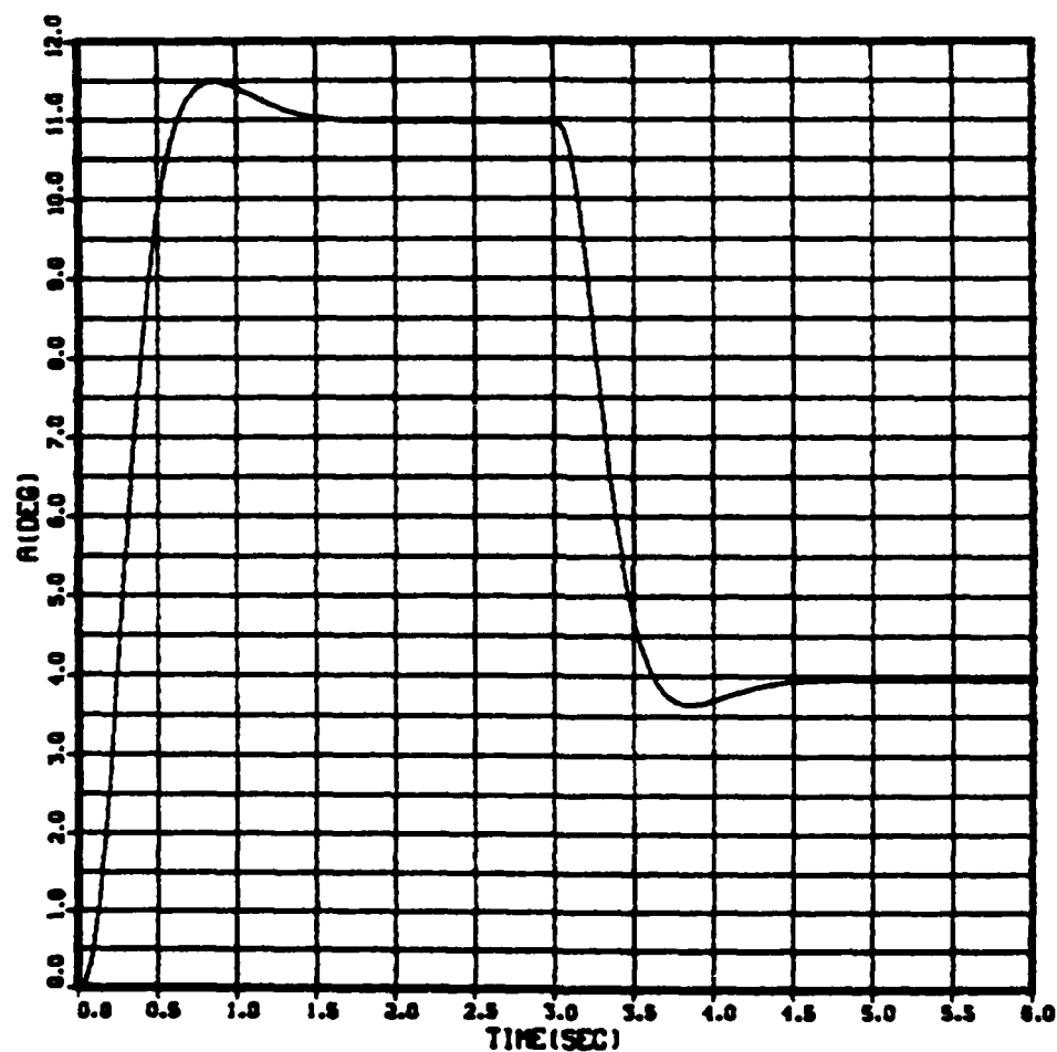
Fig. 4.45 Angle of Attack (a) vs Time (t) CBTT of Circular airframe; Faster Pitch channel; inertial and kinematic cross-coupling into Pitch channel removed; 2 Gees ( 0^\circ , 180^\circ ), K_{A_3} = -0.0387
