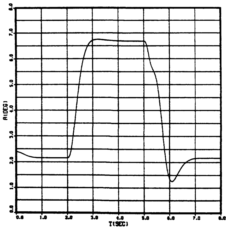
Fig. 4.8 Angle of Attack ( \alpha ) vs Time ( t ) CBTT of Elliptical airframe; 2 Gees ( 0^\circ , 180^\circ )
