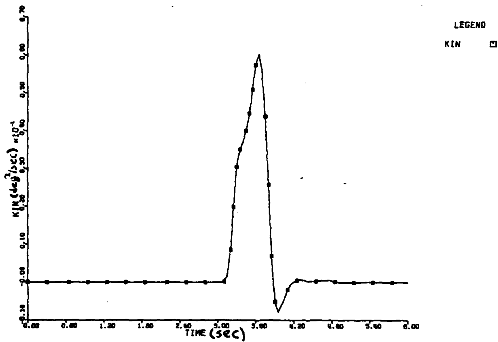
Fig. 5.28 Minimized Kinematic Coupling (-P.β) vs Time (t) CBTT of Circular airframe
