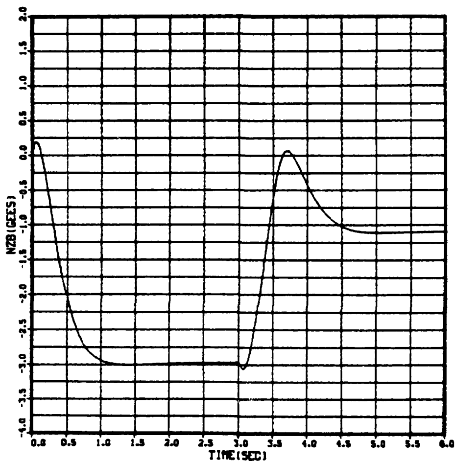
Fig. 4.29 Achieved Body-fixed Acceleration ( n_z ) vs Time ( t ) CBTT of Circular airframe; 2 Gees ( 0^\circ , 180^\circ ), K_A = -0.0274
