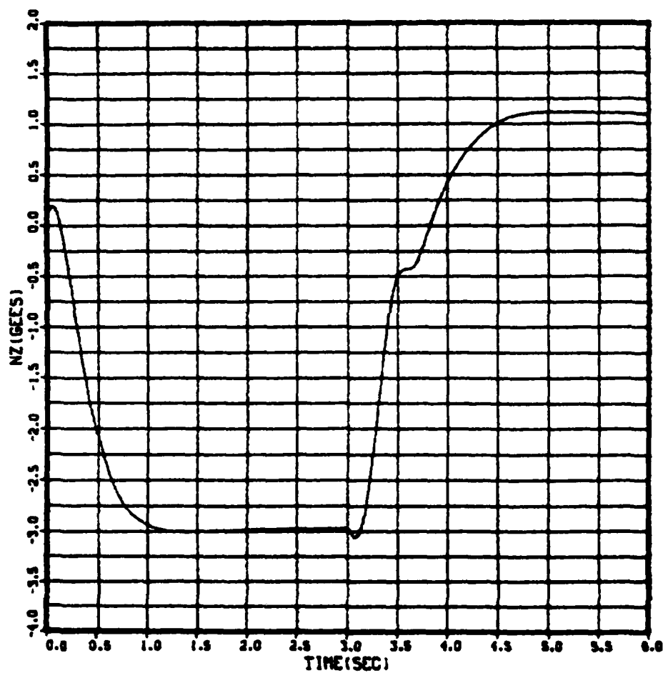
Fig. 4.28 Achieved Inertial Acceleration ( n_z ) vs Time ( t )
