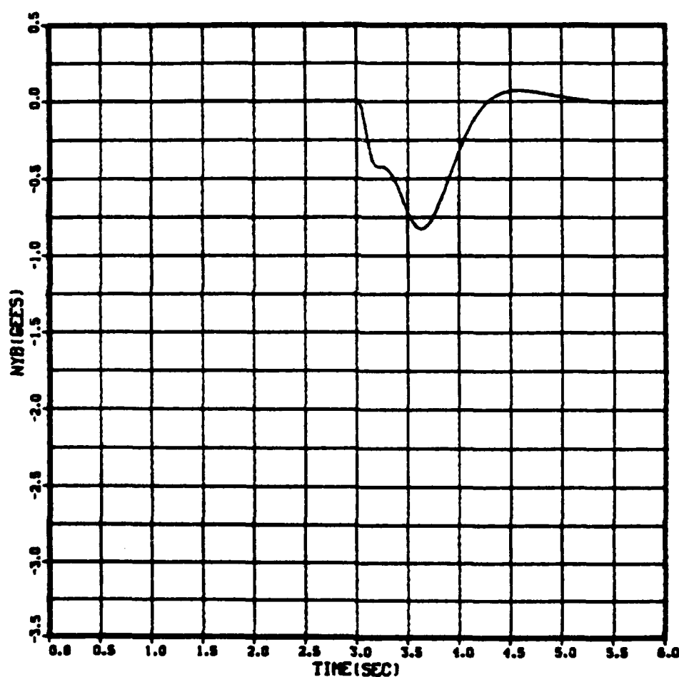
Fig. 4.44 Achieved Body-fixed Acceleration ( n_{y_B} ) vs Time (t) CBTT of Circular airframe; Faster pitch channel; inertial and kinematic cross-coupling into pitch channel removed; 2 Gees ( 0^\circ , 180^\circ ), K_{A_3} = -0.0387
