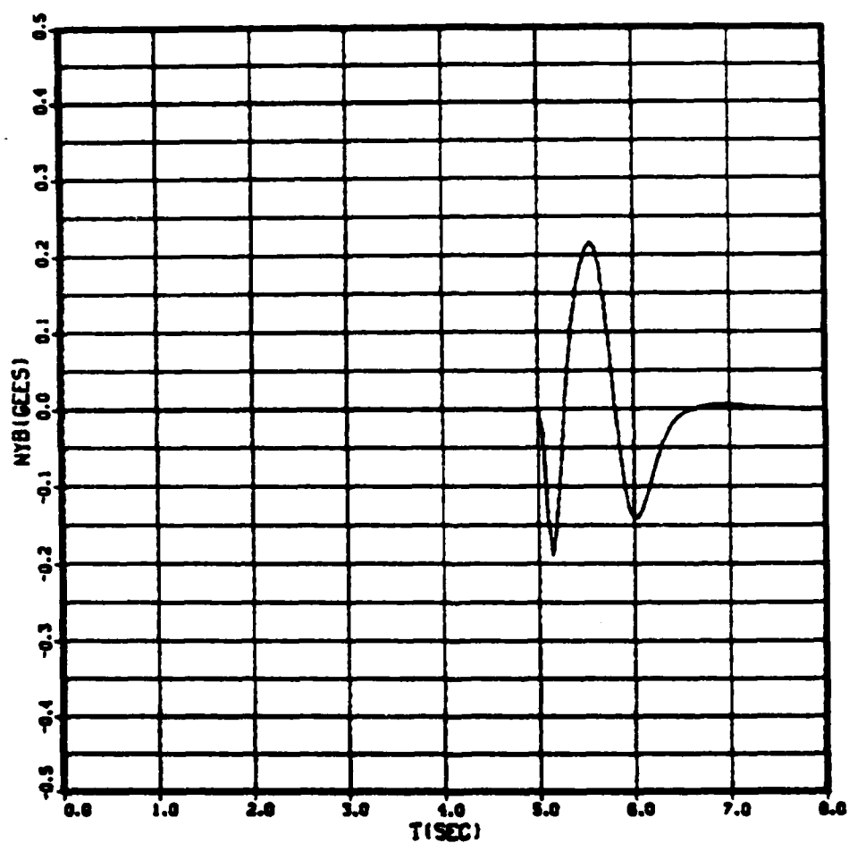
Fig. 4.7 Achieved Body-fixed Acceleration ( n_{y_B} ) vs Time (t) CBT of Elliptical airframe; 2 Gees ( 0^\circ, 180^\circ )
