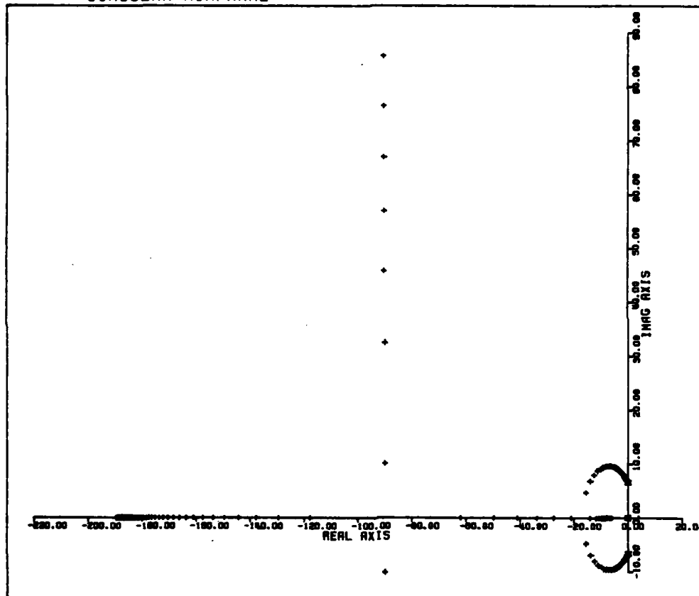
Fig. 5.19 Root locus of SAS with a/\delta_p CBTT of Circular airframe
