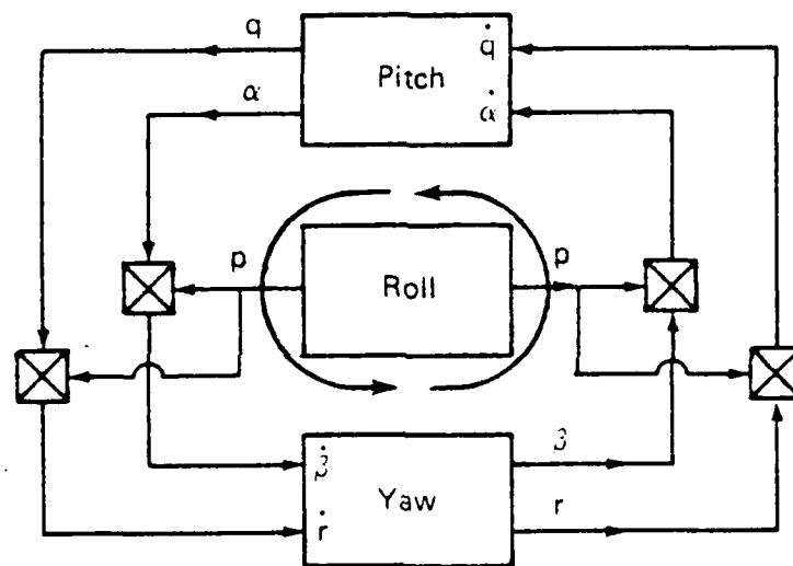
Fig. 4.25 Critical Feedback loop for CBTT
