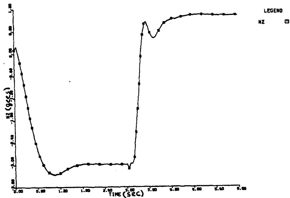
Fig. 5.25 Achieved Inertial Acceleration ( n_z ) vs Time (t)
