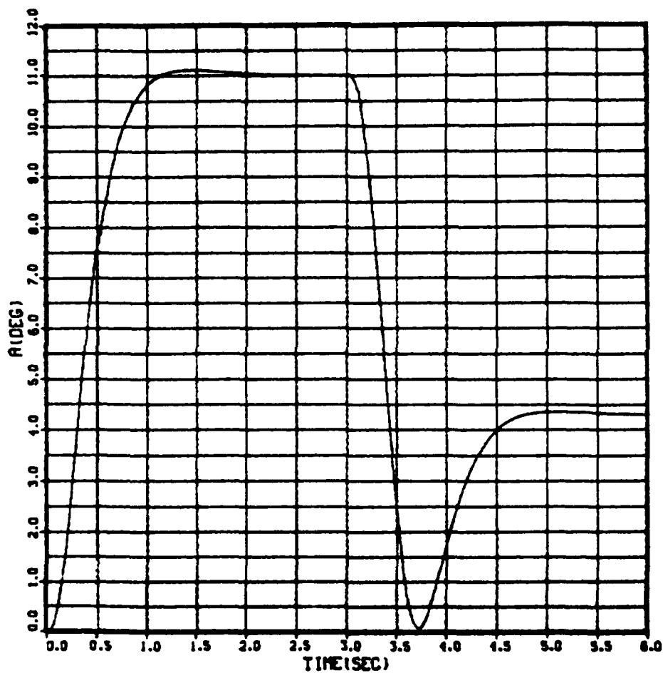
Fig. 4.31 Angle of attack (a) vs Time (t) CBTT of Circular airframe; 2 Gees ( 0^\circ , 180^\circ ), K_{A_1} = -0.0274
