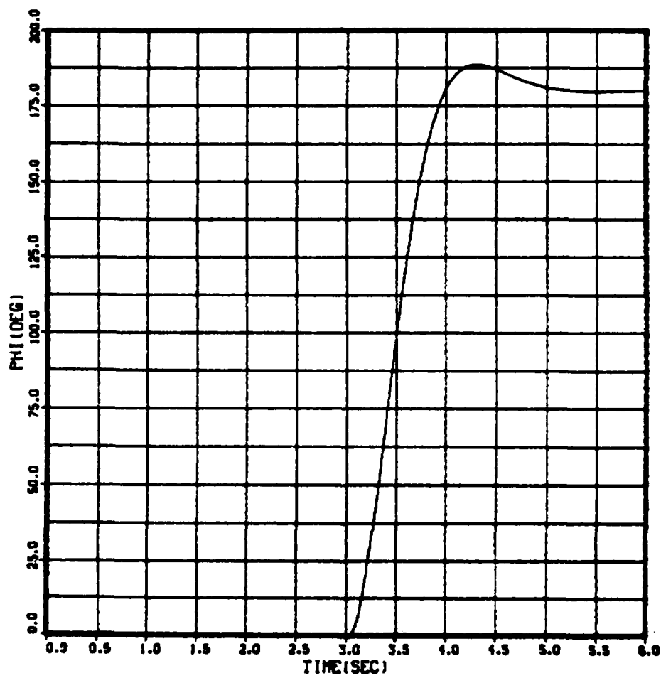
Fig. 4.36 Roll angle ( \phi ) vs Time ( t ) CBTT of Circular airframe; 2 Gees ( 0^\circ, 180^\circ ), K_{A_1} = -0.0274
