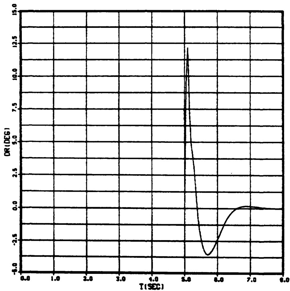
Fig. 4.16 Roll tail incidence ( \delta_R ) vs Time ( t ) CBTT of Elliptical airframe; 2 Gees ( 0^\circ , 180^\circ )
