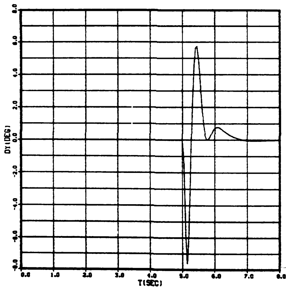
Fig. 4.15 Yaw tail incidence ( \delta_y ) vs Time ( t ) CBTT of Elliptical airframe; 2 Gees ( 0^\circ , 180^\circ )
