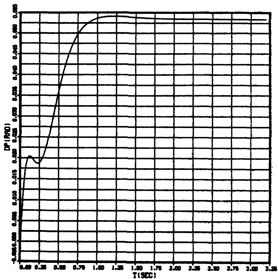
Fig. 2.9 Pitch Tail Incidence ( \delta_p ) vs Time (t)
