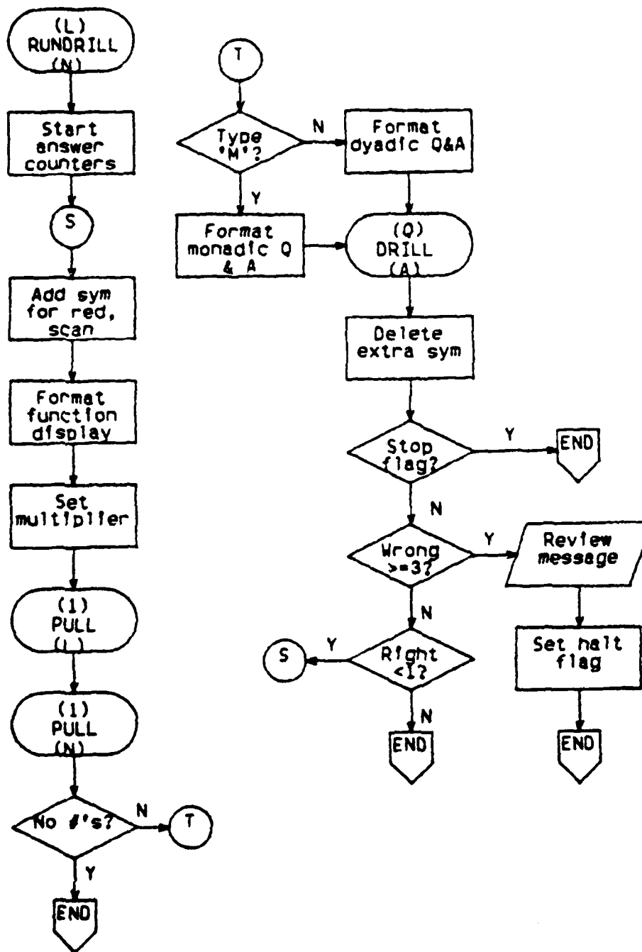
Figure B.15 Procedure of RUNDRIIL Function.
