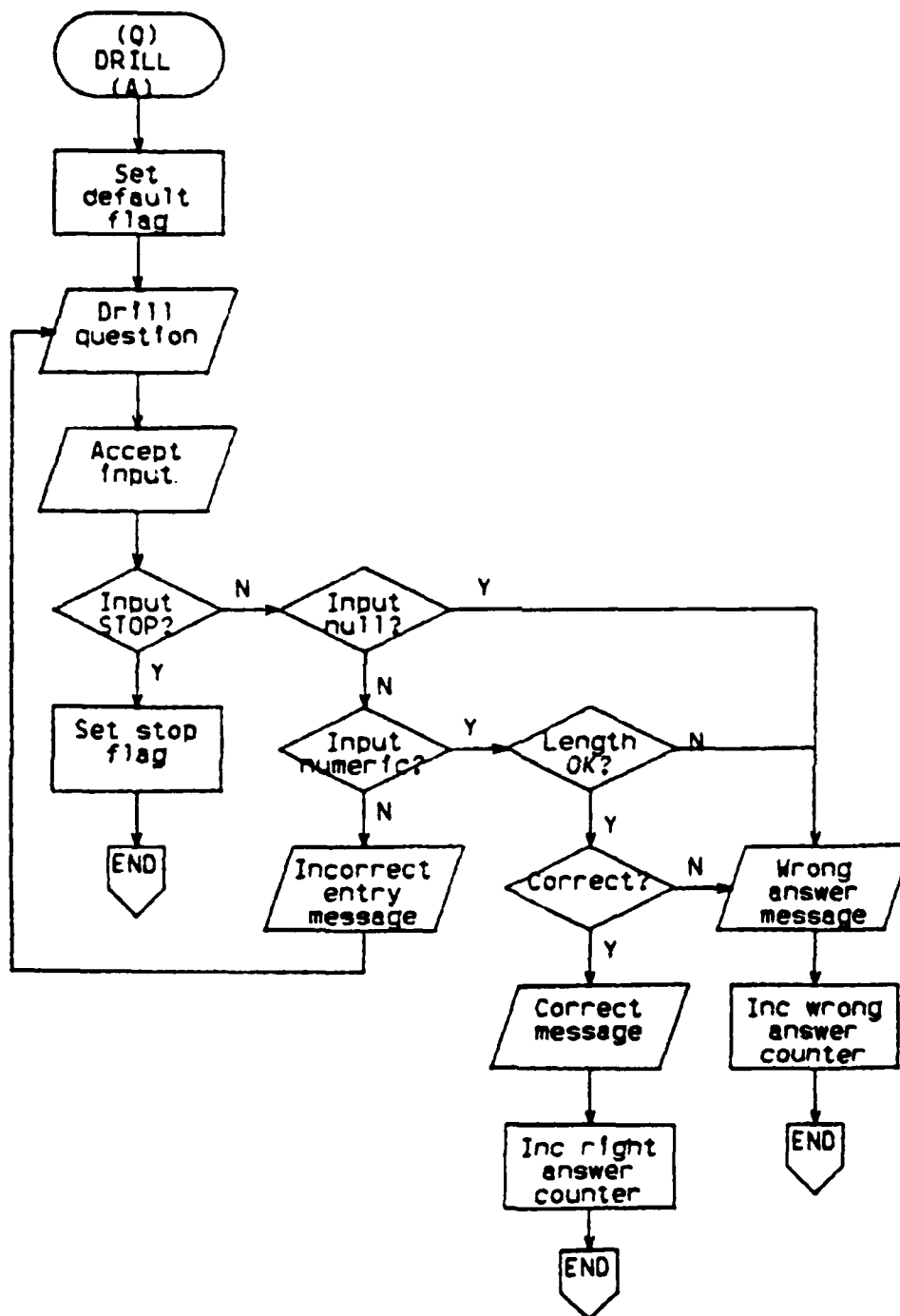
Figure B.16 Procedure of DRILL Function.
