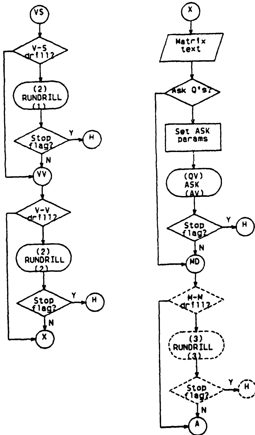
Figure B.10 Procedure of SHOW Function--2.
