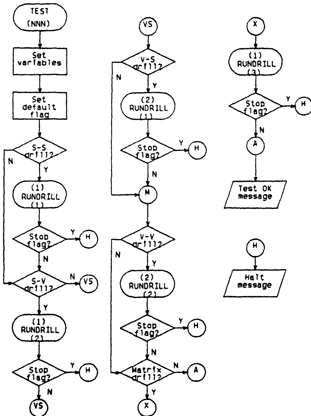
Figure B.20 Procedure of TEST Function.
