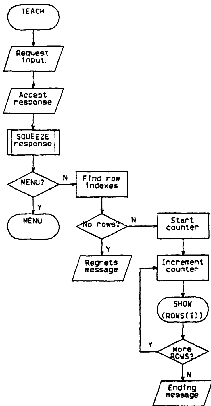
Figure B.7 Procedure of TEACH Function.
