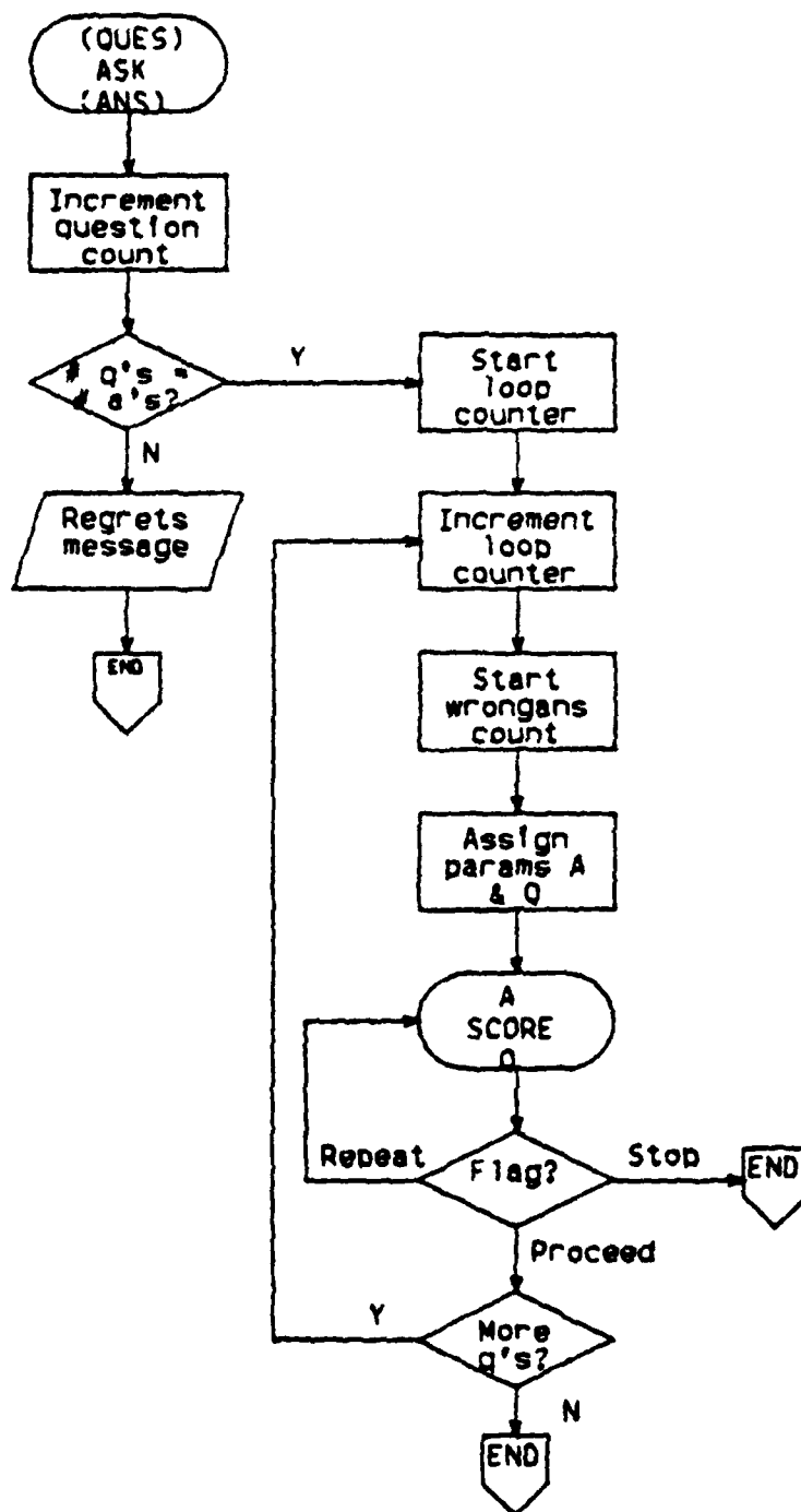
Figure B.12 Procedure of ASK Function.
