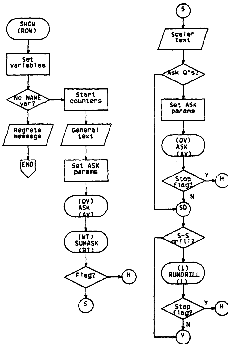
Figure B.9 Procedure of SHOW Function--1.
