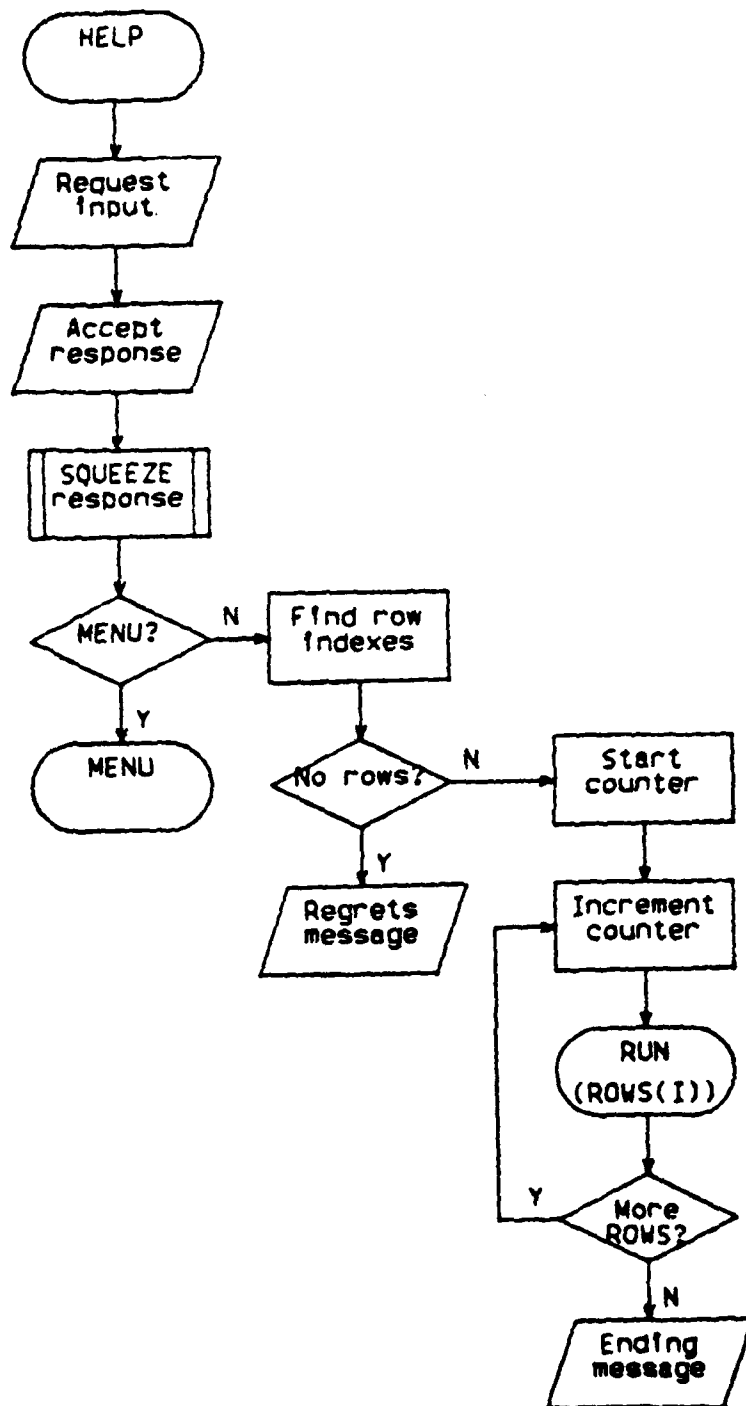
Figure B.4 Procedure of HELP Function.
