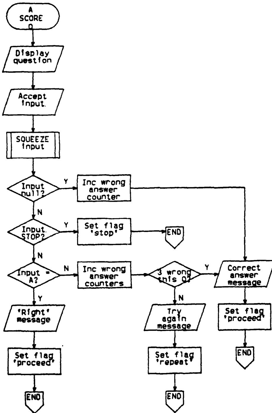
Figure B.14 Procedure of SCORE Function.
