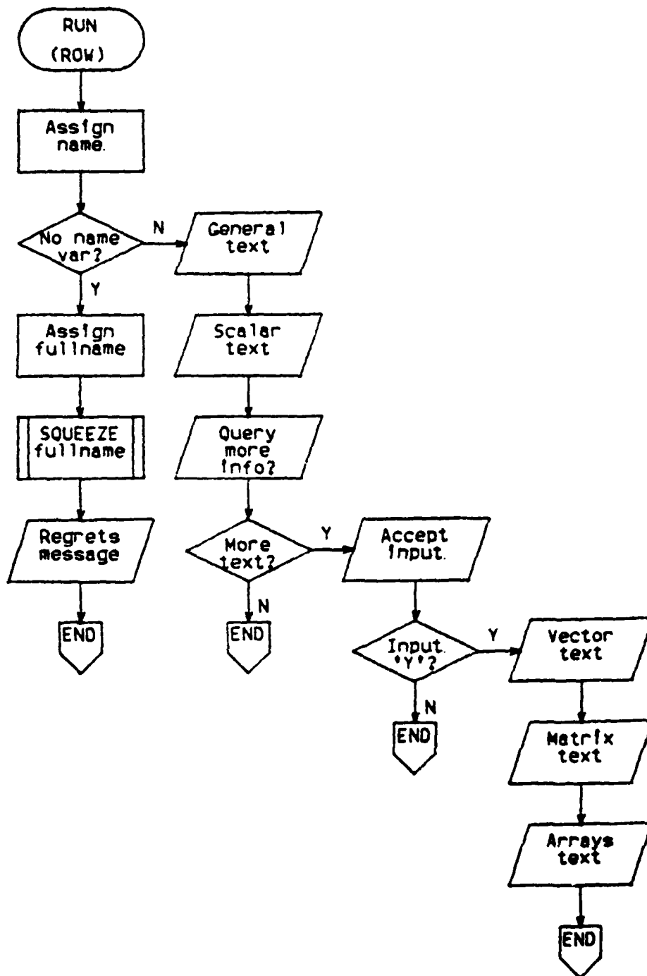
Figure B.6 Procedure of RUN Function.
