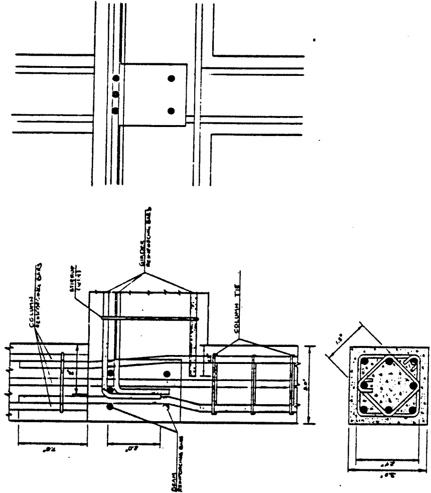
2/5 DETAIL OF GIRDER-COLUMN CONNECTION EXTERIOR COLUMNS
