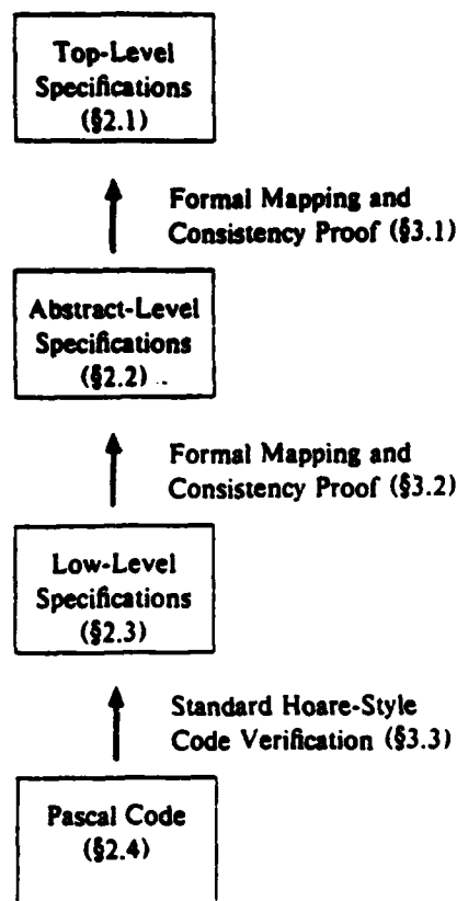
Fig. 1. Specification levels and consistency proofs.
