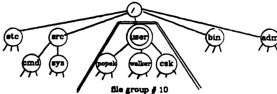
Figure 4b: Pathname Tree After Mounting File Group 10
