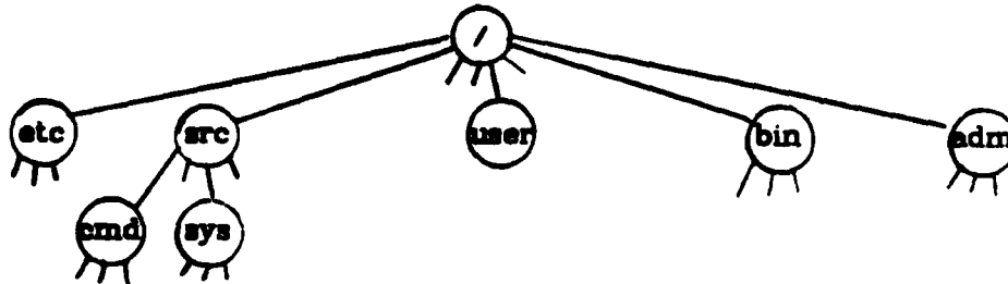
Figure 4a: Pathname Tree Before Mounting File Group 10
