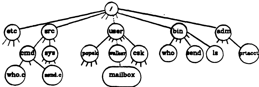
Figure 1: Hierarchical Naming
