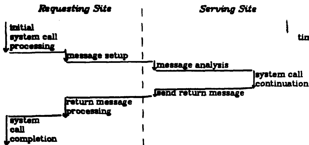
Figure 5: Processing a System Call Requiring Foreign Service
