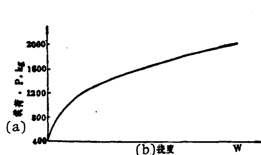
Fig. 6. Load (P)--deflection (W) curve, test specimen I. Key: (a) Load; (b) Deflection.
