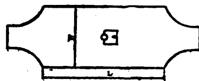
Fig. 1. Test specimen of crack toughness of PMMA.
