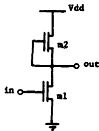
Fig. 4.1 NMOS Inverter
