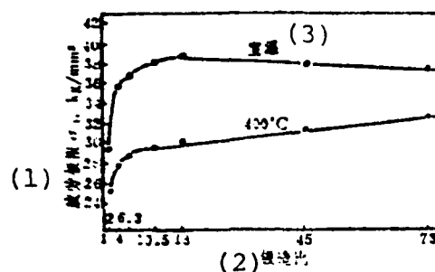
Fig. 8 Influence of forging ratio on fatigue limit of Cr steel. Key: (1) Fatigue limit; (2) Forging ratio; (3) Room temperature.
