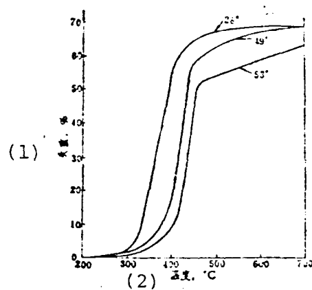
Fig. 4 Curves of heat loss of weight properties of number 648 epoxy cast resin with different molecular weights.
