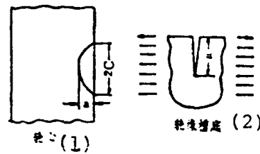
Fig. 7 Simplified mechanical calculation model chart of cracks of turbine disk's wheelboss and rim positions.
