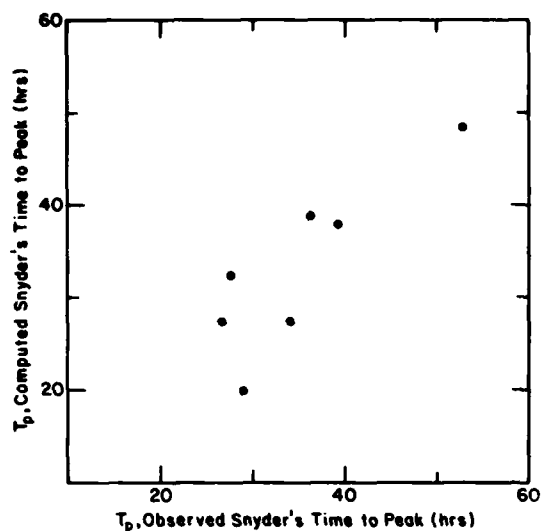
a. Snyder's time to peak, T_p .
