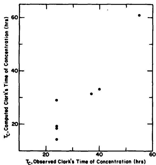
c. Clark's time of concentration, T_c .
