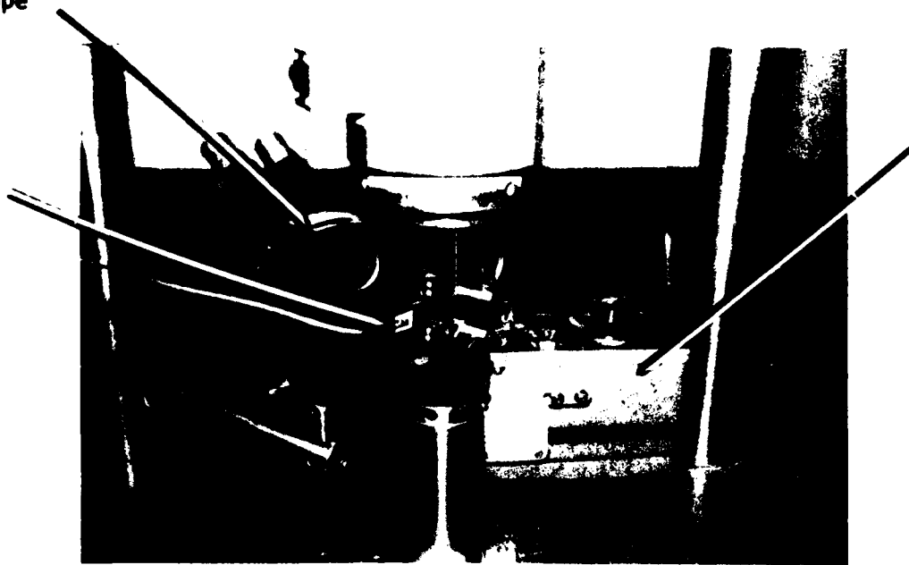
Figure 17. CT Specimen in load frame showing strobe and microscope for visual examination and COD gage for crack length measurement
