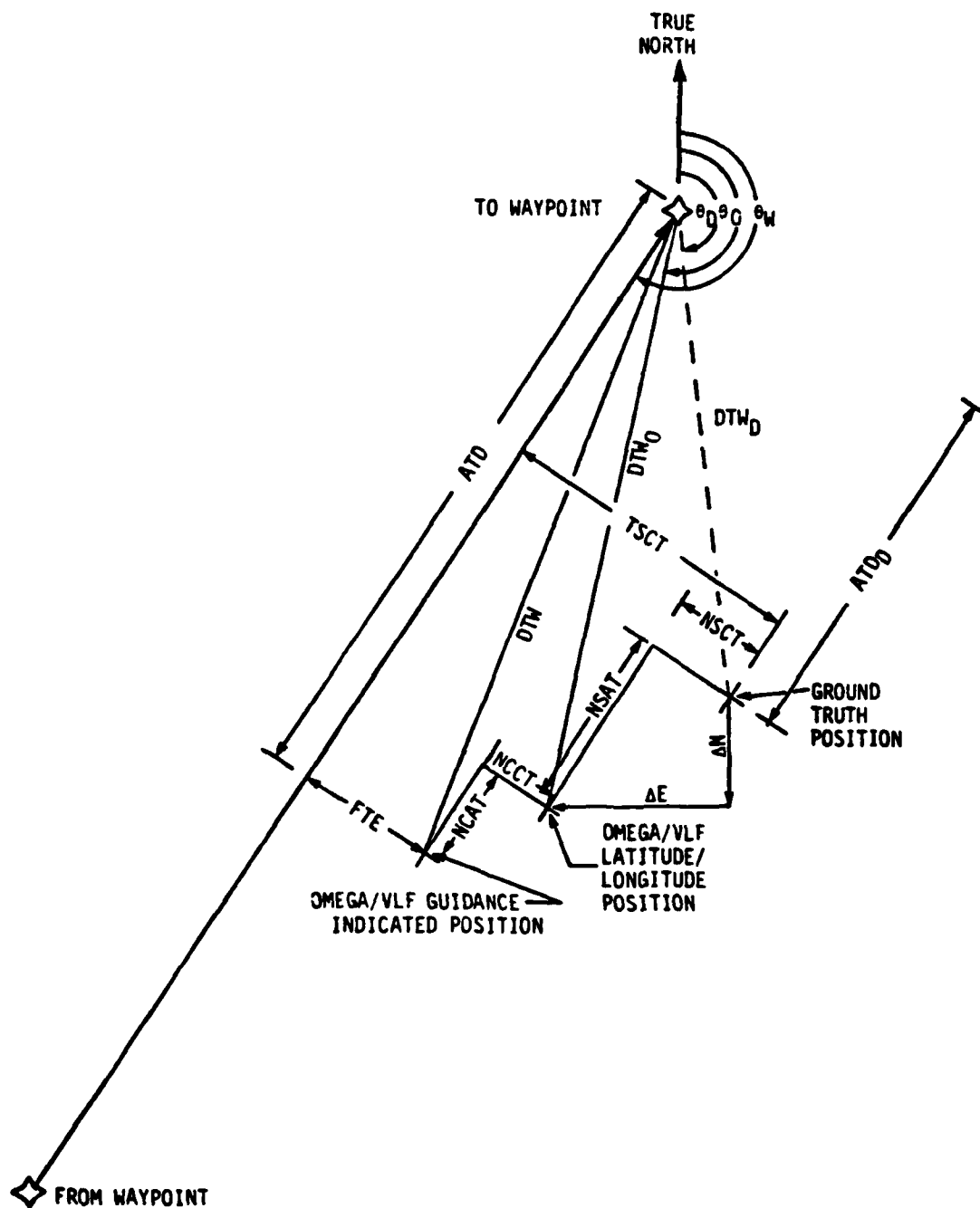
Figure 4.2 Omega/VLF System Error Geometry
