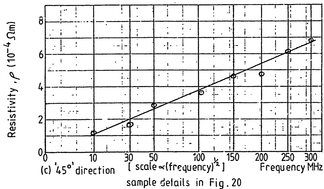
Figure 21 Resistivity-frequency characteristics for sample I
