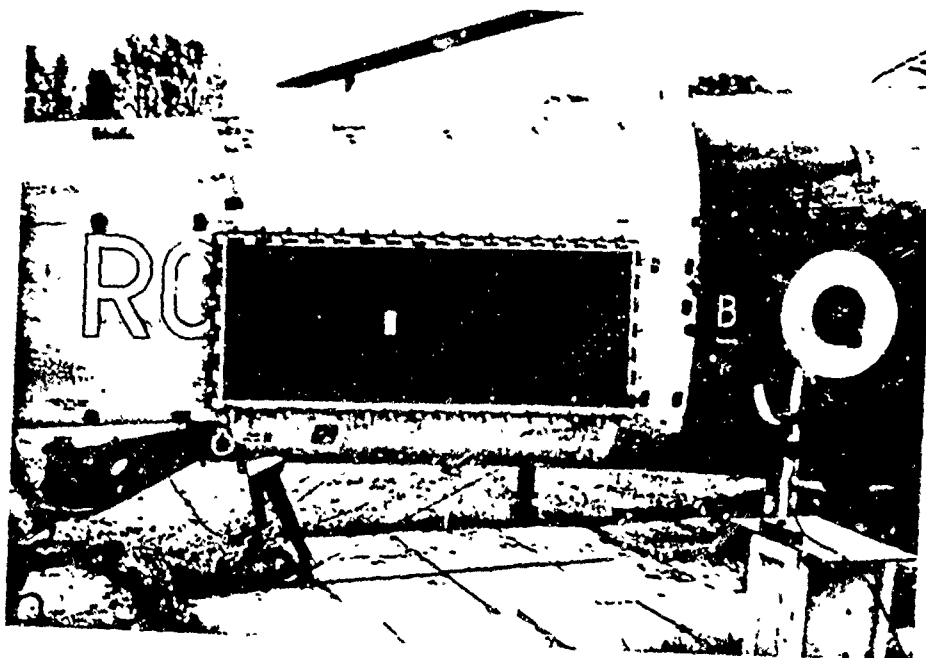
Figure 1 Modified Wessex tail cone showing mounted test panel
