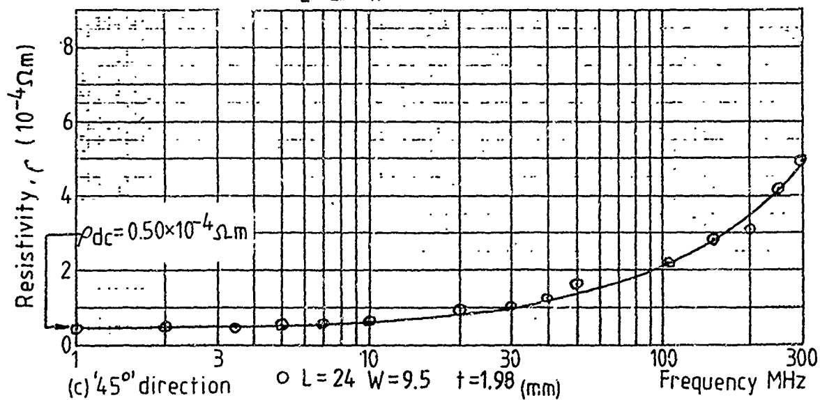
Figure 10 Resistivity-frequency characteristics for sample D
