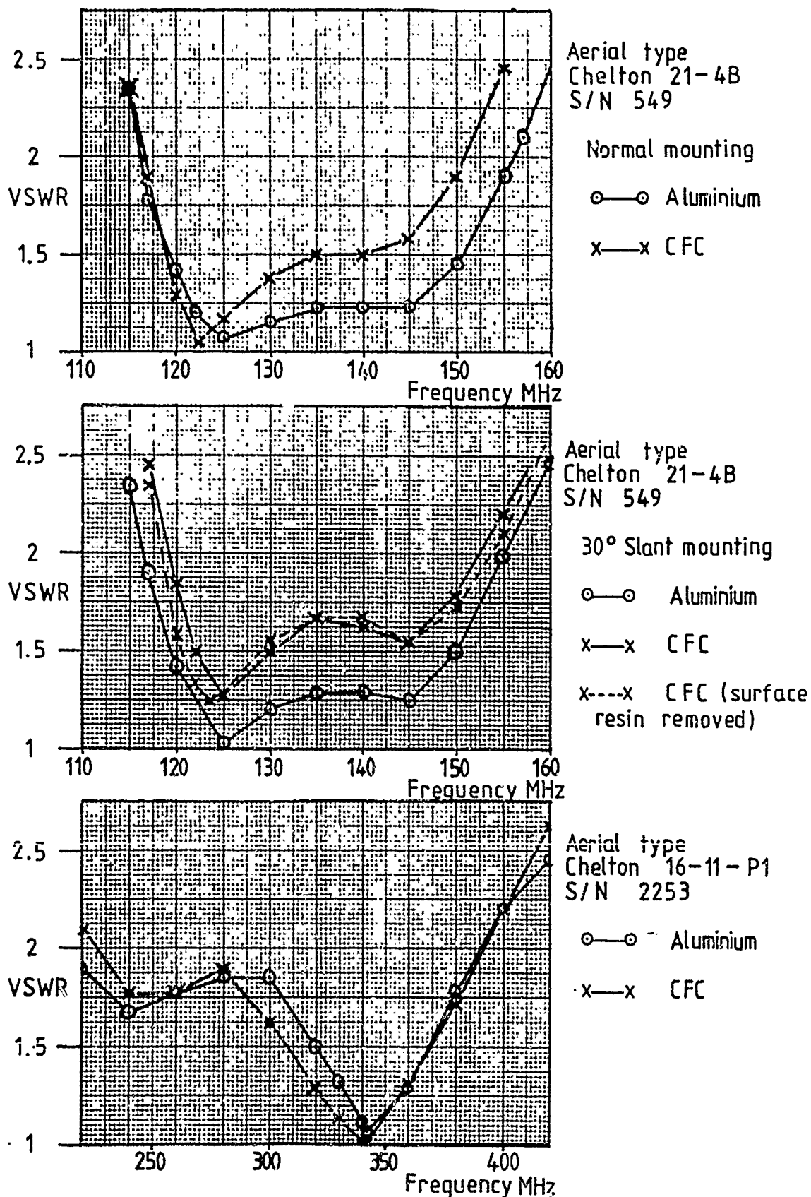
Figure 6 Comparison of VSWR for aeriels mounted on CFC and aluminium cylinders
