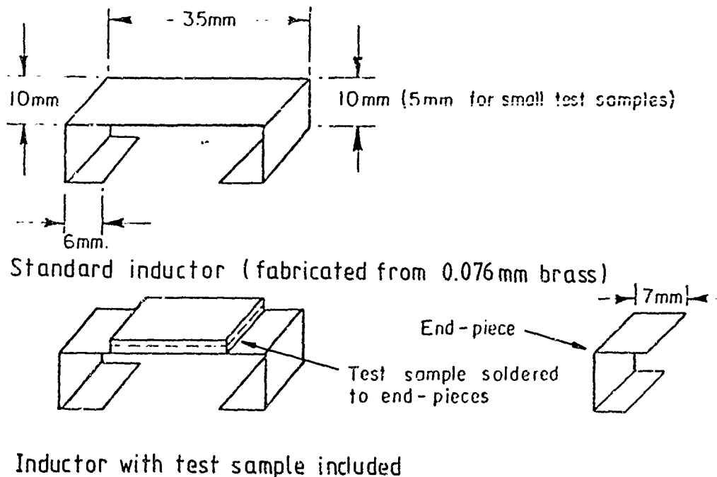
Figure 3 Test samples for 100-300 MHz
