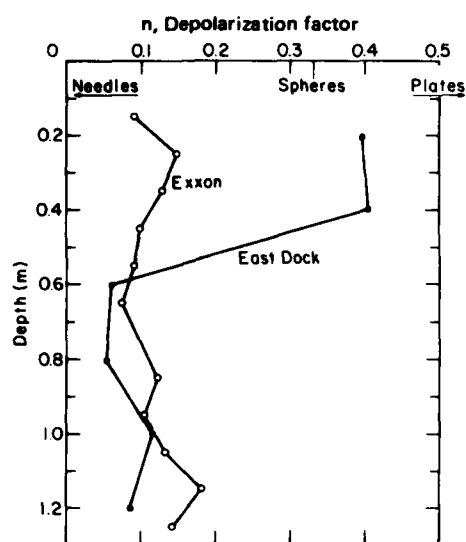
Figure 33. The depolarization factor as a function of depth at the Exxon and East Dock sites.
