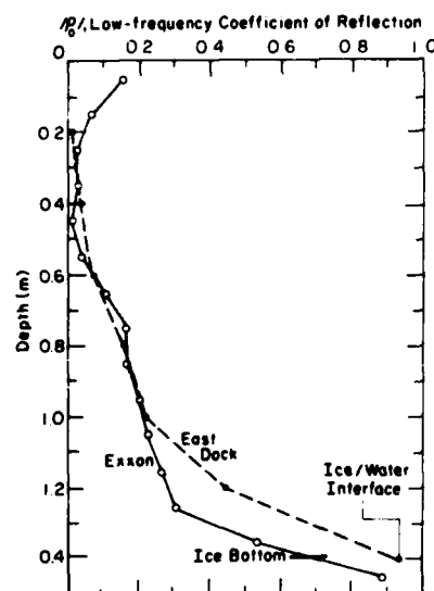
Figure 19. Magnitude of the low-frequency coefficient of reflection as a function of depth for the ladder arrays at the Exxon and East Dock sites.
