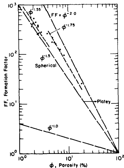
Figure 26. Formation factor as a function of porosity.
