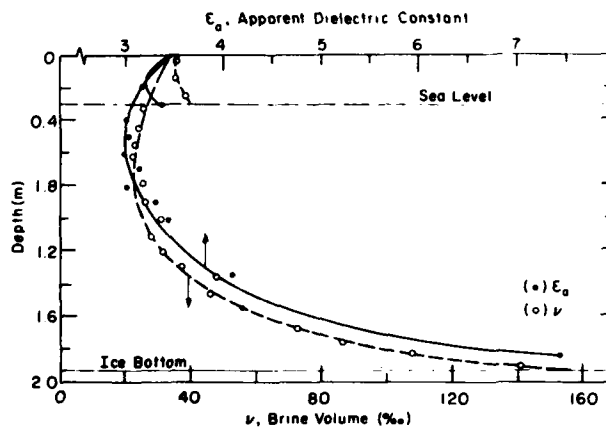
Figure 10. Apparent dielectric constant and brine volume as a function of depth at Exxon ice island site, 1979.
