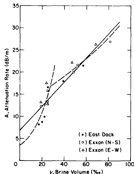
Figure 37. Attenuation rate as a function of brine volume calculated at 100 MHz.
