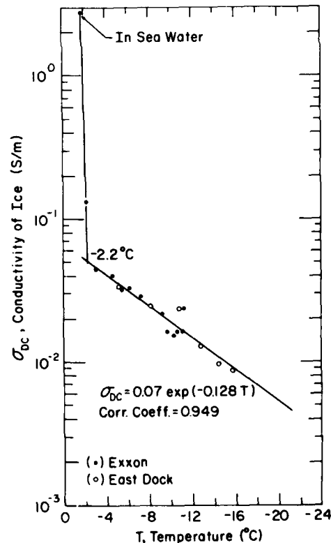
Figure 27. Measured DC conductivity of sea ice as a function of temperature.
