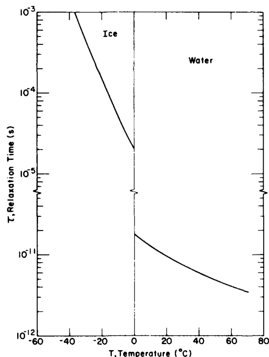
Figure 2. Relaxation time of pure ice and water as a function of temperature (after King and Smith 1981).
