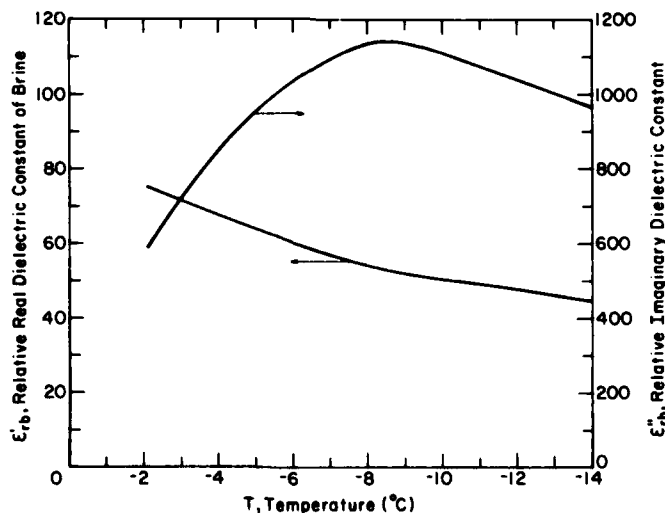
Figure 28. Calculated relative real and imaginary dielectric constants of brine at 100 MHz.
