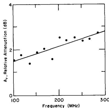
Figure 23. Example of relative attenuation as a function of frequency derived from time-domain transmission data.
