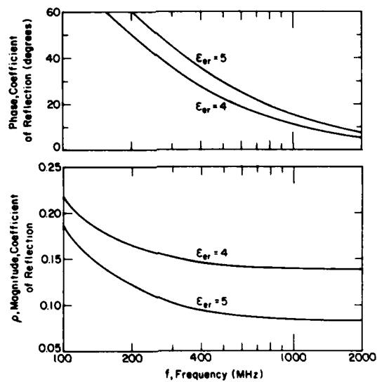
Figure 31. Magnitude and phase of the coefficient of reflection as a function of frequency for \epsilon_{er} = 4 and 5 and \sigma_e = 2.5 \times 10^{-2} \text{ S/m} .
