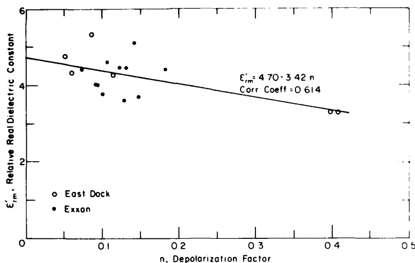
Figure 35. The calculated relative real dielectric constant of the sea ice-brine mixture as a function of the depolarization factor.
