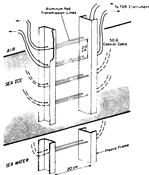
Figure 14. Schematic of ladder array of two-conductor transmission lines in sea ice.
