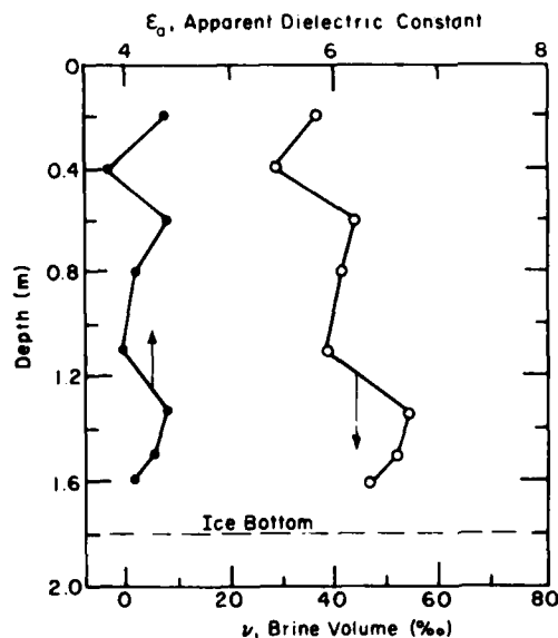
Figure 12. Apparent dielectric constant and brine volume as a function of depth at Spy Island site, 1979.
