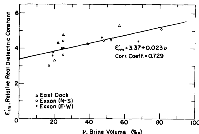
Figure 32. The relative real dielectric constant of sea ice-brine mixture as a function of brine volume. The solid line is a linear least-squares fit to all the data.
