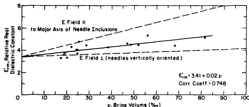
Figure 34. The calculated relative real dielectric constant of the sea ice-brine mixture as a function of brine volume. The calculation was made at 100 MHz using the depolarization factor (eq 32).
