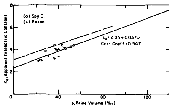
Figure 13. Apparent dielectric constant as a function of brine volume from the Exxon (1979) and Spy Island sites (1979).
