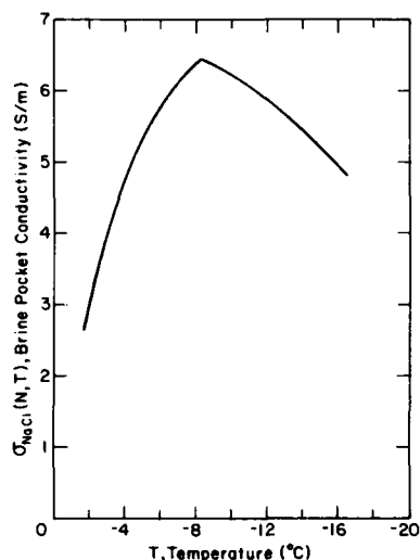
Figure 24. Brine pocket conductivity as a function of temperature.
