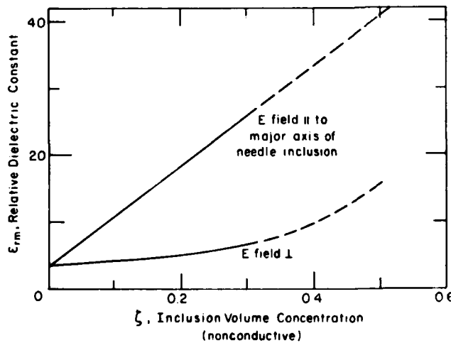
Figure 4. Relative real dielectric constant of sea ice-brine mixture as a function of inclusion volume concentration for the electric field parallel ( \parallel ) and perpendicular ( \perp ) to the major axis of the needle inclusions.
