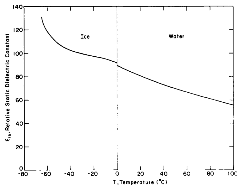
Figure 1. Relative static dielectric constant of ice and water as a function of temperature (after King and Smith 1981).
