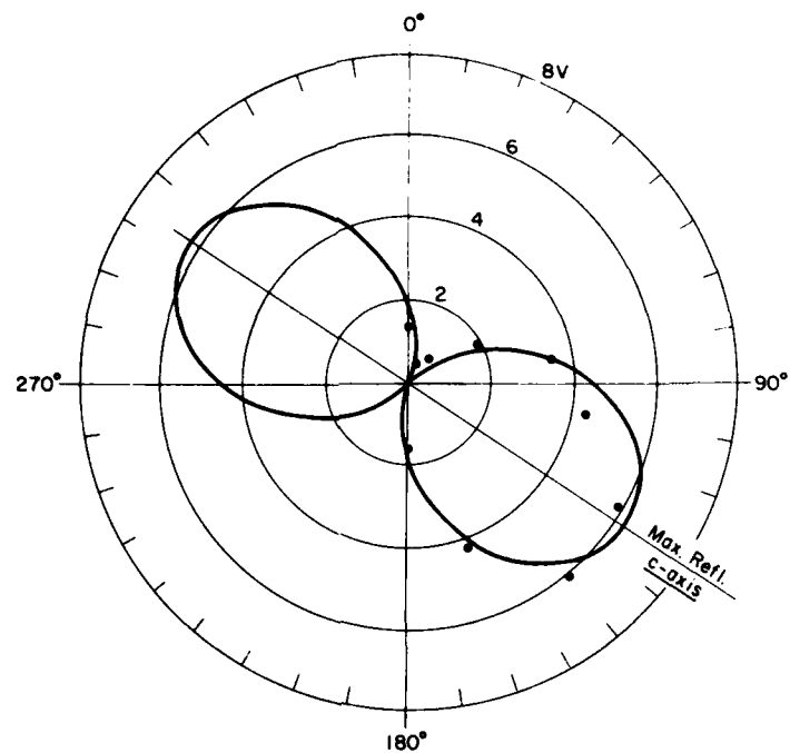
Figure 30. Voltage amplitude of the radar EM wavelet reflected from the ice antenna E-field azimuth at the Exxon site. The "lemniscate" curve fits the data with a correlation coefficient of 0.975. The major axis is at 122^\circ .
