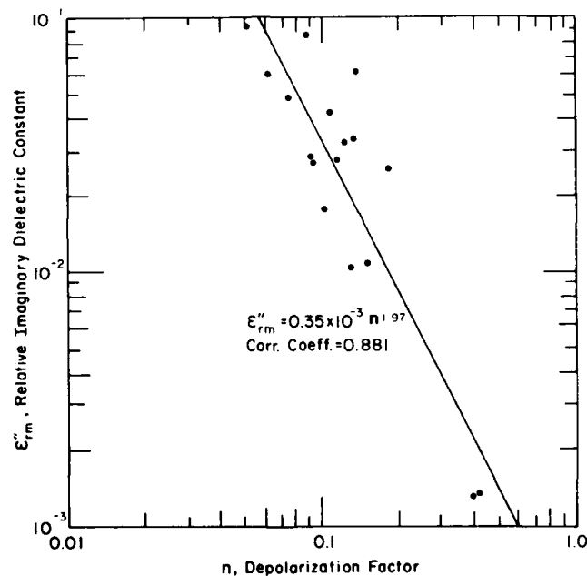
Figure 36. The calculated relative imaginary dielectric constant of the sea ice-brine mixture as a function of the depolarization factor.
