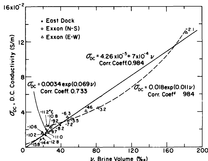
Figure 25. DC conductivity as a function of brine volume. Solid line is the linear least-squares fit. Dashed lines are exponential fits to the data above and below about the 80-cm depth.
