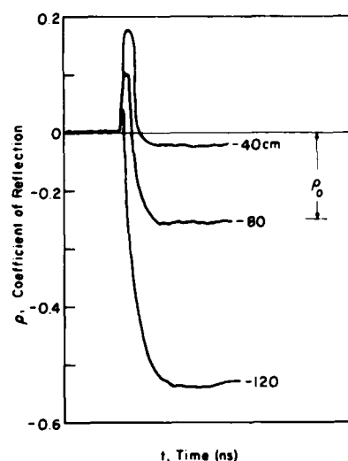
Figure 17. Examples of the coefficient of reflection as a function of time at three depths in sea ice at the East Dock site. \rho_0 is the low-frequency value of \rho .
