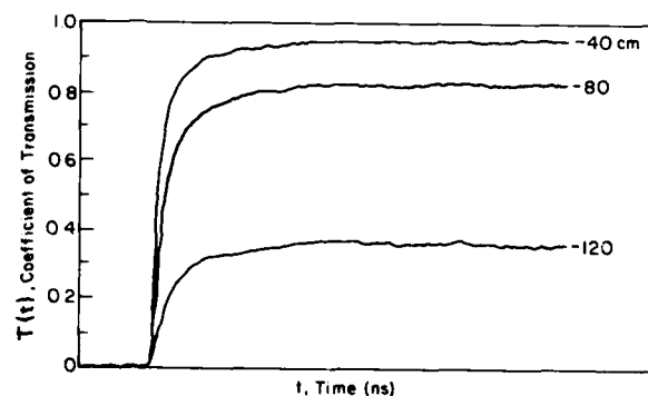
Figure 18. Examples of the coefficient of transmission as a function of time at three depths in sea ice at the East Dock site.
