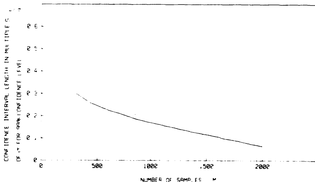
FIG C.1 DEPENDENCE OF CONFIDENCE INTERVAL LENGTH ON NUMBER OF SAMPLES FOR 99% CONFIDENCE LEVEL
