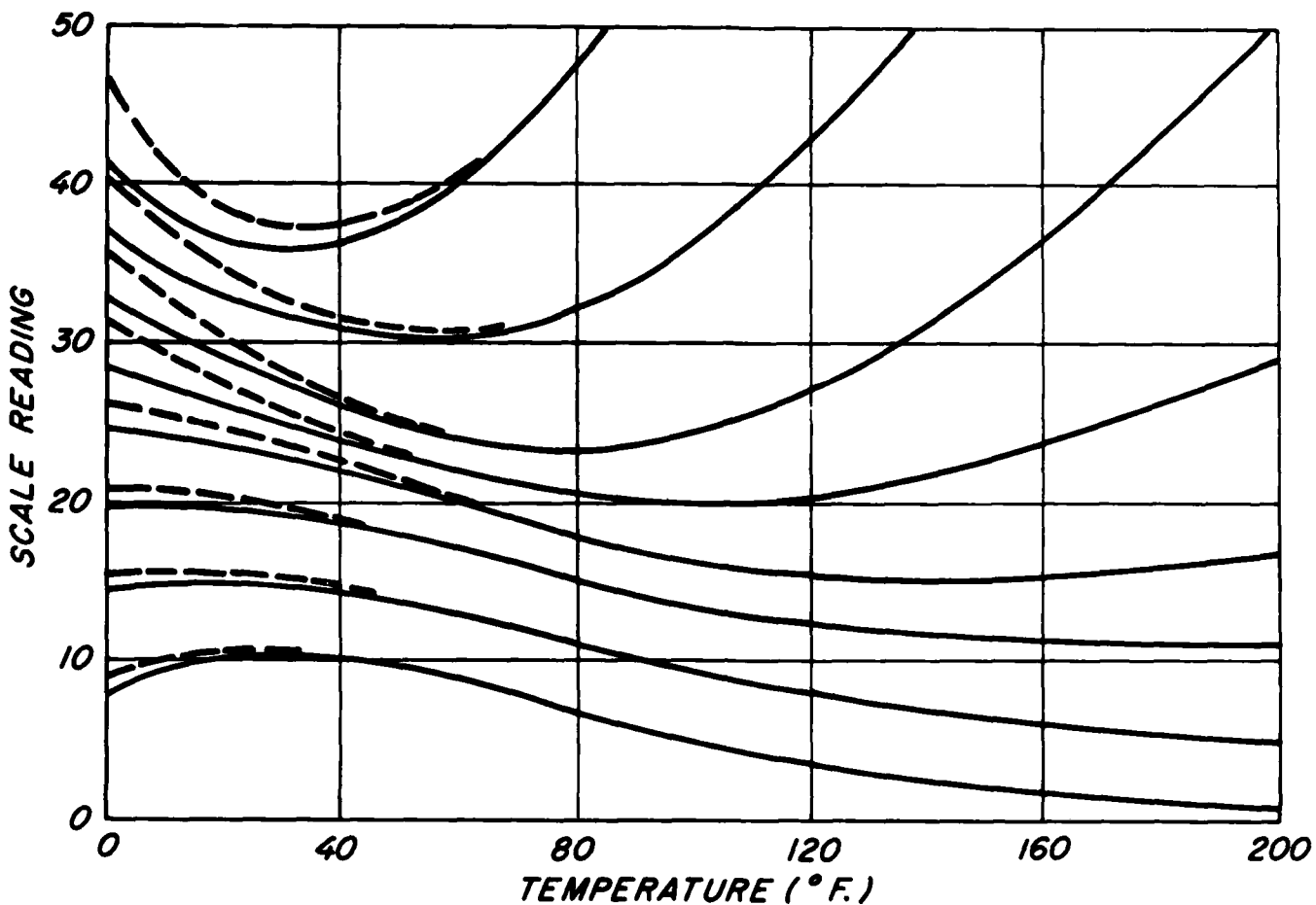
Figure 6.--Approximate temperature corrections for readings of power-loss type moisture meters; data taken using a Moisture Register model L. Locate the point whose coordinates are the observed scale reading and the specimen temperature, and trace back parallel to the curves to the calibration temperature of the meter (usually 80° F). The vertical coordinate here is the corrected scale reading, which is then converted to moisture content using the usual species conversion tables. Solid lines are for the meter itself at room temperature; dotted lines are for the meter at the same temperature as the specimens.
