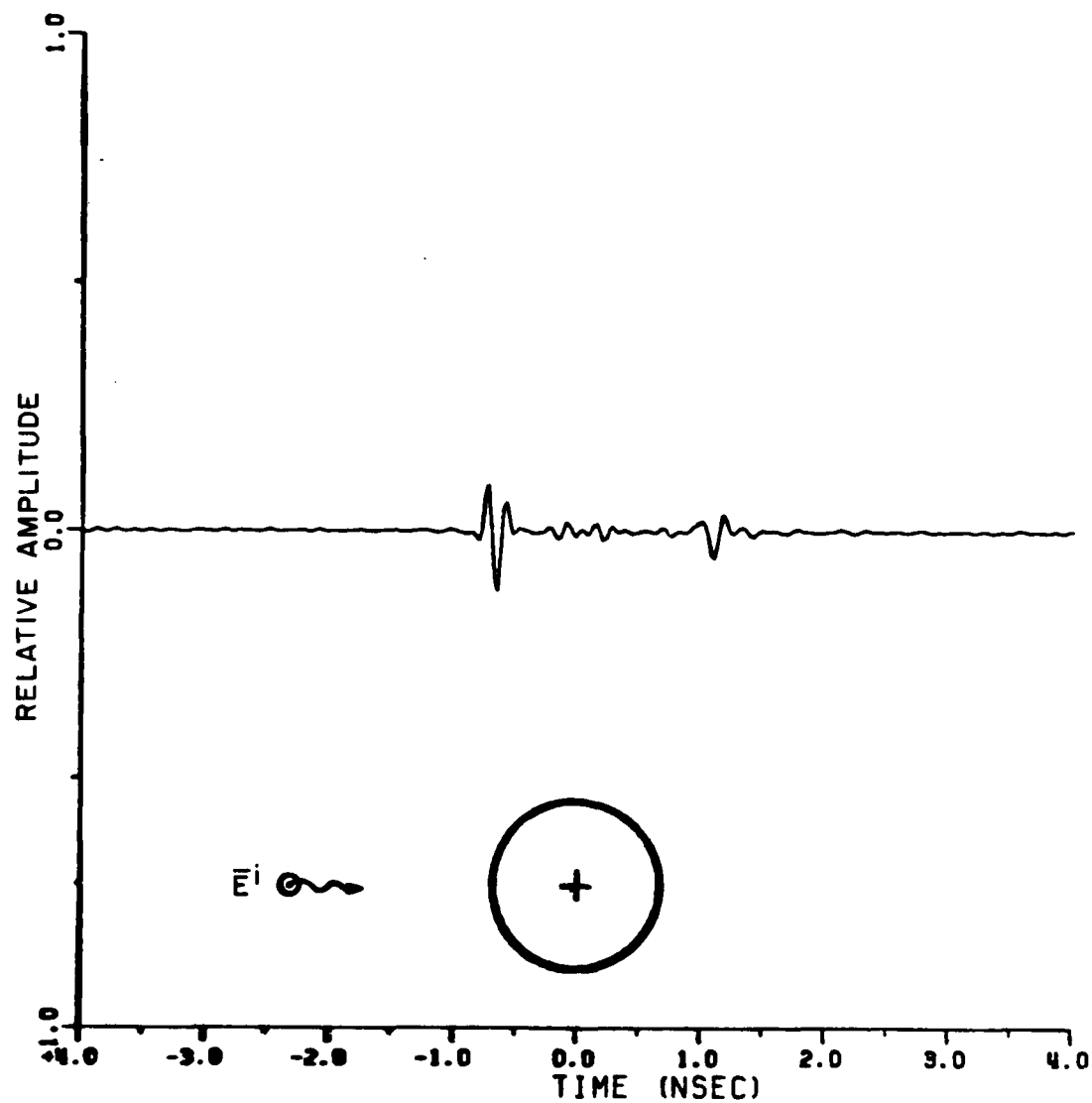
Figure F-8. Impulse response of a conducting disk, 90^\circ from normal incidence, polarization at 45^\circ to surface.
