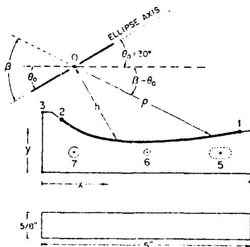
FIG. A1. Universal elliptical analyzer mounting block for four-inch crystal segments and for R_0 and h values in the ranges 10–100 and 1–4 in., respectively. The parameters that specify the curved profile that is machined into this block, for a given h value, are presented in Table A3.
