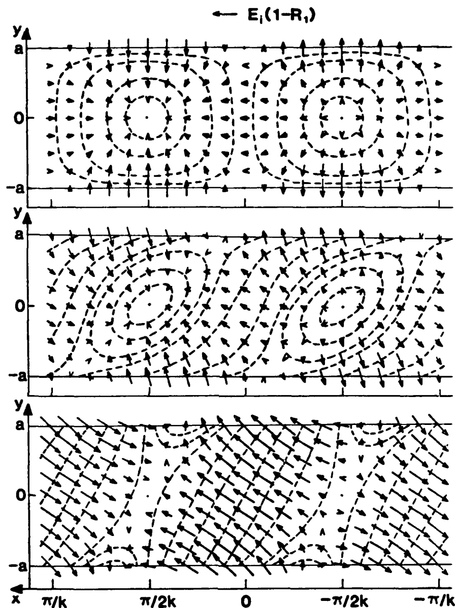
Figure 21: Three examples of the ionospheric electric field distribution (arrows) and direction of Hall current flow (dashed lines) in a high conductivity strip model of the auroral ionosphere. The incident wave is a plane polarized Alfvén wave travelling in the positive x -direction with its electric field polarized in the x -direction. The three panels are for different ratios of integrated Hall to Pedersen conductivity. The single arrow at the top of the figure shows the strength and direction the electric field would have in the case of uniform ionospheric conductivity.
