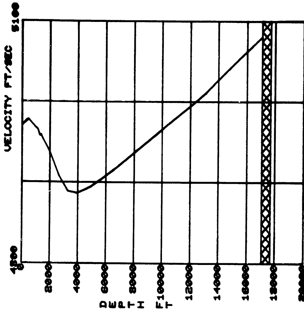
Figure 7-2. F-FACT Sound Speed Profile
