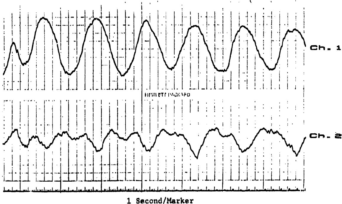
Figure 9. Respiration detected from 30 meters for subject positioned with head toward antenna.
