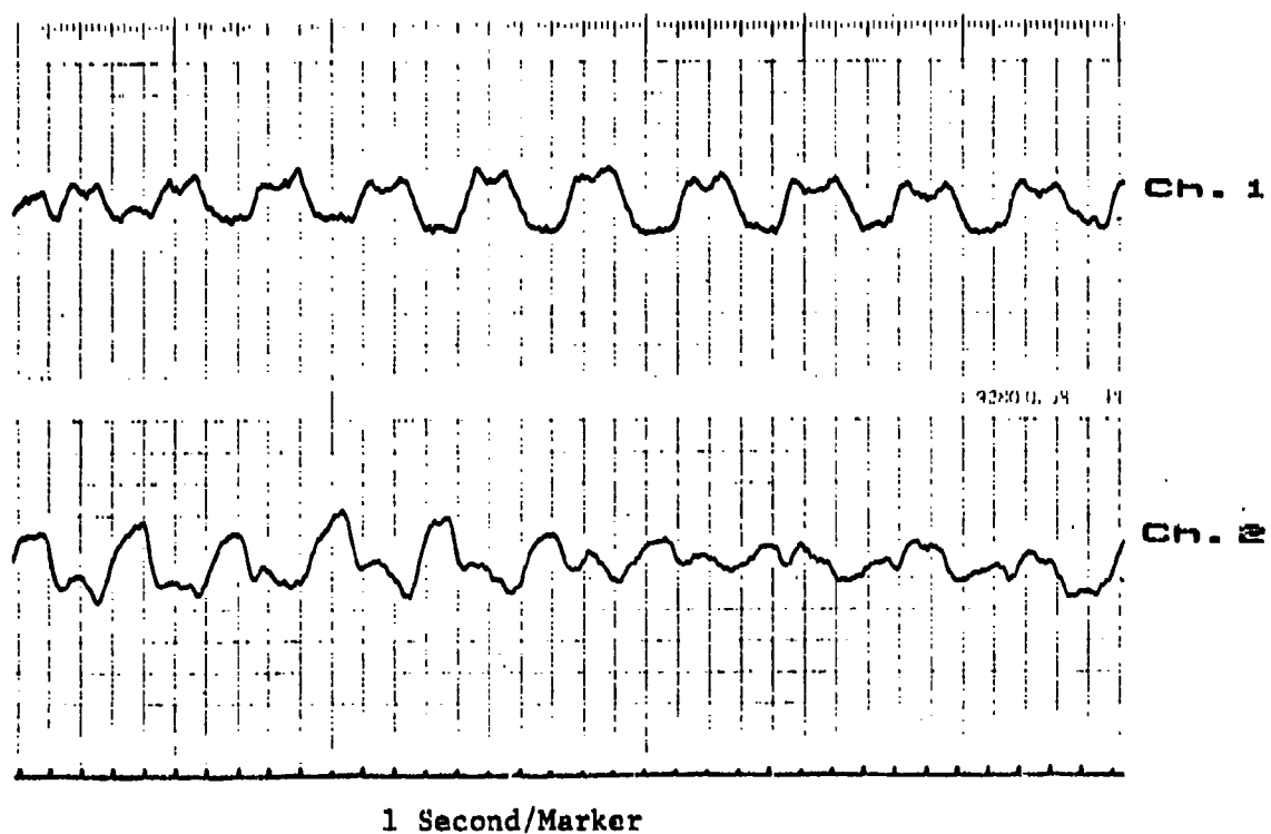
Figure 14. Respiration detected from 40 meters. Respiration signal present on both Ch. 1 and Ch. 2.
