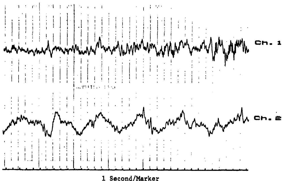
Figure 20. Respiration detected from 50 meters using 1 Hz high-pass filters. Respiration signal present on Ch. 2.
