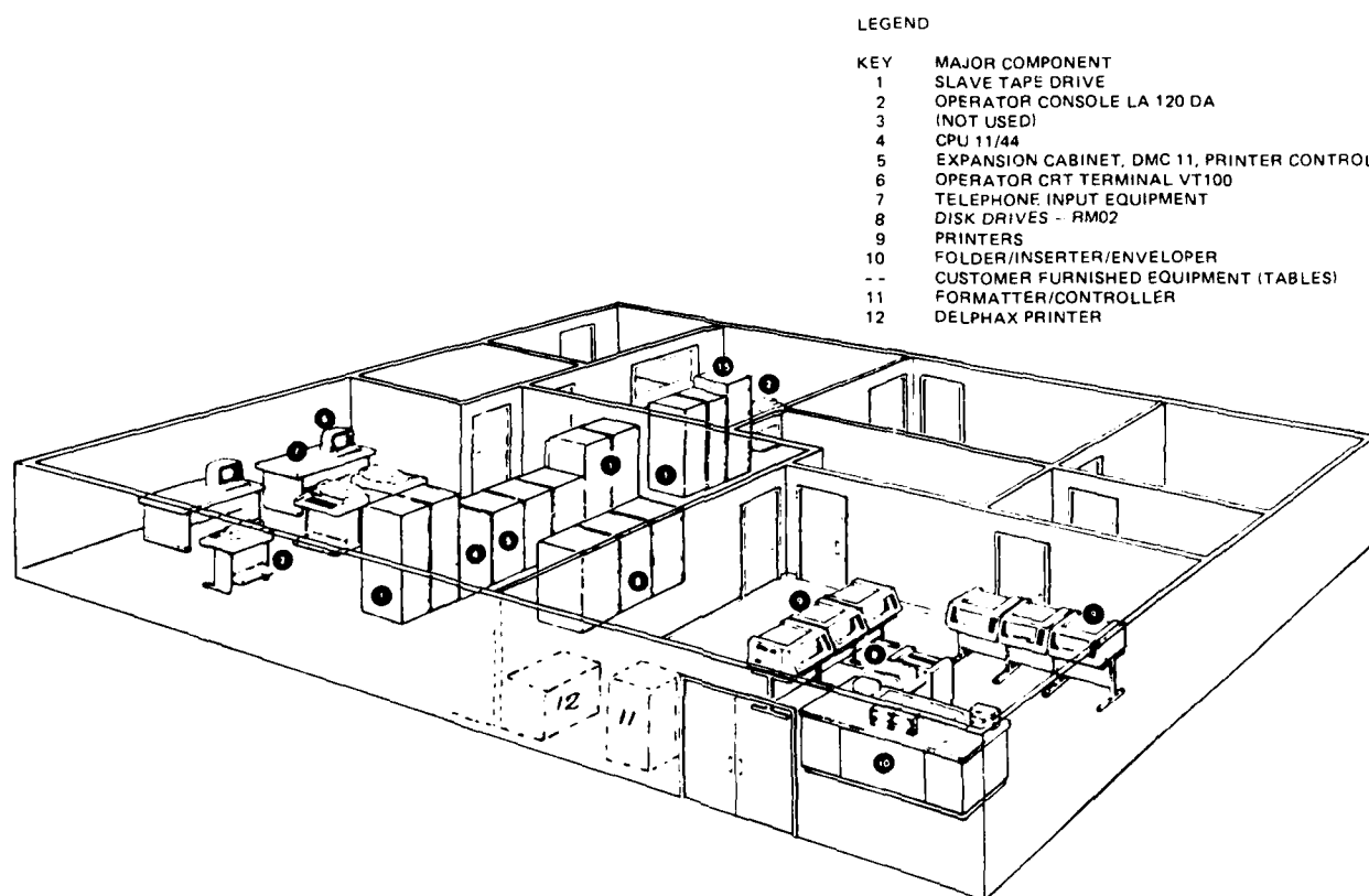
Figure B15. Delphax printer installation within an existing E-COM site.
