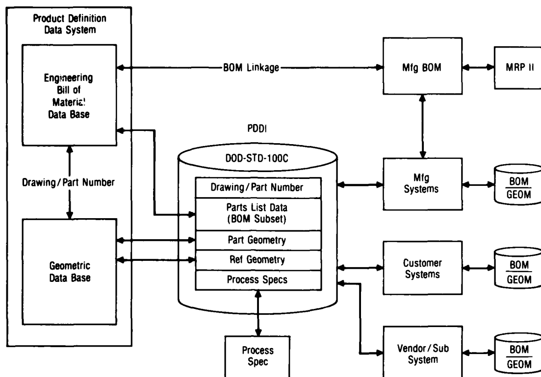
Figure 25. - PDDI - replaces the function of the engineering drawing.
