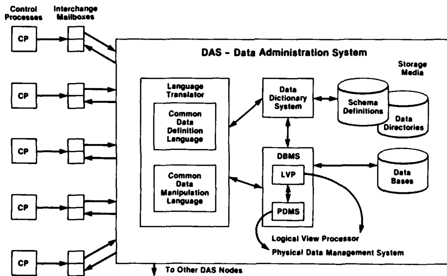
Figure 2.- Data administration system.
