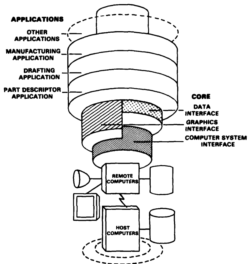
Figure 1.- System organization.
