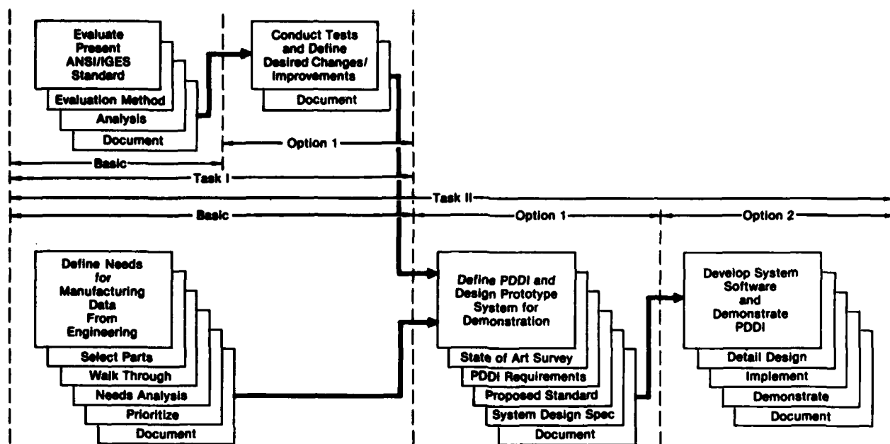
Figure 3. - Program summary.
