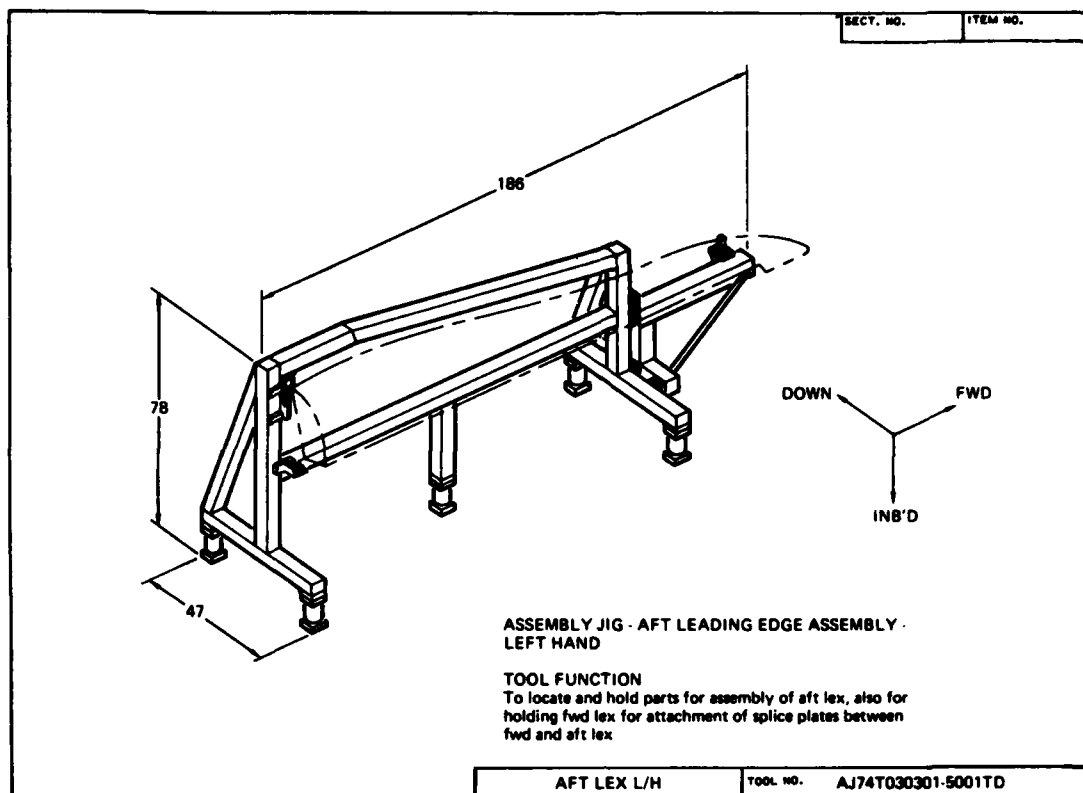
Figure 15. - Assembly jig tooling drawing.
