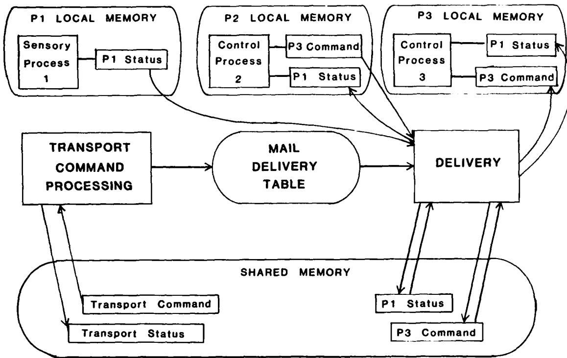
Figure 5.- Local mail transport process.
