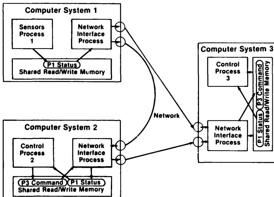
Figure 4.- Distributed memory mapped database.
