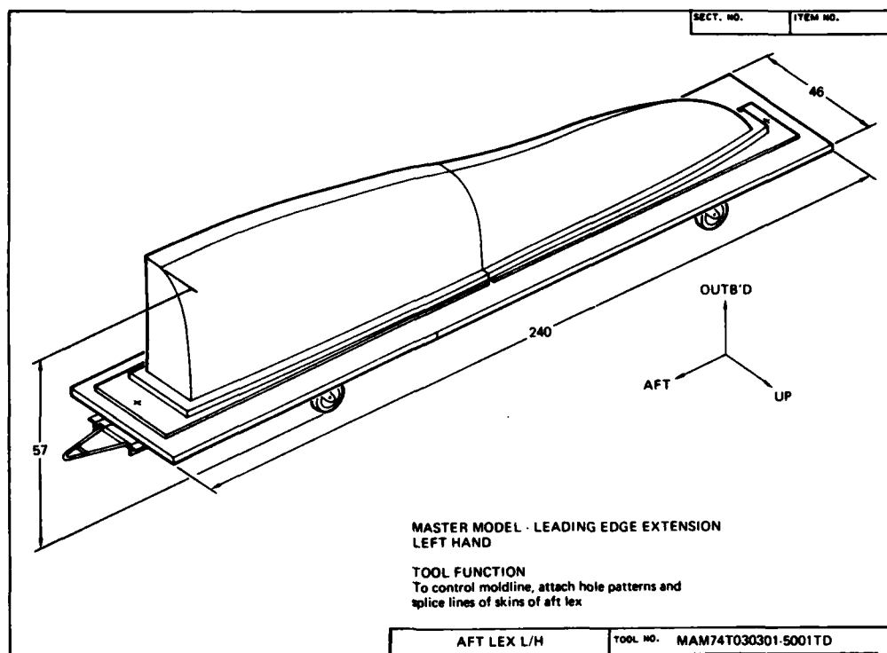
Figure 13. - Master model tooling drawing.
