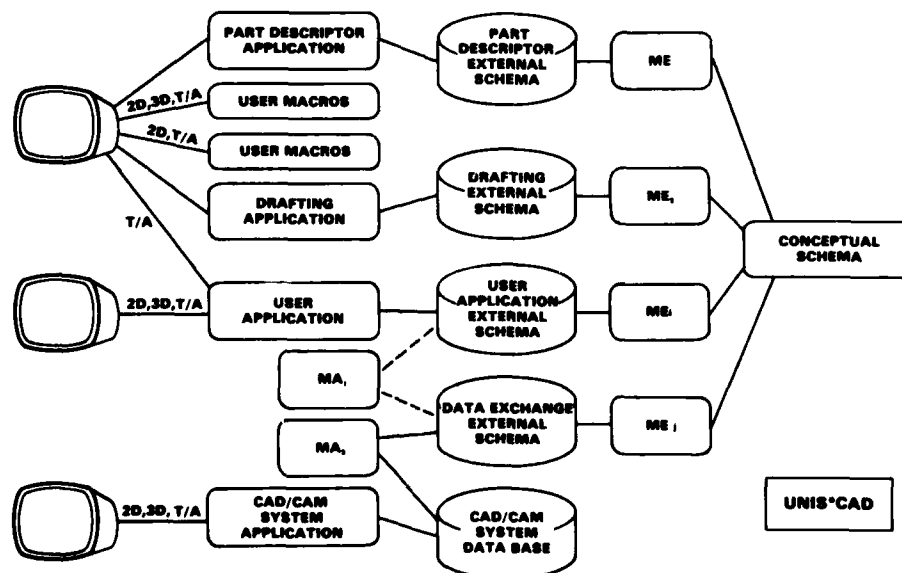
Figure 8.- User interfaces.
