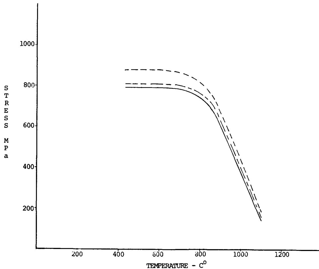
Figure 2.- Output display.
