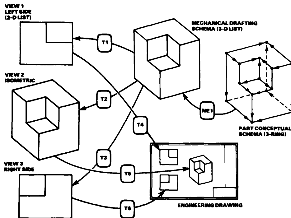
Figure 7.- Drafting view projections.
