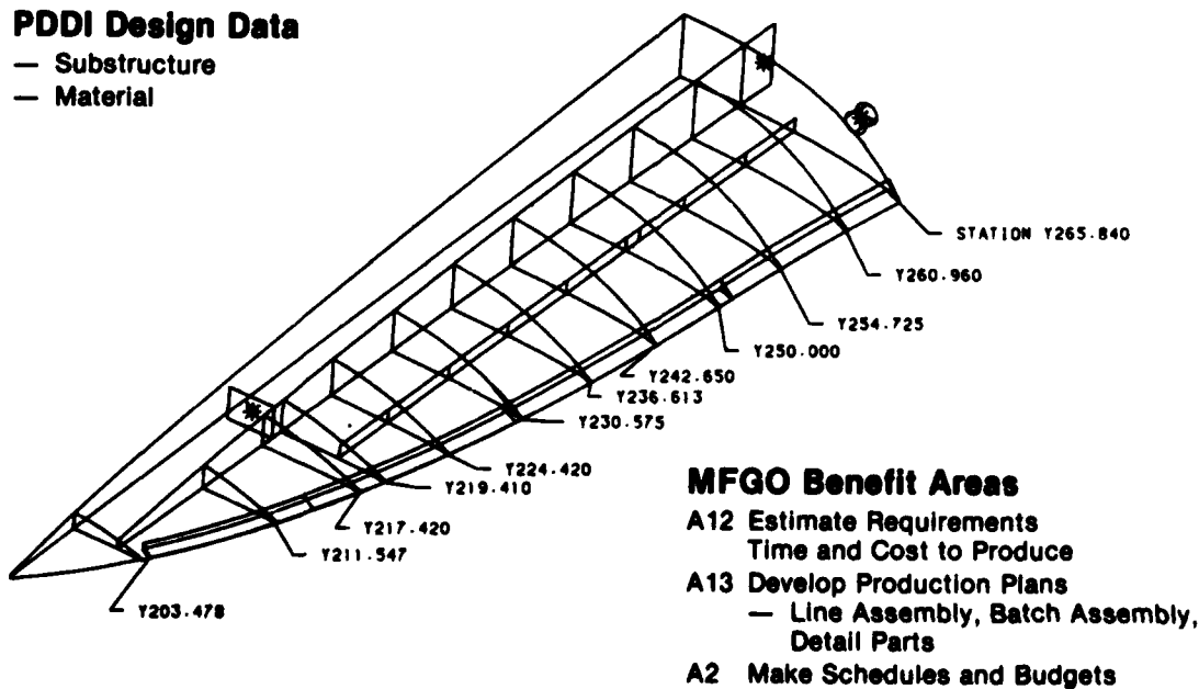
Figure 16. - Conceptual analysis - substructure definition.
