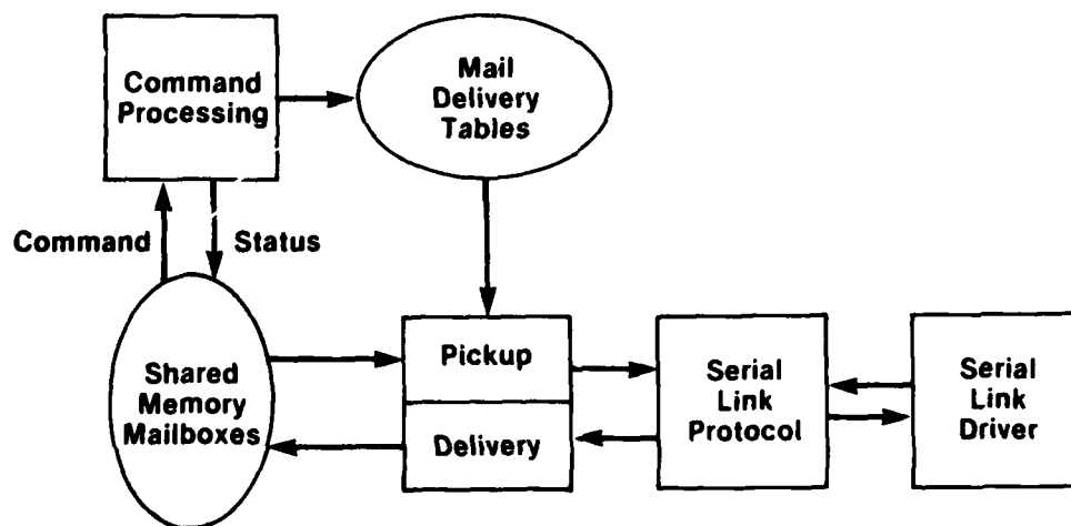
Figure 6.- Network interface process.
