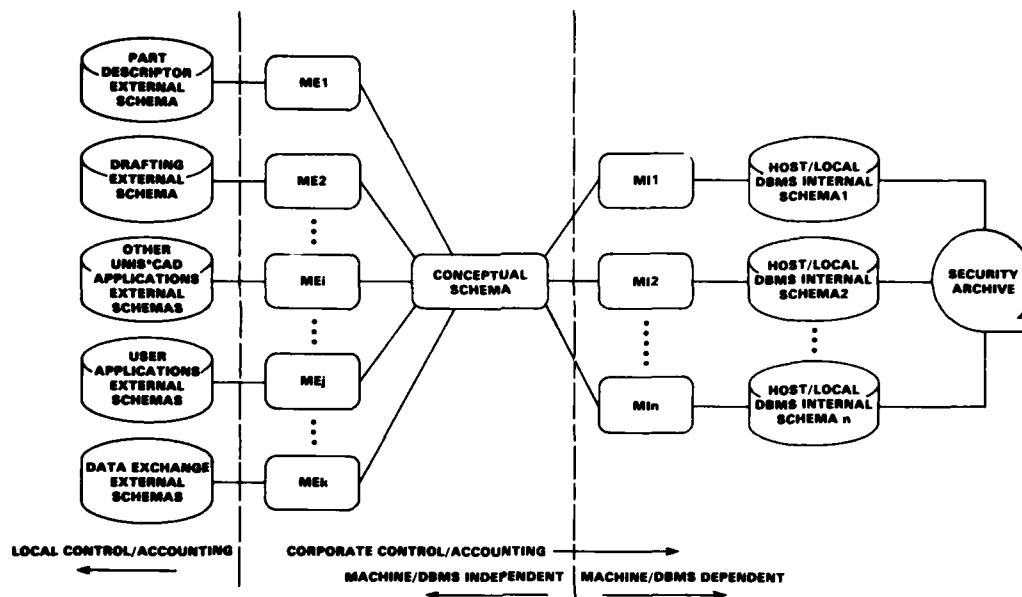
Figure 3.- Multi-schema structure for Hybrid System.
