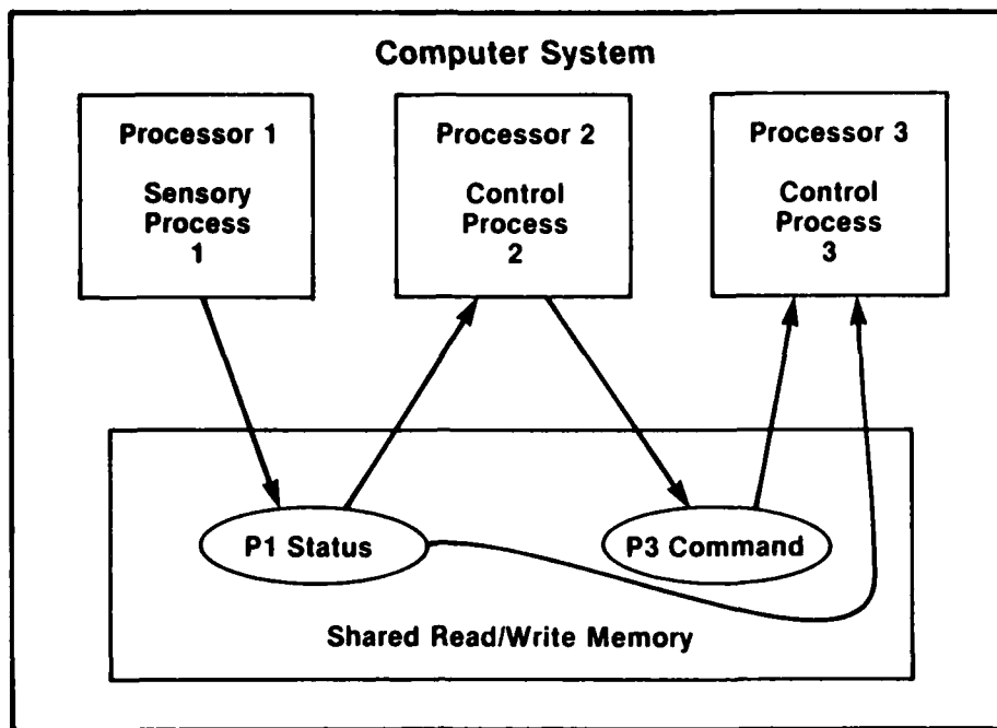
Figure 3.- Memory mapped database.
