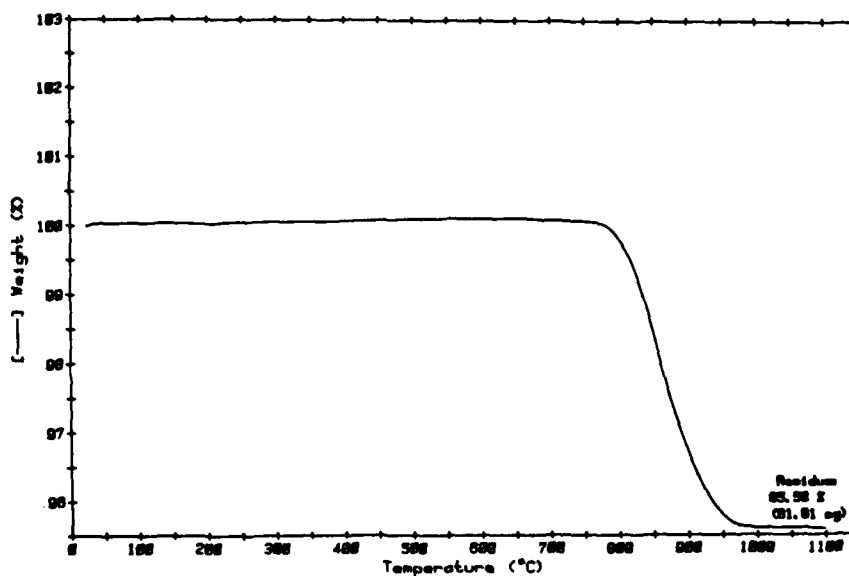
FIGURE 3. TG CURVE OF MUSCOVITE MICA, 84.77 MG, 20° C/MIN, 50 CC/MIN Ar
