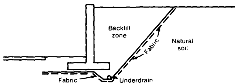
c Potential cross-sections of geotextiles placed behind a retaining wall
