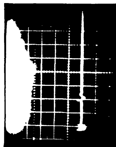
Figure 108. Transient record of discharge 11:47 on 0.020 cm second surface mirrors exposed to 16 kV electrons. We believe this is a punch-through or flash-over to the substrate, with no blow-off.
