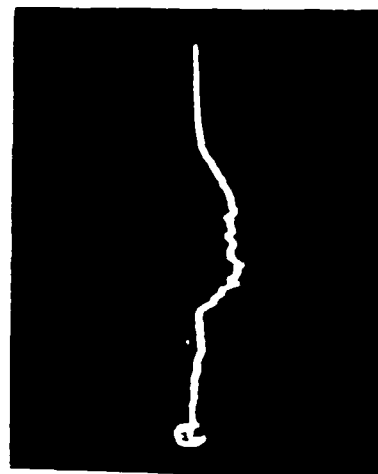
Figure 26. Transient record of discharge 4:55 on 0.005 cm Kapton exposed to 75 nA/cm 2 of 26 kV electrons.
