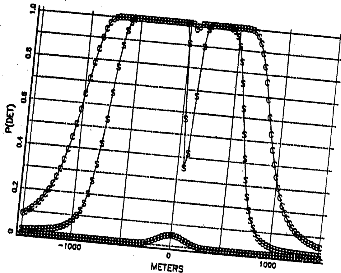
Figure 4.10. Lateral Range Curves for a Vertical Separation of 500 Meters.
