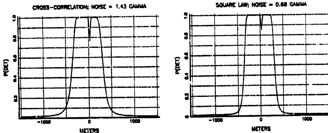
Figure 4.2. Cross-Correlation and Square Law Lateral Range Curves to Describe the Performance of an Operator with an ORF of 3.
