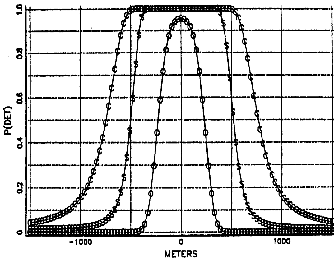
Figure 4.9. Lateral Range Curves for the Submarine Headed East and the Aircraft Headed North.
