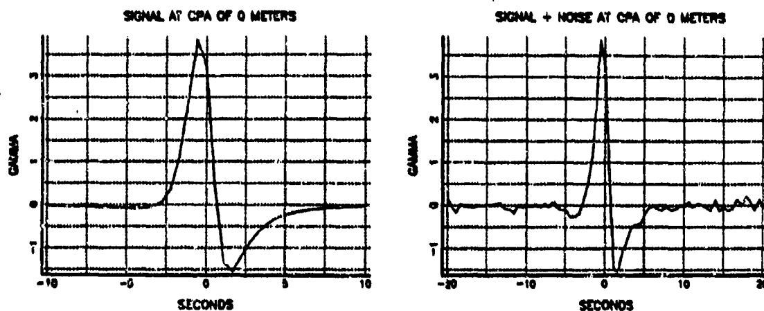
Figure 4.4. Magnetic Signal and Magnetic Signal Plus Magnetic Noise at a Lateral Range at CPA of 0 Meters for the Base Case.
