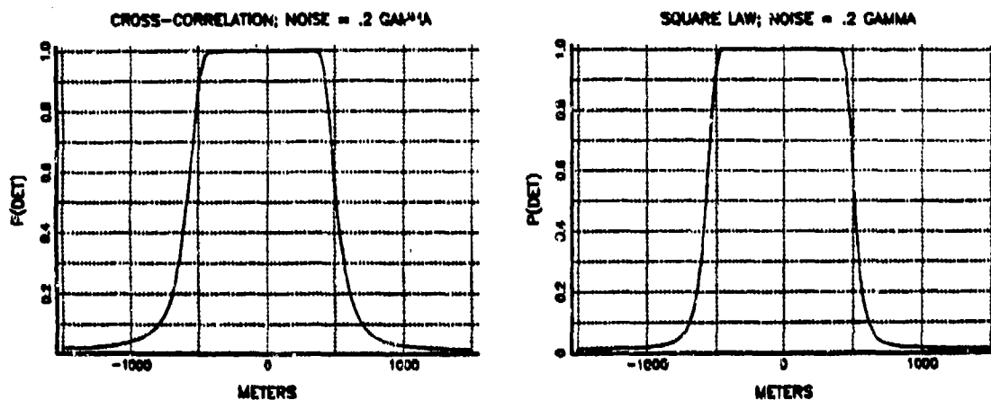
Figure 4.3. The Cross-Correlation and Square Law Models to Describe LRC's for the CAE Automatic Detection System.
